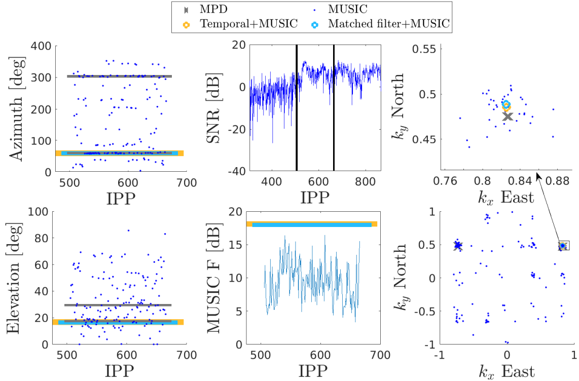
Figure 2. Meteor recorded at 2018-12-13 00:03:27.302 UTC. The upper right-middle panel illustrates SNR versus IPP and the two vertical black lines denotes when the meteor occurred. This event had three range ambiguities: 187.9 km, 257.9 km and 327.9 km, and two angular ambiguities. The peak SNR was 8.7 dB. The two angular ambiguities are marked by red-grey horizontal lines in the upper left panel (azimuth) and the lower left panel (elevation). The MUSIC DOA output from event-individual IPPs are illustrated as blue dots and-while the green-light blue and orange transparent line-denotes-lines denote the DOA output after temporal integration with and without matched filter optimization, respectively . The same information is given in wave vector ground projected space, k_x, k_y in the lower-right-panel . Here, the MPD-file ambiguities are marked by red crosses and the temporally integrated MUSIC by a green circle two rightmost panels . Finally, the distribution of MUSIC responses F as a function of IPP is illustrated in the lower middle panel. Here, the green-line-denotes-horizontal lines denote the MUSIC response for the temporally integrated spatial correlation matrix/matrices .
