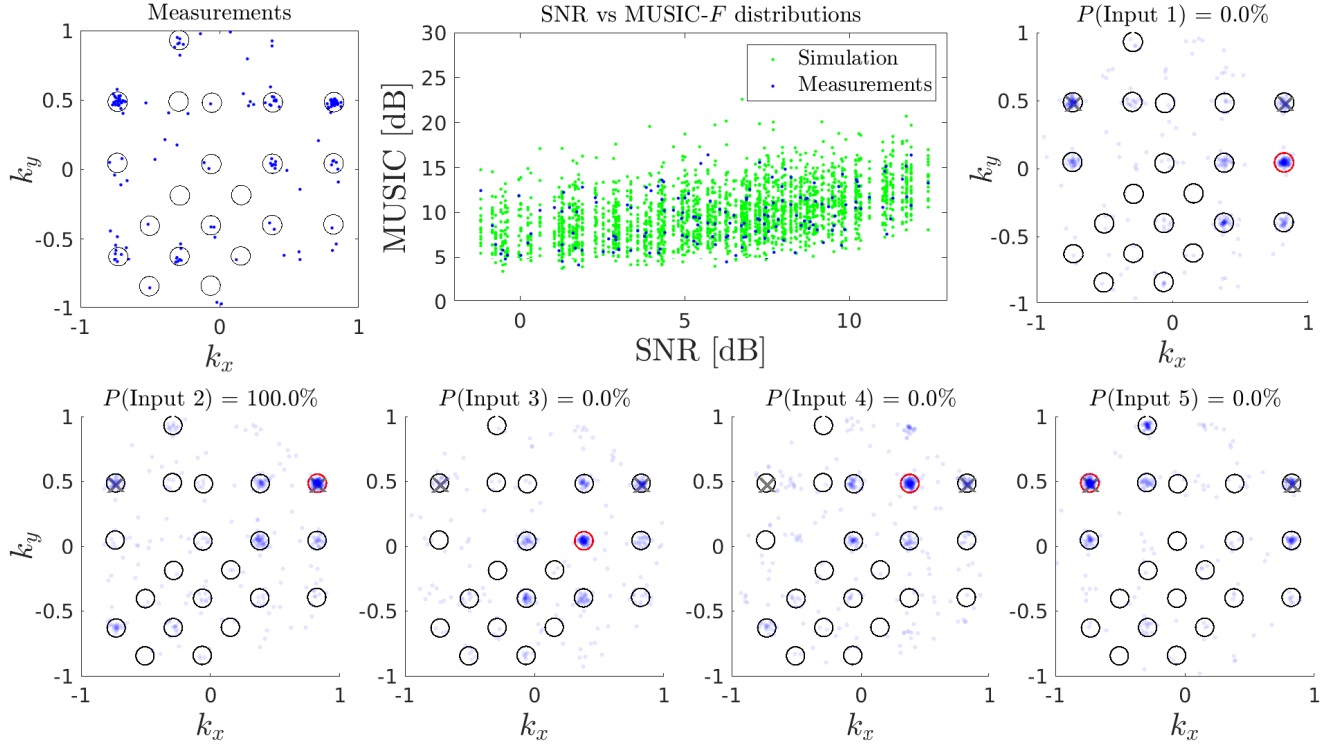
Figure 3. Summary of the DOA determination simulations and the Bayesian inference results for the meteor in Fig. 2. Four Five different possible true DOAs were identified and their individual MC simulations are illustrated in the panels titled Input 1-4 1-5 . The Bayesian probability of an input DOA being the true location of the trail is given in the title. In each of these panels, the input DOA is marked by a large red circle and the MPD-file results are marked by red grey crosses. The measured DOA output distribution is given in the upper left panel. The black circles denote the possible ambiguities and their inclusion regions. The small red circle denotes the MUSIC output after temporal integration and matched filter results illustrated in Fig. 2 coincide with the largest probability location here . The upper middle panel shows the measured and simulated distributions of MUSIC response F versus SNR.
