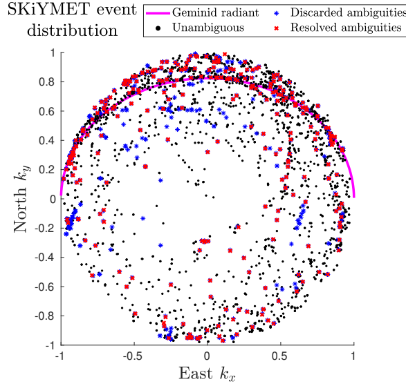
Figure 4. Illustration of the event DOA distribution improvement in 10 minutes of 2,222 events in Sodankylä SKiYMET meteor radar data before and after applying temporal integration. The black dots are the unambiguous meteor trail events, the green-dots-blue stars are the original ambiguous locations that could be discarded, and the red crosses are the resolved ambiguities after temporal integration. There are multiple green-dots-blue stars per event and red cross. The data was recorded during the Geminid meteor shower. The blue-solid line illustrates directions that fulfill the specular condition for meteors arriving from the Geminid radiant.
