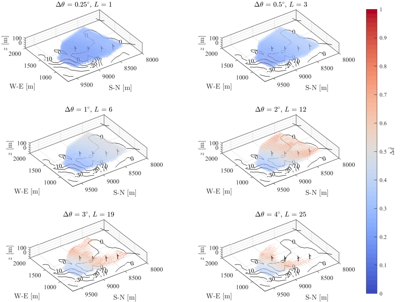
Figure 6. Random data spacing, \tilde{\Delta d} , for 6 volumetric scans with different angular resolution and \sigma = 1/4 . Points violating the Petersen-Middleton constraint ( \tilde{\Delta d} > 1 ) are not displayed.
