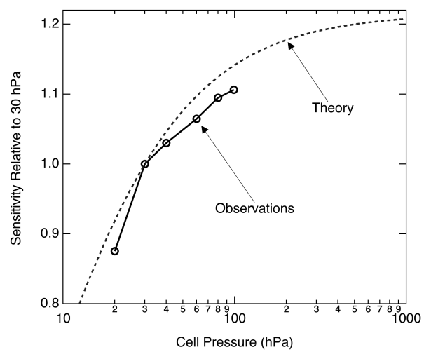
Figure 6. Calculated and measured dependence of the LIF signal sensitivity on sample cell pressure.
