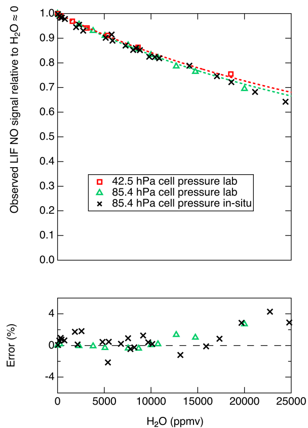
Figure 7. Top panel: Markers show the observed S/S_0 values, and dashed lines show the calculated \frac{S}{S_0} values using k_{H_2O} = 6.9 \times 10^{-10} \text{ cm}^3 \text{ molecules}^{-1} \text{ s}^{-1} . Bottom panel: Relative difference between observed and calculated S/S_0 values shown in the top panel.
