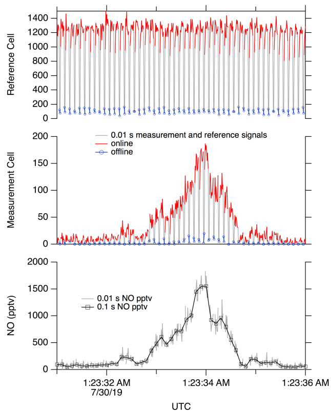
Figure 9. A five second segment of typical data. Bottom The top panel shows observed online signal in the reference cell, and offline the middle panel shows the signal rates in the measurement cell. Top The bottom panel shows the calculated NO at 10 Hz.
