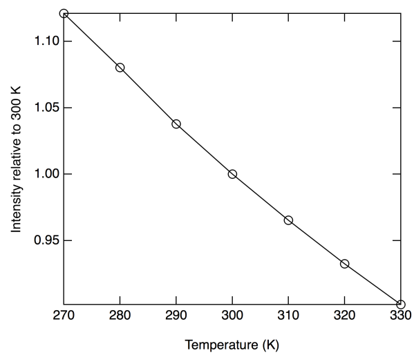
Figure 5. Calculated temperature dependance dependence of the absorption cross section near 300K.
