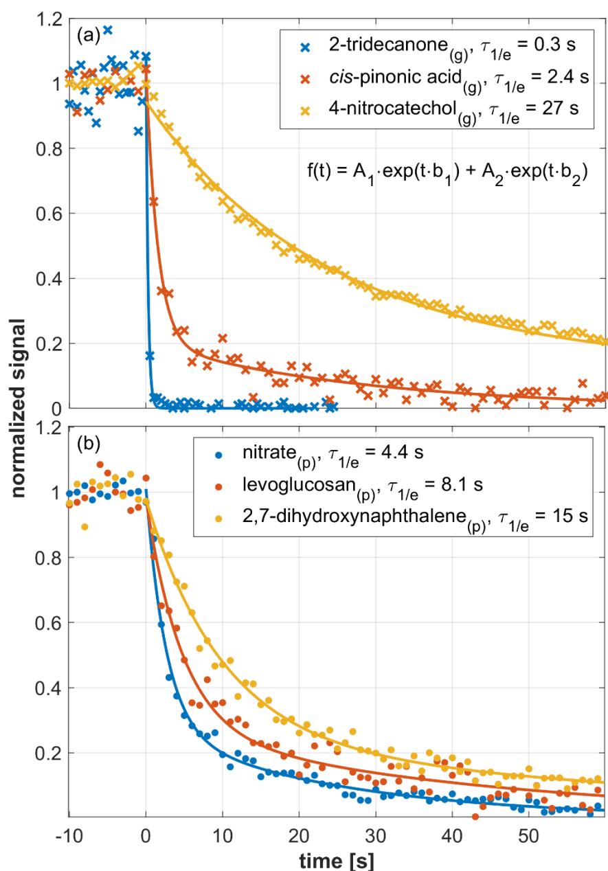
Figure 3. Signal decay as observed in an EVR PTR-MS analyzer ( T_{\text{drift}} = 120^\circ\text{C} ) after a steady supply of analyte was instantly switched off at t = 0 s. The decay of gaseous analytes is shown in the upper panel, while the lower panel refers to particulate analytes. Initial steady-state mixing ratios were as follows: 2-tridecanone (g) : 1 ppbv, cis -pinonic acid (g) : 2.2 ppbv, 4-nitrocatechol (g) : 30 ppbv, nitrate: 3 ppbv; levoglucosan (p) : 1.2 ppbv, 2,7-dihydroxynaphthalene (p) : 0.3 ppbv. Signals were fitted using a double exponential decay function (see insert in the upper panel). All fitting parameters are listed in Table S2.
