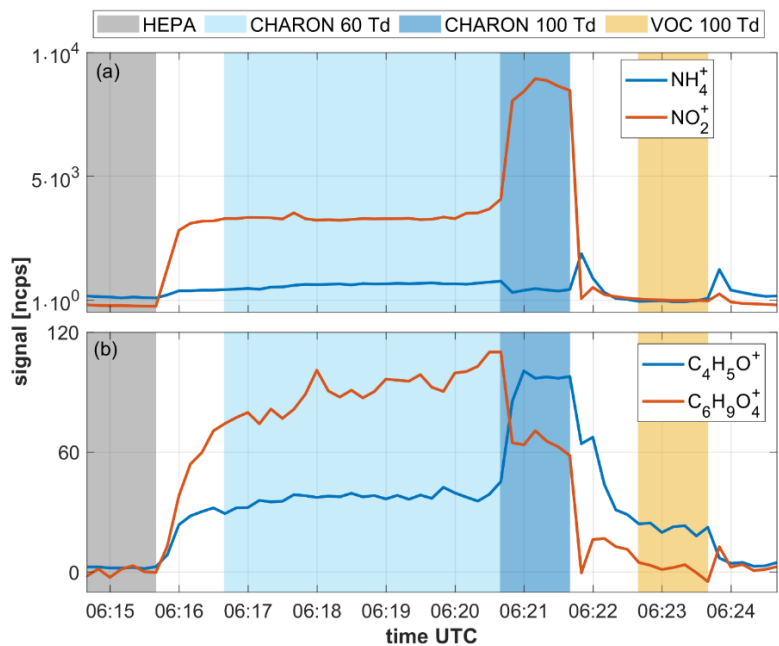
Figure 7. Time series showing various analyte signals as recorded during a 10-minute measurement cycle of ambient air. The 10-min measurement cycle included: i) 1 min of instrumental background measurements with the CHARON inlet including a HEPA filter, ii) 4 mins of particulate measurements at an E/N of 60 Td, iii) 1 min of particulate measurements at an E/N of 100 Td and iv) 1 min of gas measurements at an E/N of 100 Td. The benefit of measuring particles at 60 and 100 Td is explained in Leglise et al. (2019) and is not discussed here. The CHARON inlet enriched the particle concentration by a factor of ~20, which explains the higher signal intensities in the particle measurement (in blue) as compared to the gas measurement (in yellow).
