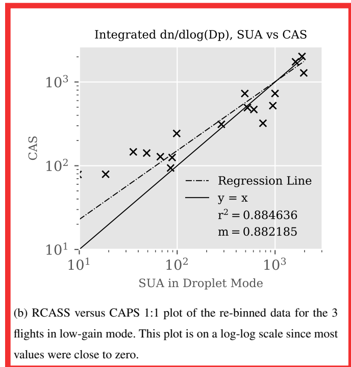
Figure 10. 1:1 plots for the re-binned dN/d\log(D_p) . The solid line represents perfect agreement; the dotted line is the regression line using RMAR. r^2 is the coefficient of determination and m is the gradient of the regression line.
