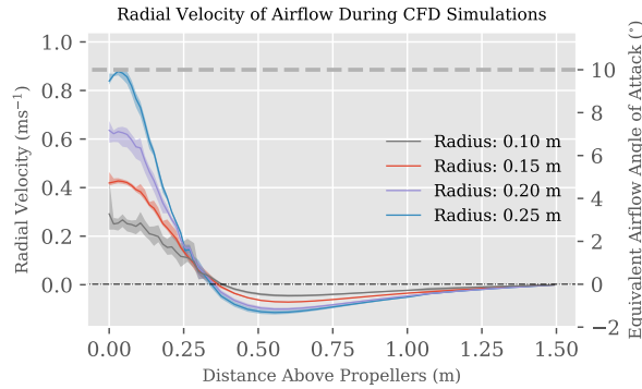
Figure 8. CFD results for the (circumferential averaged) radial velocity of the airflow as a function of distance above the propellers. The shaded regions around the lines show the variation of the air velocity around the circumference of the domain, while the bold lines show the mean. The dashed line represents the angle of attack limit specified in Smith et al. (2019).
