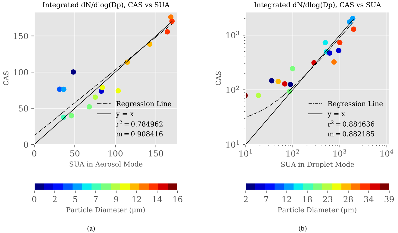
Figure 11. 1:1 plots for the re-binned dN/d\log(D_p) . The solid line represents perfect agreement; the dotted line is the regression line using RMAR. r^2 is the coefficient of determination and m is the gradient of the regression line. In Fig. 11b, a log-log scale was used since most values were close to zero; the appearance of a curved regression line in Fig. 11b is simply due to the log-log scale. The colour of the points corresponds to the bin geometric mean diameter, which is shown on the colour-bar beneath the graph.
