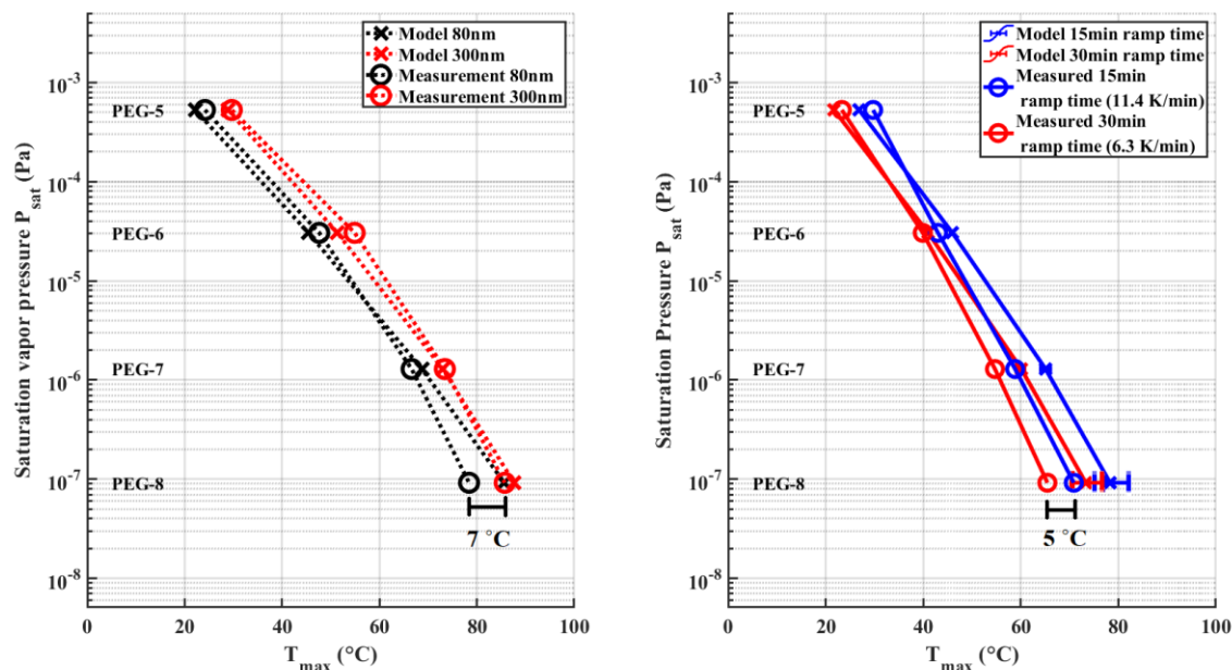
Figure 7. a) T_{\text{max}} values measured for 80 nm and 300 nm particles with ramp time of 15 min. The difference in T_{\text{max}} between the two particles sizes is \sim 7 °C. Panel b) shows measured T_{\text{max}} values of 15 min and 30 min ramping times using polydisperse aerosol particles. The difference between the two heating rates is \sim 5 °C. Error bars are omitted from the measured values in the figure for sake of clarity. In the panel b) whiskers show the range of model results when using uncertainties of evaporation enthalpy shown in Krieger et al., (2018). The standard deviations of the for all measured points is panel a) is between 0.2-0.5 °C. In panel b) the standard deviations for measured points are between 0.2 – 1.3 °C.
