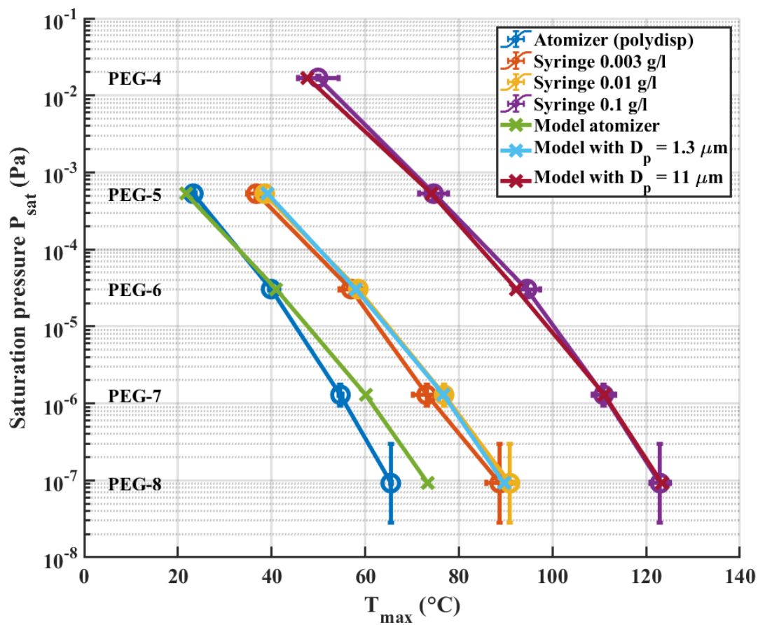
Figure 4. Comparison of the solution concentration effect on PEG results with model results. Error bars in T_{\text{max}} values are standard deviations of three repetitions.
