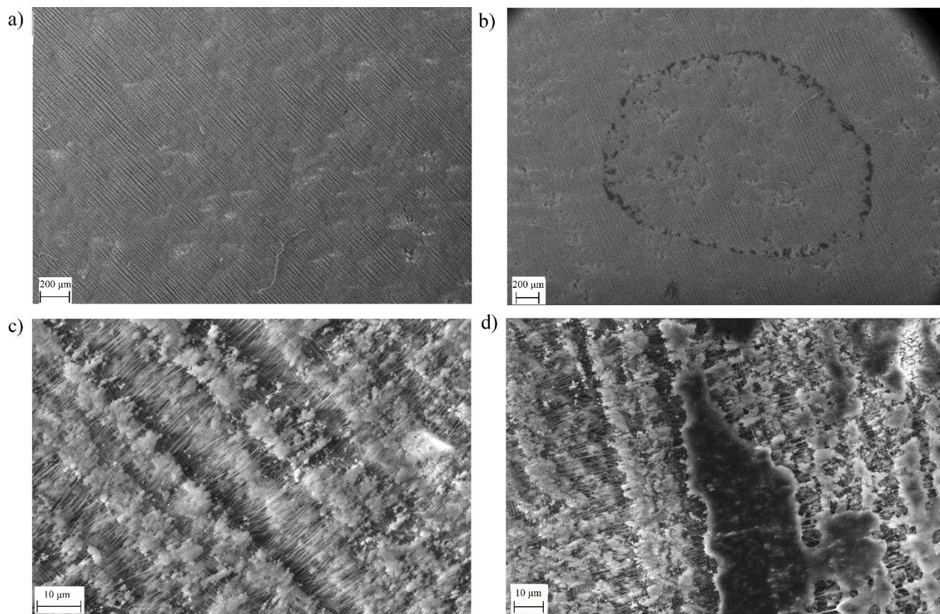
Figure 5. SEM pictures. Panel a) 10 \mu\text{l} of pure ACN deposited on the filter. Panel b) 3 \mu\text{l} of PEG-8 with concentration of 0.01 \text{ g L}^{-1} (30 ng) in ACN deposited on the filter. Panel c) magnification shows magnification panel a) and panel d) shows magnification of the PEG-8 residue.
