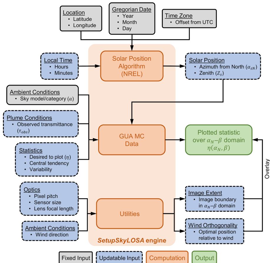
Figure 6. Flow chart of the main procedure of the SetupSkyLOSA software tool. The user provides the location, Gregorian date, time zone, and local time, which are used to compute the corresponding solar position using the Solar Position Algorithm of the National Renewable Energy Laboratory (NREL; Reda and Andreas, 2008). Then, with data on ambient conditions and observed plume transmittance, the software tool plots the desired statistic of soot mass column density over the \alpha_N - \beta domain. Additional utilities include the overlay of the image sensor and optimal positioning relative to the wind on the plotted statistic, in addition to the “maximizer” and “positioner” utilities, which are not shown in the figure. The latter two utilities permit a user to identify acceptable camera positions and pointings over a measurement period and output these data in .kml format for use with mapping software such as Google Earth.
