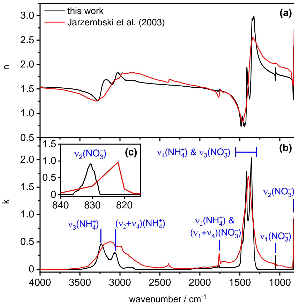
645 Figure 4: Real (a) and imaginary (b) parts of the complex refractive for solid AN at 223 K derived from this work (black lines) in comparison with room-temperature data from Jarzembki et al. (2003) (red lines). The insert (c) shows an expanded view of the k spectrum in the regime of the \nu_2(\text{NO}_3^-) mode.
