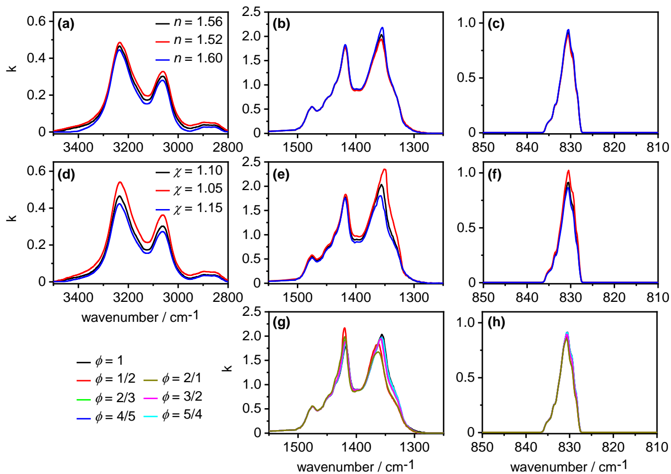
650 Figure 5: Sensitivity of the retrieved k(\tilde{\nu}) spectrum on the parameters n(\tilde{\nu}_x) , \chi , and \phi in different wavenumber regimes. (a) – (c) Variation of n(\tilde{\nu}_x) with \chi = 1.1 and \phi = 1 . (d) – (f) Variation of \chi with n(\tilde{\nu}_x) = 1.56 and \phi = 1 . (g) and (h) Variation of \phi with n(\tilde{\nu}_x) = 1.56 and \chi = 1.1 .
