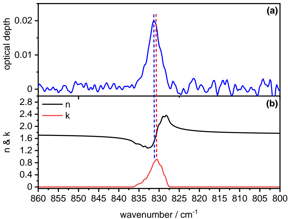
670 Figure B2: Comparison between the measured infrared extinction spectrum of crystalline AN particles (a) and the retrieved optical constants (b) in the 800 – 860 \text{cm}^{-1} wavenumber range. The retrieval was performed with the parameters n(\tilde{\nu}_s) = 1.56 , \chi = 1.1 , and \phi = 1 . Vertical dashed lines indicate the peak position in the particle extinction spectrum (blue) and the k(\tilde{\nu}) spectrum (red).
