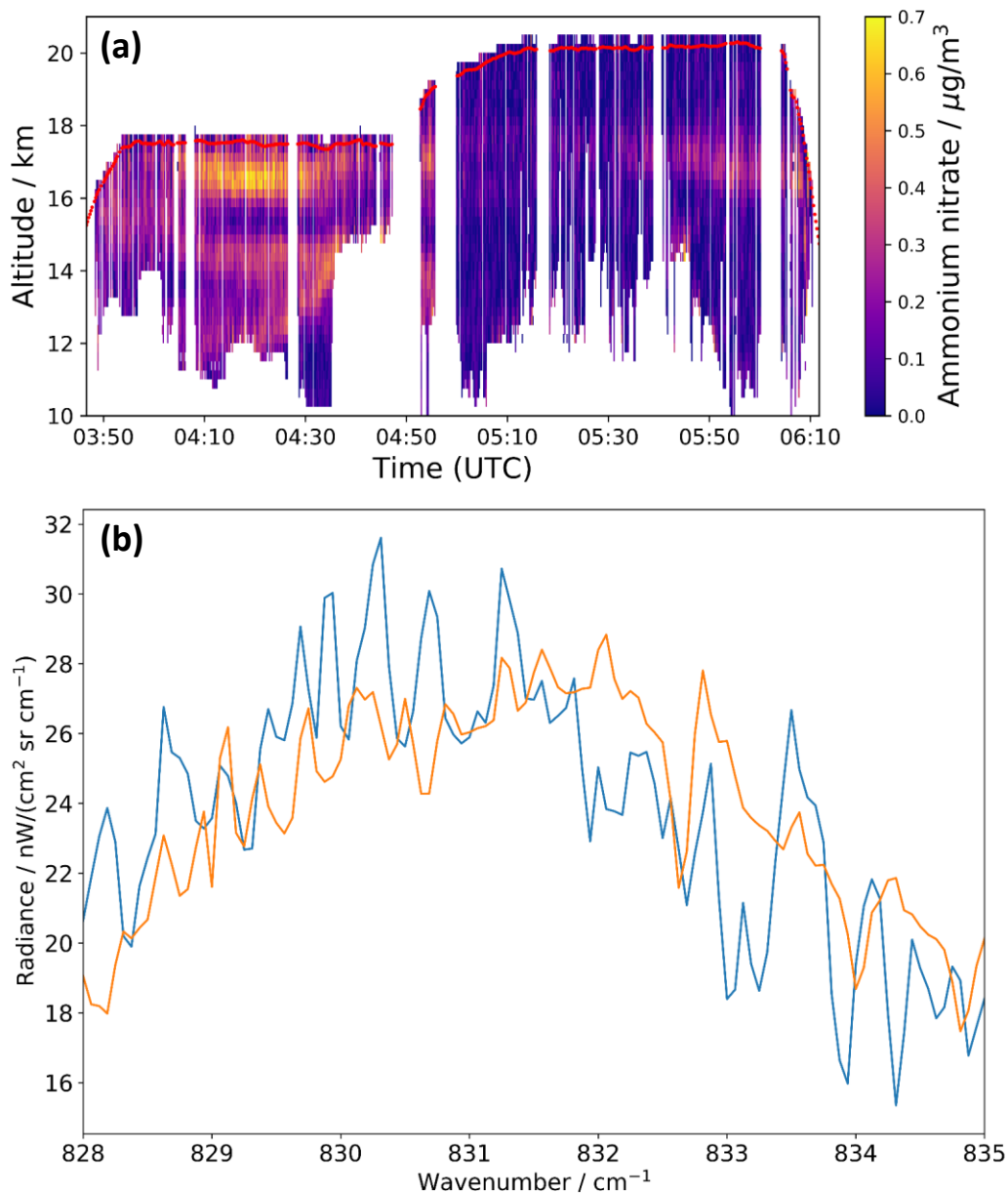
655 Figure 6: (a) AN mass concentrations retrieved from GLORIA measurements during the StratoClim research flight on 31 July 2017 using the n(\tilde{\nu}_x) = 1.56 , \chi = 1.1 , and \phi = 1 refractive index data set (see Fig. 3b in Höpfner et al. (2019) as a comparison). Red line: aircraft altitude. (b) Difference of mean GLORIA spectra between 04:15 – 04:21 and 04:35 – 04:43 UTC at 16.5 – 16.75 km altitude (blue) and best spectral fit with the AN optical constants (orange) in the range of the \nu_2(\text{NO}_3^-) mode.
