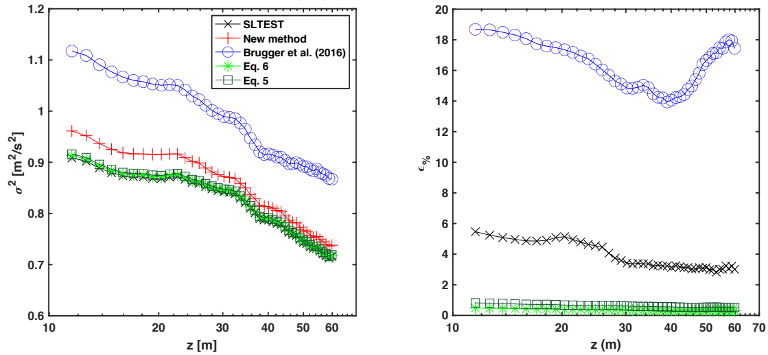
Figure 12. Correction of the streamwise velocity variance with different methods for the SLTEST dataset: (a) streamwise velocity variance; (b) percentage correction of the velocity variance, \epsilon\% . The marker colors are black for the raw LiDAR data, red for the proposed method, light green for Eq. 6, dark green for Eq. 5, and blue for the method proposed by Brugger et al. (2016).
