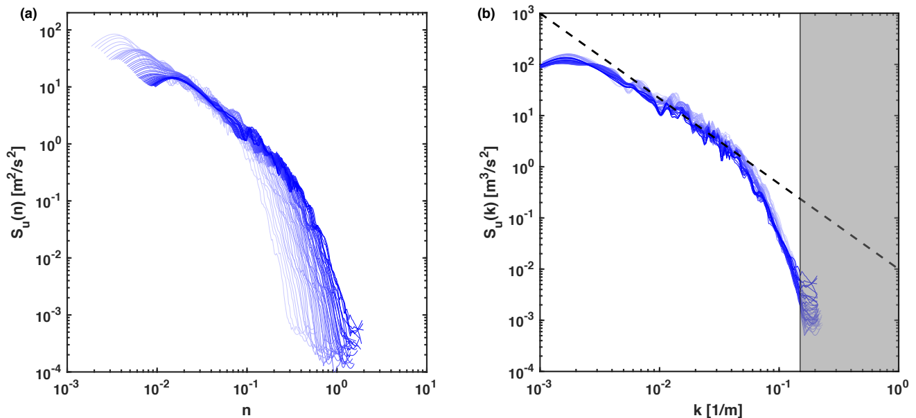
Figure 8. Velocity spectra for the SLTEST dataset at different heights: (a) spectra as a function of the reduced frequency, n ; (b) spectra as a function of the wavenumber , k . Line color is darker with increasing height. The black dashed line represents the -5/3 slope. In (b), the shaded area covers the noisy part of the velocity spectra.
