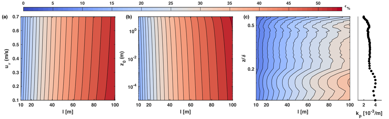
Figure 13. Variation of the percentage variance damping, \epsilon_{\%} connected with the LiDAR spatial averaging for different probe lengths and wind conditions: (a) variability with the friction velocity, u_{\tau} ; (b) variability with the aerodynamic roughness length, z_0 ; (c) variability with sampling height, z . The side panel of (c) reports the vertical profile of the parameter k_p estimated for the SLTEST dataset.
