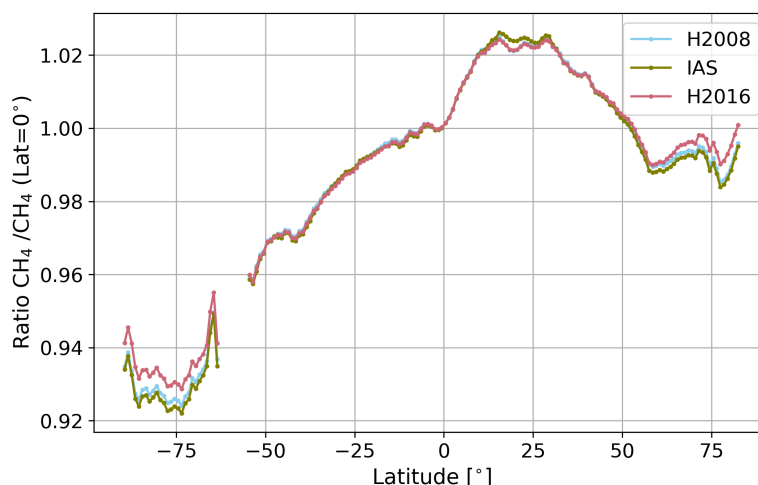
Figure 1. Latitudinal distribution of TROPOMI \text{XCH}_4 retrieved using HITRAN 2008 (blue), HITRAN 2016 (pink) and SEOM-IAS (green), referenced to the value at 0^\circ latitude. Daily measurements from Sep 2018 – Sep 2019 are gridded into a 0.2^\circ \times 0.2^\circ grid, averaged longitudinally and then binned in 1^\circ latitude.
