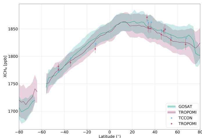
Figure 11. Latitudinal distribution of XCH_4 measured by TROPOMI and GOSAT, and the TROPOMI and TCCON collocations over the selected stations for validation in Sect. 4. The shaded bands indicate the scatter (i.e. 1\sigma standard deviation) around the mean.
