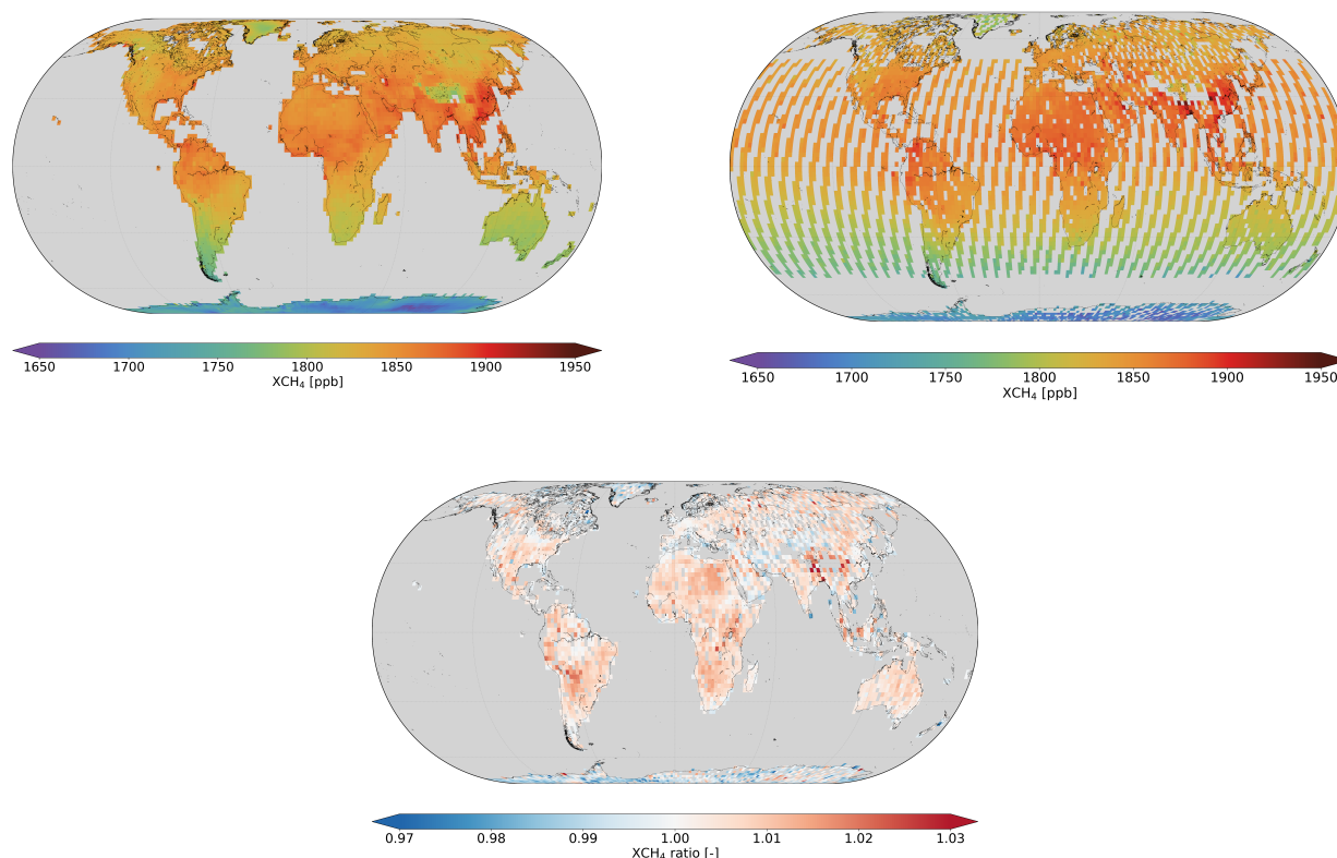
Figure 10. Global distribution of XCH_4 measured by (a) TROPOMI, (b) GOSAT and (c) the ratio of GOSAT to TROPOMI XCH_4 . Daily collocations are averaged to a 2^\circ \times 2^\circ grid for the period 1 Jan 2018 – 31 Dec 2019.
