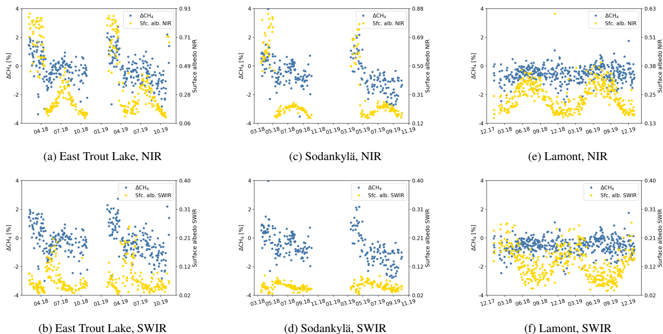
Figure 9. Daily mean relative differences (blue, left axis) between TROPOMI and TCCON XCH_4 ( \Delta CH_4 ) and surface albedo in the NIR (yellow, secondary axis, first row) and surface albedo in the SWIR (yellow, secondary axis, second row) at East Trout Lake ( 54.3^\circ N ) (first column), Sodankylä ( 67.4^\circ N ) (second column) and Lamont ( 36.6^\circ N ) (third column).
