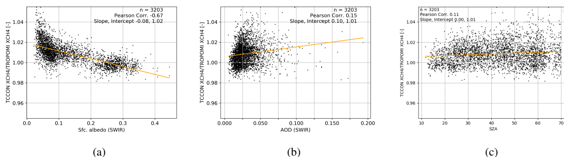
Figure 3. Ratio of \text{XCH}_4 measurements by TCCON and TROPOMI as a function of (a) retrieved surface albedo in the SWIR spectral range, (b) retrieved effective aerosol optical depth (AOD) in SWIR spectral range and (c) solar zenith angle (SZA).
