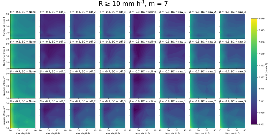
Figure B2. Overall RMSE for observations \geq 10 \text{ mm h}^{-1} as a function of number of trees, maximum depth, \beta parameter and bias-correction method. The maximum number of randomly chosen variables at each split is here set to 7.
