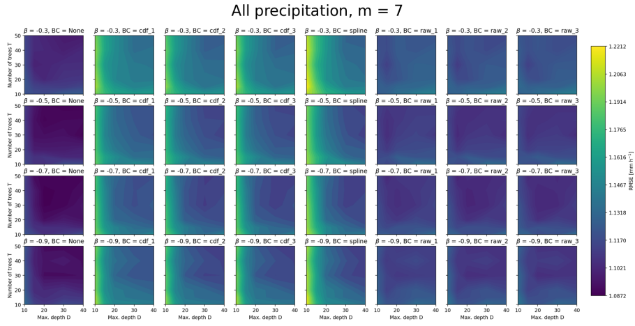
Figure B1. Overall RMSE, for all observations as a function of number of trees, maximum depth, \beta parameter and bias-correction method. The maximum number of randomly chosen variables at each split is here set to 7.
