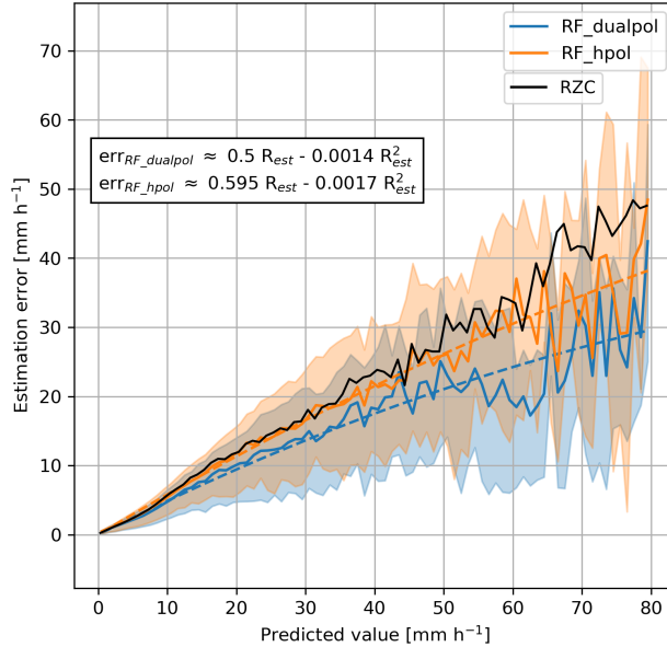
Figure 12. Absolute error of the precipitation estimate as a function of the precipitation estimate, evaluated over 5 iterations of 5-fold cross-validation, for the two RF models. The coloured semi-transparent area corresponds to the Q25-Q75 interquartile, the solid lines to the mean, and the dashed line to a polynomial fit, which formulation is shown in the box on the left. The black solid line corresponds to the average error of the RZC model which is shown as a reference. All quantiles and means have been obtained using a discretization on the predicted values with a step of 1 \text{ mm h}^{-1} .
