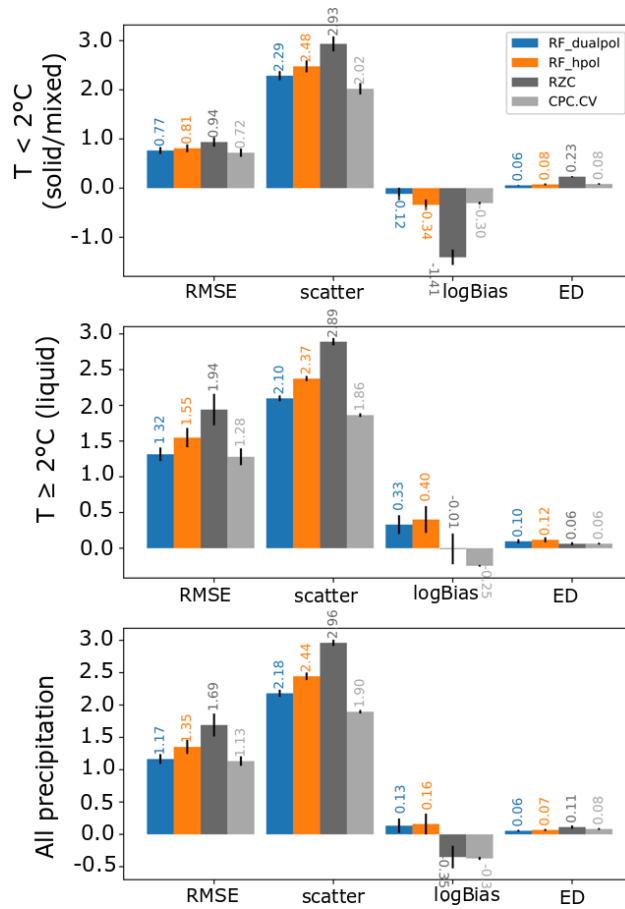
Figure 8. Overall performance metrics of the fitted RF models and the references for a 5-fold cross-validation. The small black lines at the center of the bars indicate the standard deviation of the metrics over the 5-fold cross-validation.
