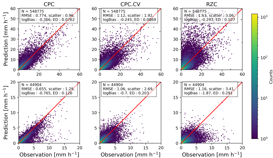
Figure 4. Scatter-plots and performance scores of the reference products CPC, CPC.CV and RZC for all available observations (upper row) and for observations with T < 2^\circ C (lower row). The 1:1 line is shown in red. The colorbar gives the counts in logarithmic scale.
