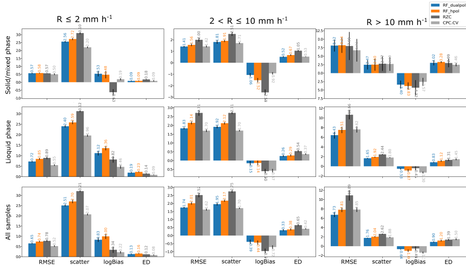
Figure C1. 5-fold cross-validation performance of RZC, CPC.CV, RF_dualpol and RF_hpol for different observed precipitation ranges for liquid and solid/mixed precipitation and for both together (which includes all additional observations from stations where no temperature measurement is available). The y-scale is different for all precipitation ranges, since the scores are significantly different.
