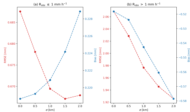
Figure D1. Hourly RMSE and linear bias (average of estimated vs observed value), as a function of the value of \sigma , (a) for low intensities, (b) for higher intensities.
