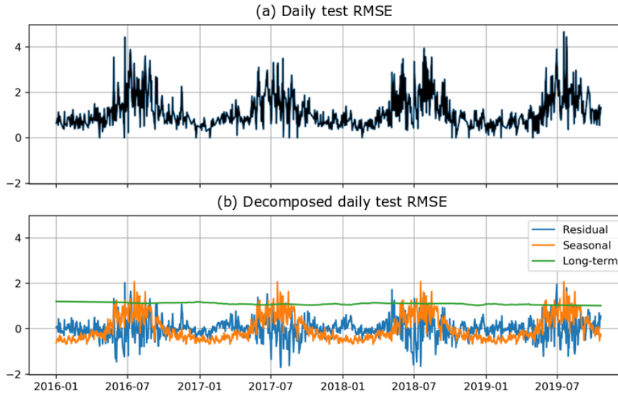
Figure 7. (a) Average daily test RMSE obtained from a 5-fold cross-validation, (b) daily test RMSE decomposed into seasonal and long-term trends, and fluctuations from these two trends.
