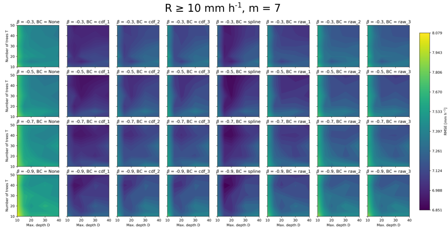
Figure B2. Overall RMSE for observations \geq 10 \text{ mm h}^{-1} as a function of number of trees, maximum depth, \beta parameter and bias-correction method. The maximum number of randomly chosen variables at each split is here set to 7.
