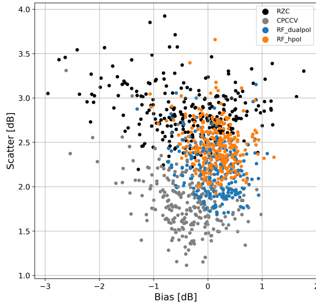
Figure 11. logBias versus scatter at every ground station for RF_dualpol, RF_hpol, RZC and CPC.CV. Every dot corresponds to a different station.
