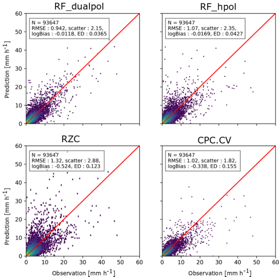
Figure 9. Example of prediction versus observations scatter-plots on the test fraction for one cross-validation iteration. The 1:1 line is shown in red.
