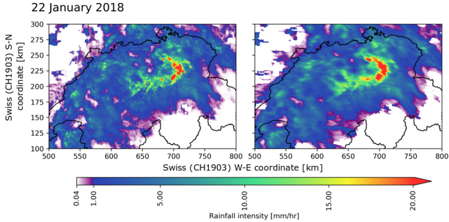
Figure 13. Resulting QPE field on a case of widespread snowfall, on the left with Gaussian smoothing ( \sigma = 0.5 pixels), on the right with advection correction.
