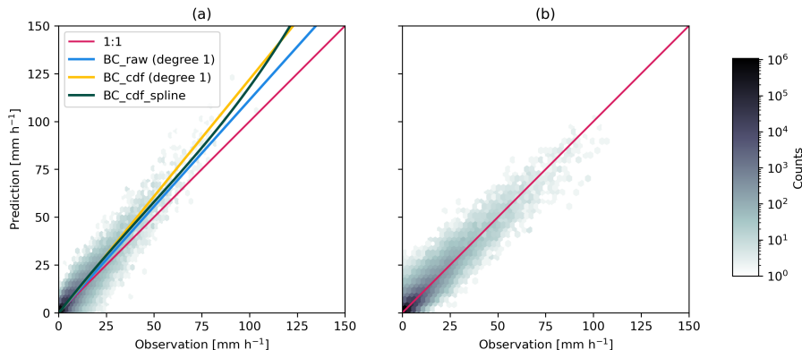
Figure 3. Panel (a) shows an example of raw uncorrected predictions (as a density plot) versus observations on the training fraction. The blue, yellow and dark green lines are the corresponding fitted bias-correction models, which try to estimate the observed value as a function of raw predicted values. Panel (b) shows the raw predictions corrected with the BC_cdf_spline method (dark green line in the panel (a)), which brings them much closer to the 1:1 line.
