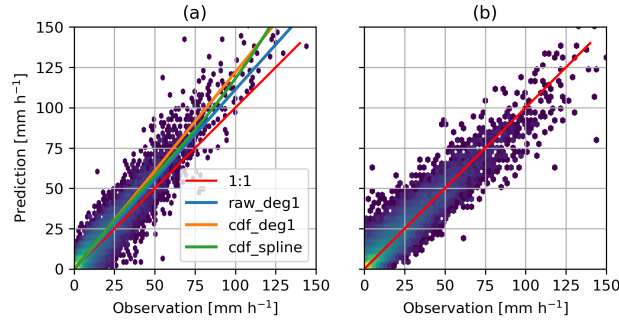
Figure 3. Panel (a) shows an example of raw uncorrected predictions (as a density plot) versus observations on the training fraction. The blue, orange and green lines are the corresponding fitted bias-correction models, which estimate the observations as a function of raw predicted values. Panel (b) shows the raw predictions corrected with the BC_cdf_spline method, which brings them much closer to the 1:1 line.
