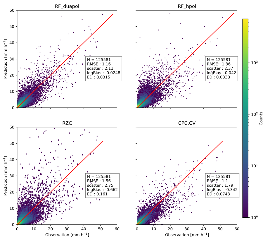
Figure 9. Example of prediction versus observations scatter-plots on the test fraction for one cross-validation iteration. The 1:1 line is shown in red.
