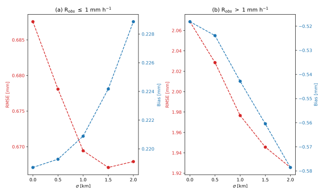
Figure D1. Hourly RMSE and linear bias (average of estimated vs observed value), as a function of the value of \sigma , (a) for low intensities, (b) for higher intensities.
