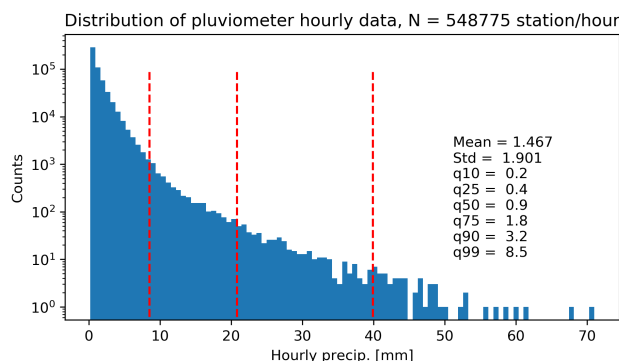
Figure 2. Distribution and statistical indicators of hourly observed precipitation intensities for the entire database (January 2016 to December 2019). The three vertical dashed red bars indicate the percentiles 99, 99.9 and 99.99.
