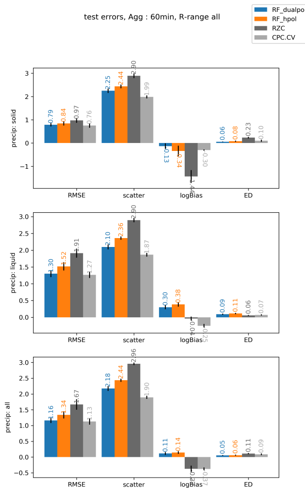
Figure 8. Overall performance metrics of the fitted RF models and the references for a 5-fold cross-validation. The small black lines at the center of the bars indicate the standard deviation of the metrics over the 5-fold cross-validation.
