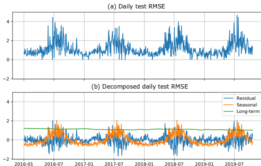
Figure 7. (a) Average daily test RMSE obtained from a 5-fold cross-validation, (b) test RMSE decomposed into daily fluctuations, seasonal trend and long-term trend.
