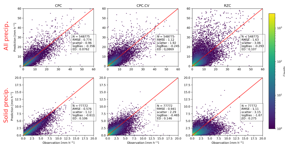
Figure 4. Scatter-plots and performance scores of the reference products CPC, CPC.CV and RZC for all available observations (upper row) and for observations with T < 2^{\circ}\text{C} (lower row). The 1:1 line is shown in red. The colorbar gives the counts in logarithmic scale.
