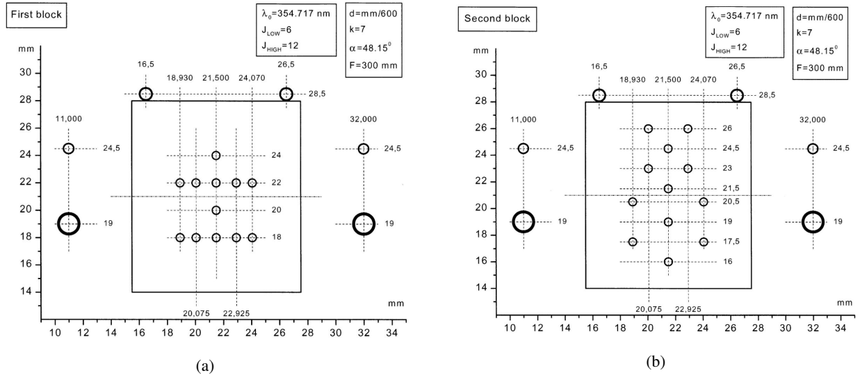
Figure 6. The outline of the two fibers' blocks shows the positions of the input, output and intermediate (from stage-1 to stage-2) fibers as a function of the abscissa-ordinate , x - y Cartesian's coordinates . (a) Two optic fibers transmitting the PRR and the elastic signal enter the temperature polychromator through the first fibers' block. (b) The eight Stokes and Anti-Stokes J -signals are transmitted through the intermediate fibers into the second fibers' block. The eight J -signals are recombined by the diffraction grating polychromator into two groups of total J -signals ( J_{\text{high}} and J_{\text{low}} ) and sent to the output fibers. Holes shown outside the fiber's block are not fibers' holders.
