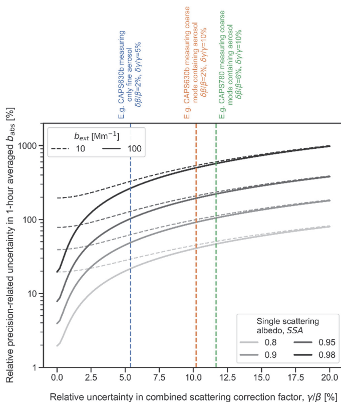
1505 Figure 4: Theoretically-calculated relative uncertainty in 1-hour averaged CAPS PM 2.5 b_{abs} measurements as a function of the relative uncertainty in the combined scattering correction factor (defined in Eq. 6 using the ratio of the truncation correction factor \gamma and the instrument cross-calibration factor \beta ). Curves are shown for four different SSA values (grey shading) and two different aerosol loadings ( b_{ext} of 10 and 100 Mm^{-1} ). The curves were generated using the error model presented in Sect. 2.3 and Appendix A2 with inputs that were chosen to represent instrument characteristics during the Cabauw field campaign, as detailed in the main text.
