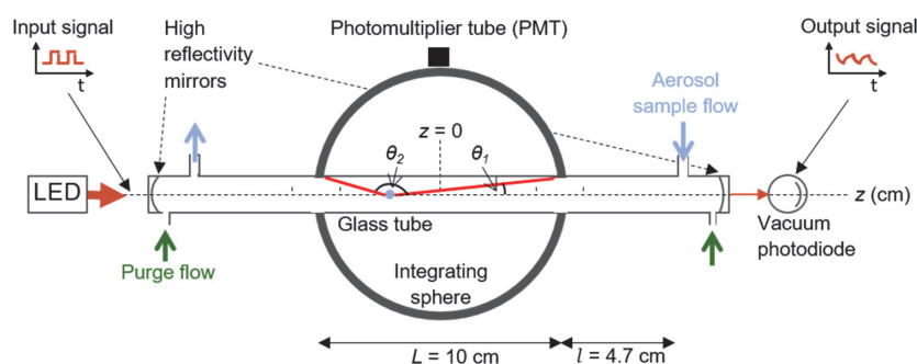
Figure 1: Schematic diagram of the CAPS PMssa monitor with relevant components and variables highlighted. A glass tube encapsulates the aerosol sample to be measured. A light-emitting-diode (LED) delivers a square-wave modulated light signal as input to the optical cavity. The phase shift of the output signal from the cavity relative to the input signal is measured by a vacuum photodiode: this is the extinction channel of the instrument. Light scattered from the aerosol sample is collected by the integrating sphere and measured with a photomultiplier tube (PMT): this is the scattering channel of the instrument. \theta_1 and \theta_2 are the two truncation angles for light scattered from a particle at position z along the instrument axis (without considering reflection from the glass tube).
