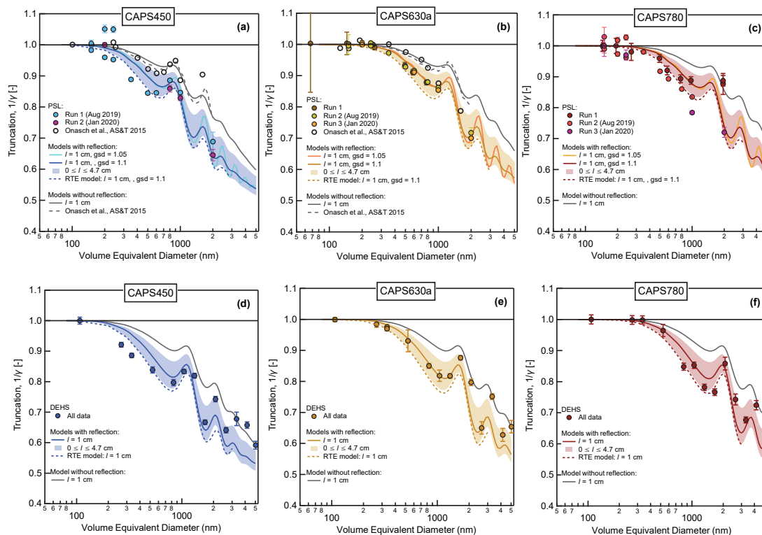
Figure 6: Measured and modeled truncation values as a function of volume equivalent particle diameter for PSL and DEHS aerosols. The truncation values plotted on the y-axis correspond to the inverse of the truncation correction factor \gamma defined by Eq. (4). Modeled curves were calculated with the truncation model presented in Appendix 1 as well as the radiative transfer equation (RTE) model presented by Liu et al. (2018). The parameter l represents the extra path length beyond the integrating sphere, and gsd refers to the geometric standard deviation of the modeled test aerosols.
