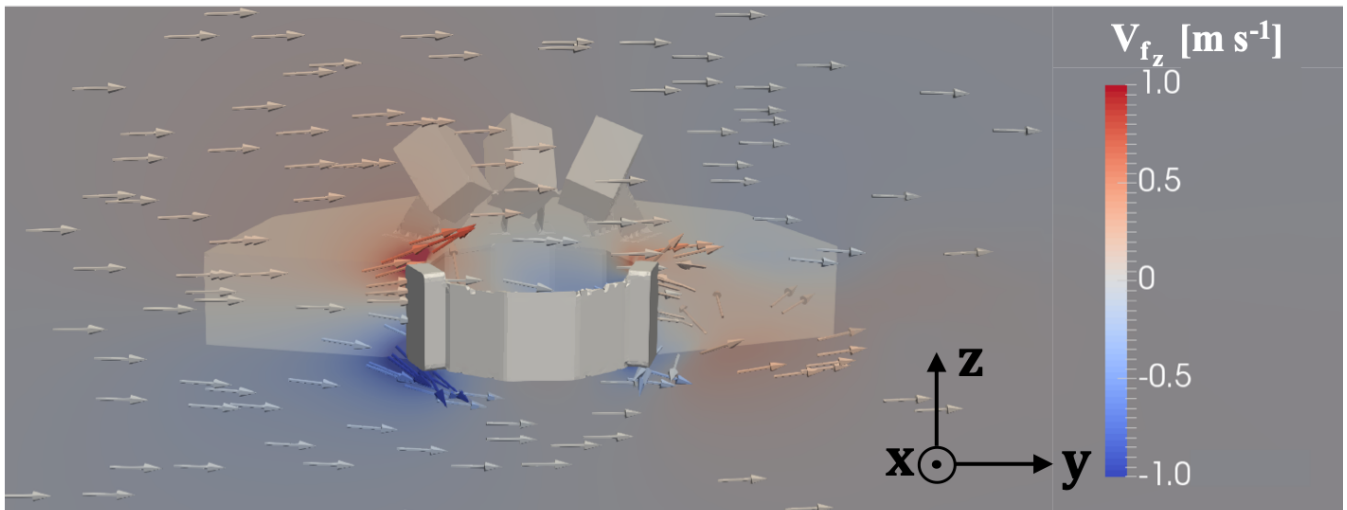
Figure 13. Simulated wind field around the MASC with undisturbed winds set at 1 \text{ m s}^{-1} towards the +y direction. Color represents the vertical wind speed v_{f_z} , and arrows show wind directions on the y - z plane. The plane in which the arrows are located is aligned with the center of the aperture on the y - z plane, and x -positive points out of the page.
