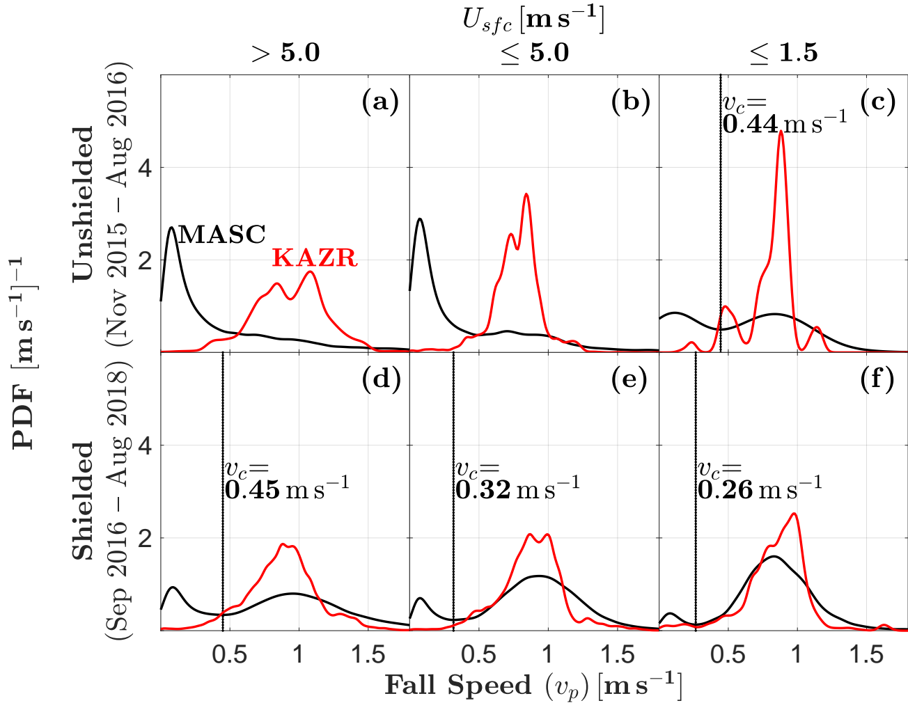
Figure 5. Comparison of MASC hydrometeor fall speed and KAZR mean Doppler fall speed PDF estimates for (a)–(c) unshielded and (d)–(f) shielded MASC measurements. Surface wind speeds U_{sfc} decrease from left to right. Where MASC PDFs are bimodal, the vertical line marks the cutoff fall speed v_c , indicating the location of the local minimum separating the two modes. The number of observations for each case is listed in Table 1. The terms “shielded” and “unshielded” refer only to the MASC. Unshielded and shielded MASC observations are from two separate periods: 29 November 2015 to 21 August 2016 and 22 August 2016 to 28 August 2018, respectively.
