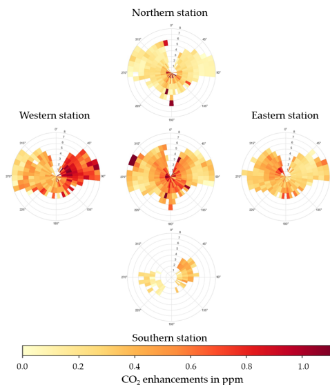
Figure 12. Concentration enhancements over the background for each of the five stations displayed as a polar histogram. The CO 2 enhancements are represented by the different colors (low=yellow to red=high). The wind direction is indicated by the location of the respective cells in the circle and the wind speed by the distance of the cells to the center point.
