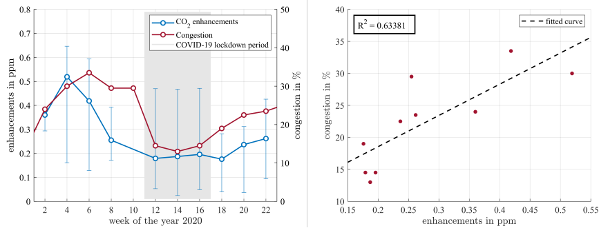
Figure 13. Correlations between the CO 2 enhancements over the background measured at our inner city station in Munich, and the traffic amount represented by the congestion rate (left: time series, right: regression plot). The time period includes the COVID-19 lockdown in spring 2020. We show the median trend of all column concentration gradients clustered into biweekly bins. The error bars show the 1\sigma standard deviation of all enhancements within the respective two-week period. Traffic data are from ©2020 TomTom International BV.
