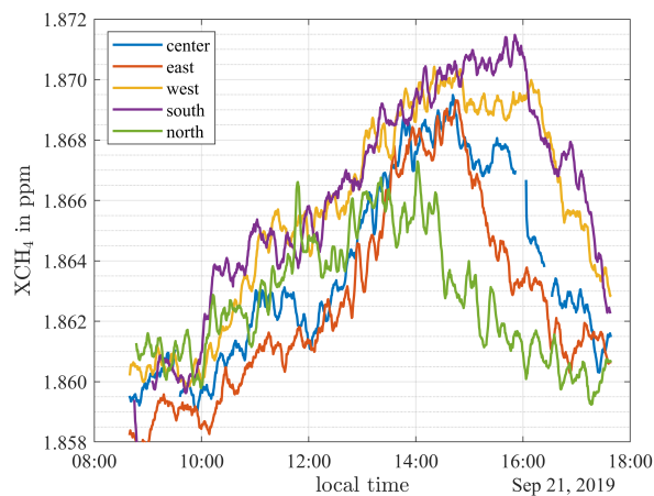
Figure 11. CH 4 measurement values (5-minute average) from all five stations during our Oktoberfest 2019 campaign on September 21, 2019. The concentration gradients between the single stations are clearly visible, which indicates the presence of strong CH 4 sources in the city.
