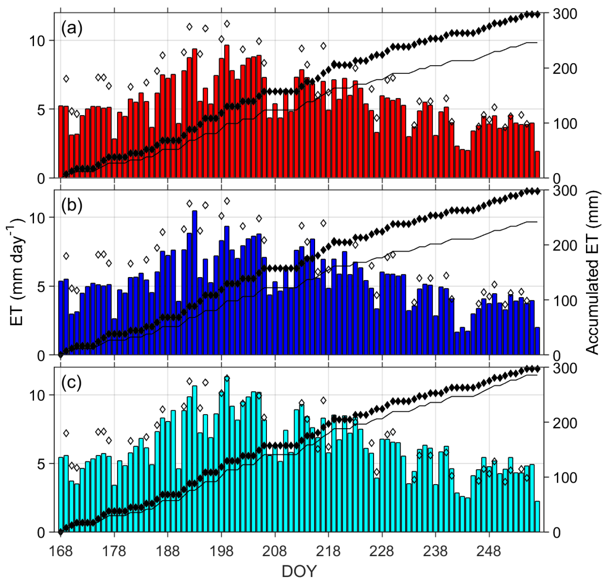
585 Figure 7: Daily ET determined with (a) LI-7500RS (red), (b) LI-7500A (blue), and (c) LI-7500 (cyan). The daily lysimeter ET is displayed by open diamond markers. Accumulated lysimeter ET is shown with solid diamonds and accumulated eddy covariance ET measurements with solid lines.
