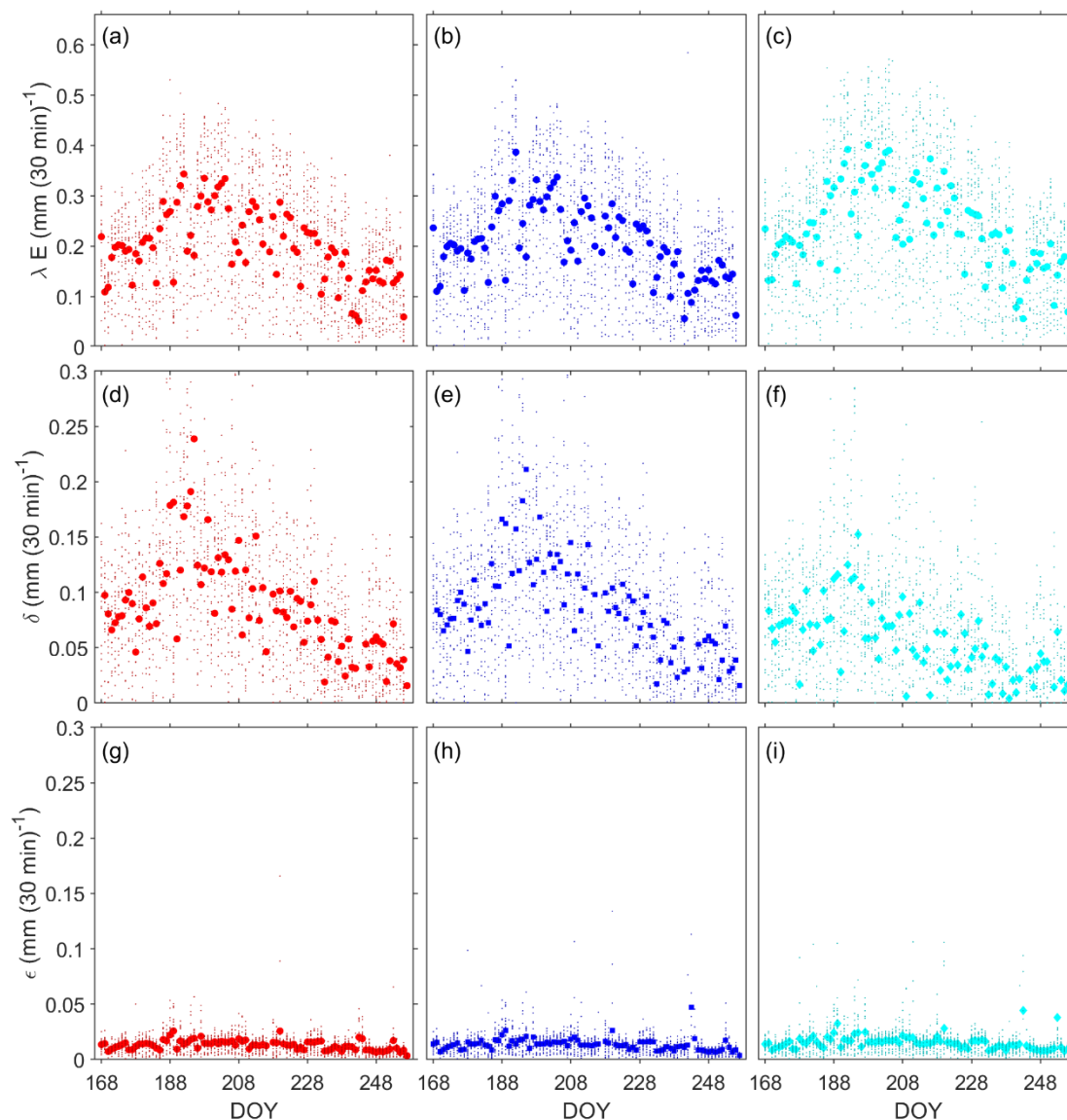
590 Figure 8: Daytime (9 AM–7 PM LST) ET fluxes for EC systems with an (a) LI-7500RS, (b) LI-7500A, and (c) LI-7500 and the accompanying systematic errors (d–f) and random errors (g–i). Mean values are displayed as larger points.
