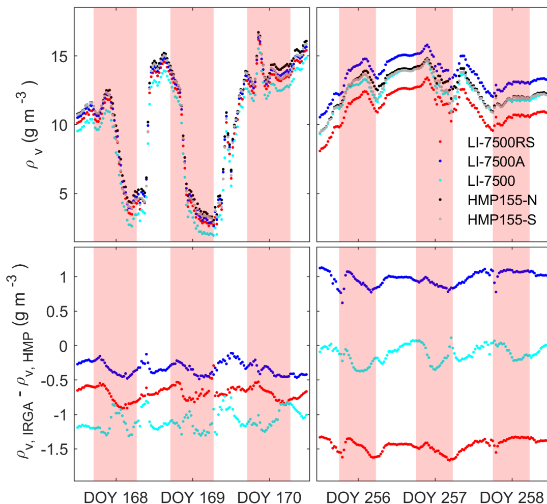
Figure 2: Absolute humidity \rho_v (top) magnitude and (bottom) difference \Delta\rho_v between paired IRGA and HMP instruments (HMP155-N is paired with the LI-7500RS and LI-7500A; HMP155-S is paired with the LI-7500) during the first and last three days of the study. Shaded areas indicate daytime.
