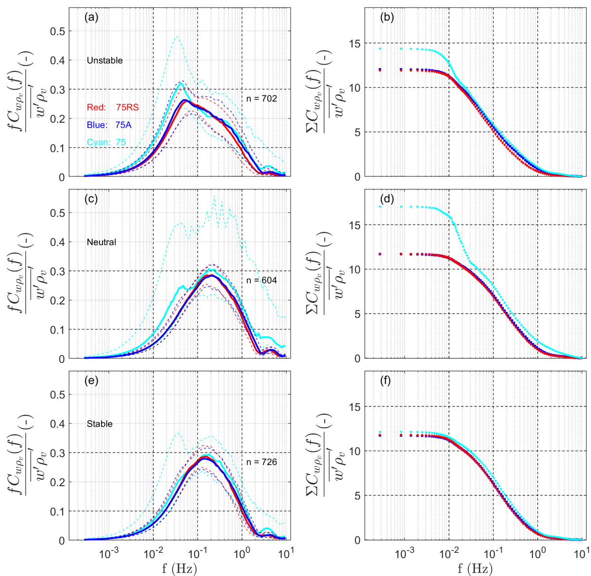
Figure 6: Ensemble median daytime (a, c, and e) cospectra and corresponding (b, d, and f) ogives under unstable, neutral, and stable conditions. For cospectra, the area between dotted lines shows the interquartile range.
