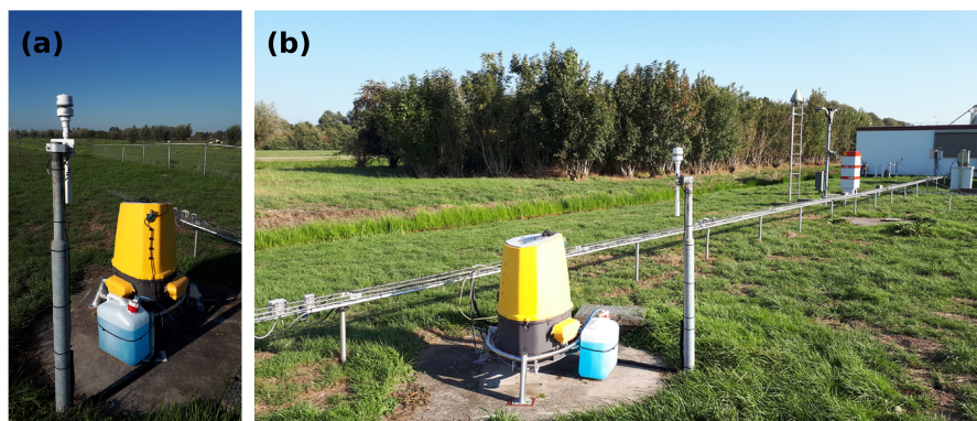
Figure 14. Photos of (a) the meteo station of ZephIR 300 instrument located on a separate pole and (b) a view to the South-East direction, showing building on RSS and nearby trees.
