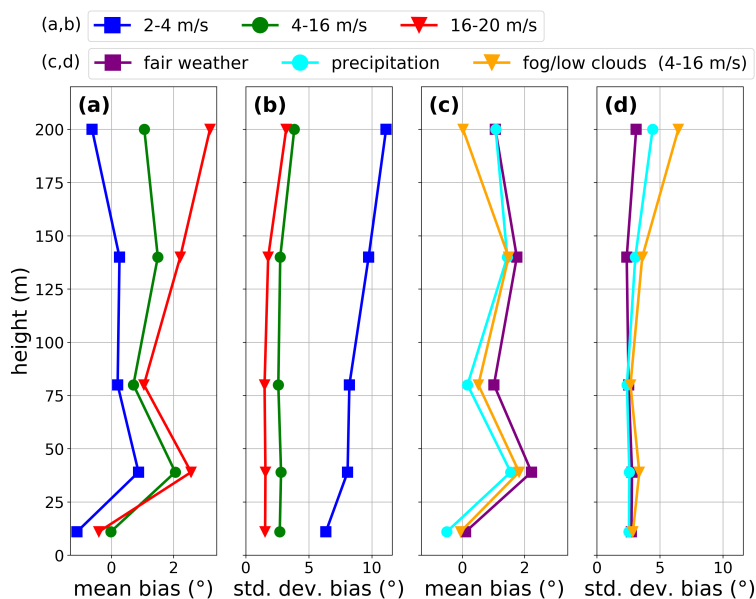
Figure 11. Profiles of the biases in the wind direction for different wind speed classes and meteorological conditions. Panels (a) and (b) show the mean bias and standard deviation of the bias applied to three different wind speed classes: 2-4 m/s (blue squares), 4-16 m/s (green circles) and 16-20 m/s (red triangles). Panels (c) and (d) show the mean bias and standard deviation of the bias applied to three different meteorological conditions (and wind speed is bounded to the 4-16 m/s range): fair weather (purple squares), precipitation (cyan circles) and fog/low clouds (orange triangles).
