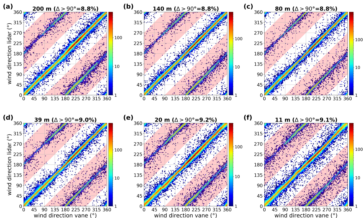
Figure 12. Wind direction comparison between wind lidar and mast data for the different heights: (a) 200 m, (b) 140 m, (c) 80 m, (d) 39 m, (e) 20 m and (f) 11 m. Compared to Fig. 10, here all wind directions the 20 m level are included. The regions of incorrectly assigned wind direction are indicated in red; the percentage of data in those areas are indicated on top of each panel.
