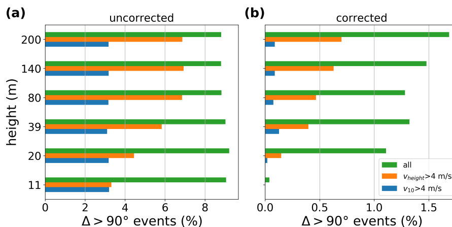
Figure 13. Panel (a): histogram of the \Delta > 90^\circ events for the different measuring heights, based on either all events (green), wind speeds at the measuring height larger than 4 m/s (orange) and 10 m wind speeds than 4 m/s (blue). Panel (b): same as Panel (a) but after application of the correction scheme (see text), based on information from the 10 m mast wind vane.
