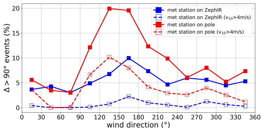
Figure 15. The \Delta > 90^\circ occurrence for the lowest measuring height of 11 m for different wind sectors (binsize 30^\circ ), separating the data regarding the location of the meteo station and including a wind speed threshold of 4 m/s (as measured at 10 m).
