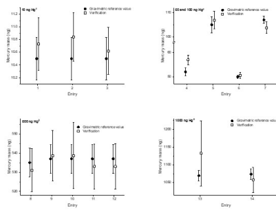
Figure 2. Verification results of the second comparison with mercury amounts of approximately 10, 50, 100, 500 and 1000 ng on sorbent tubes. The open squares are the verification results. The closed circles are the reference values determined gravimetrically. The error bars indicate the expanded uncertainty for the reference value (ng) ( k=2 ) and the verification value (ng) ( k=2 ).
