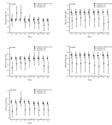
Figure 1. Verification results of the first comparison with mercury amounts of approximately 2, 4, 6, 8 and 10 ng on sorbent tubes. The open squares and triangles are the results from the measurement calibrated with the Dumas equation. The closed circles are the reference values determined gravimetrically. The error bars indicate the expanded uncertainty for the reference value (ng) ( k=2 ) and the verification values (ng) ( k=2 ). Entry 1.1, 1.2 and 1.3 show the verification results of VSL from the first round. The verification results of NPL in the first round are entry 1.4 and 1.8, in the second round 2.1 and 2.2 and in the third round 3.1 and 3.2.
