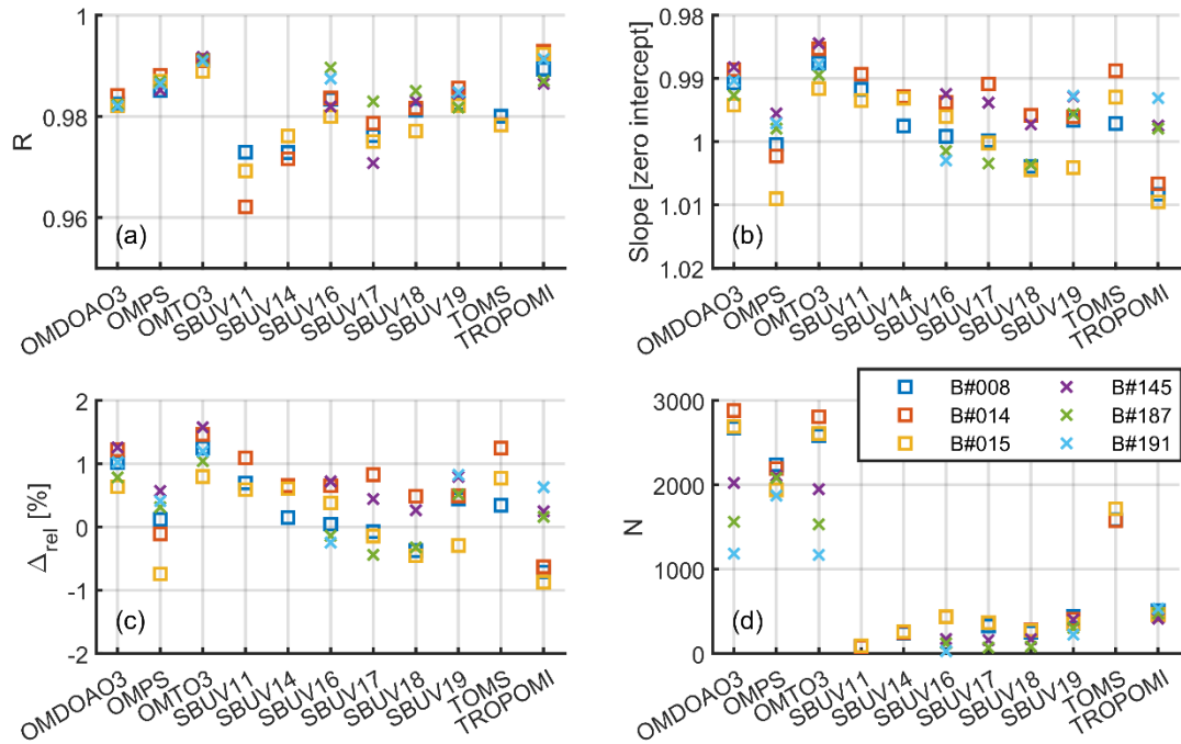
475 Figure 67. Summary of the regression analysis between satellites and the world Brewer reference triads. The four panels represent the (a) correlation coefficient ( R ) between individual Brewer instruments and different satellites (labelled at the bottom axis), (b) the slope of the zero intercept regression line (multiplicative bias), (c) relative percentage difference (bias), and (d) the total number of coincident observations.
