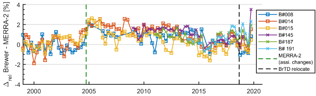
Figure 78. The relative difference between the reference Brewers and MERRA-2 reanalysis. Each point represents a 3-month average. The green dash line represents the time when MERRA-2 changed its assimilation sources from SBUV-2 to MLS/OMI (causing about 2% relative difference). The black dash line represents the time when BrT-D was relocated to Egbert.
