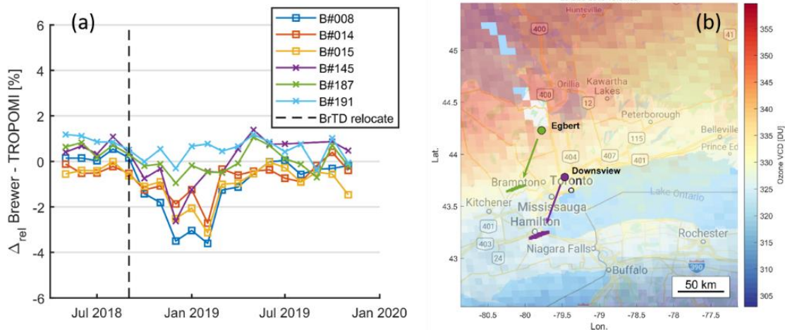
Figure 89. Example of small scale column ozone field variation. (a) Monthly relative differences between Brewers and TROPOMI total column ozone overpass measurements (for Downsview in Toronto) and (b) TROPOMI total column ozone measured on 29 December 2018 over southern Ontario, masked with Brewers' viewing directions and sampling areas. The base map is from © Google Maps.
