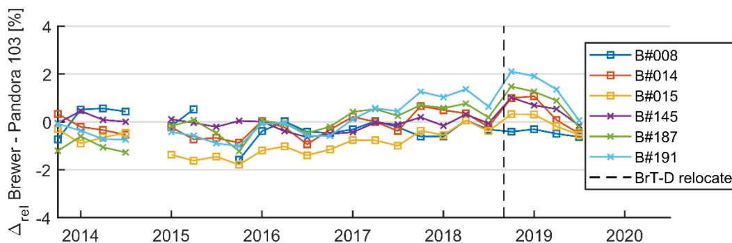
Figure 34. 3-month relative differences between Brewers and Pandora total column ozone. 3-month averages are calculated if there are at least ten coincident measurements between Brewer and Pandora for that period. The black dash line represents the time when BrT-D was relocated to Egbert, i.e., Pandora and BrT-D were not co-located.
