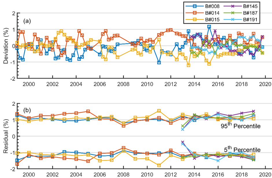
Figure 12. Model 1 estimated deviations and residual of ozone values. (a) Deviations of ozone values of individual triad Brewers from the mean of the three instruments. Each point on (a) represents a 3-month average. Panel (b) shows the 5 th and 95 th percentiles of the residuals of the Model 1 analysis. Each point on (b) is based on one year of data.
