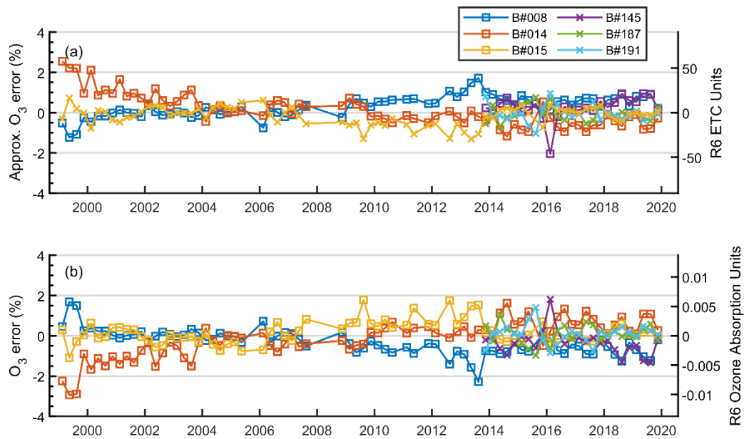
405 Figure 23. Relative systematic uncertainties in ETCs and effective ozone absorption coefficients estimated using Model 2. The right y-axes represent the values in the units used in the actual Brewer algorithm (i.e., R6 ratio units); the left y-axes demonstrate the % values of these errors in total ozone values. Each point on the graph represents a 3-month average.
