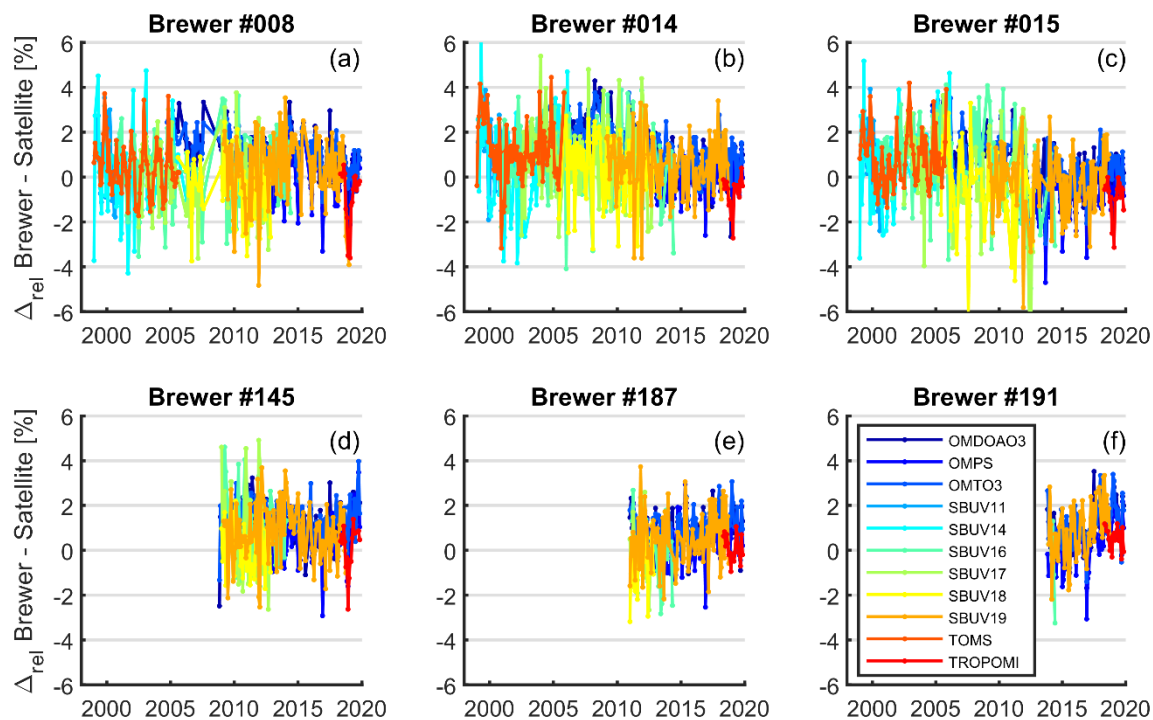
Figure 56. The relative difference between satellites and the world Brewer reference triads (BrT and BrT-D). Each point represents a 3-month average. Brewers and satellite data are paired with the criteria shown in Table 3.
