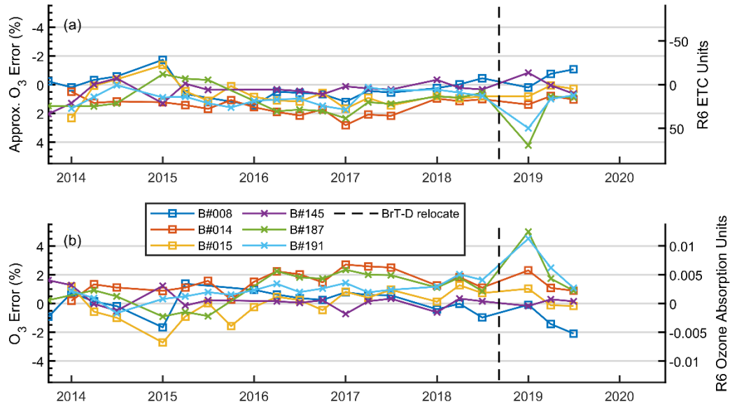
Figure 45. Relative systematic uncertainties in ETCs and effective ozone absorption coefficients estimated using Model 3. Description of y-axes is in Fig. 23. Each point on the graph represents a 3-month average. The black dash line represents the time when BrT-D was relocated to Egbert.
