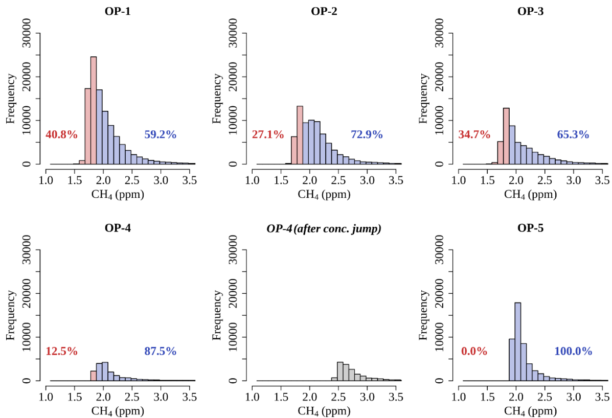
Figure 2: Histograms of recorded 1-minute average concentrations of GF3 devices OP-1, OP-2, OP-3, OP-4 and OP-5. Few values greater than 3.5 ppm are not shown. Blue: values > 1.88 ppm, red: values <= 1.88 ppm. Grey: Data from device OP-4 during the campaign H19-3 that passed the quality check but have been omitted in the analysis due to an obvious jump in the concentration (Figure 3).
