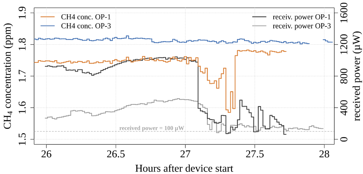
Figure 4: Example of a concentration dent followed by a step change related to losses in the received power of device OP-1. The data were recorded during the intercomparison campaign K19 on 2019-04-26 between 2am and 4am. From hour 27 onwards, the data exhibit R2 values above 0.98.
