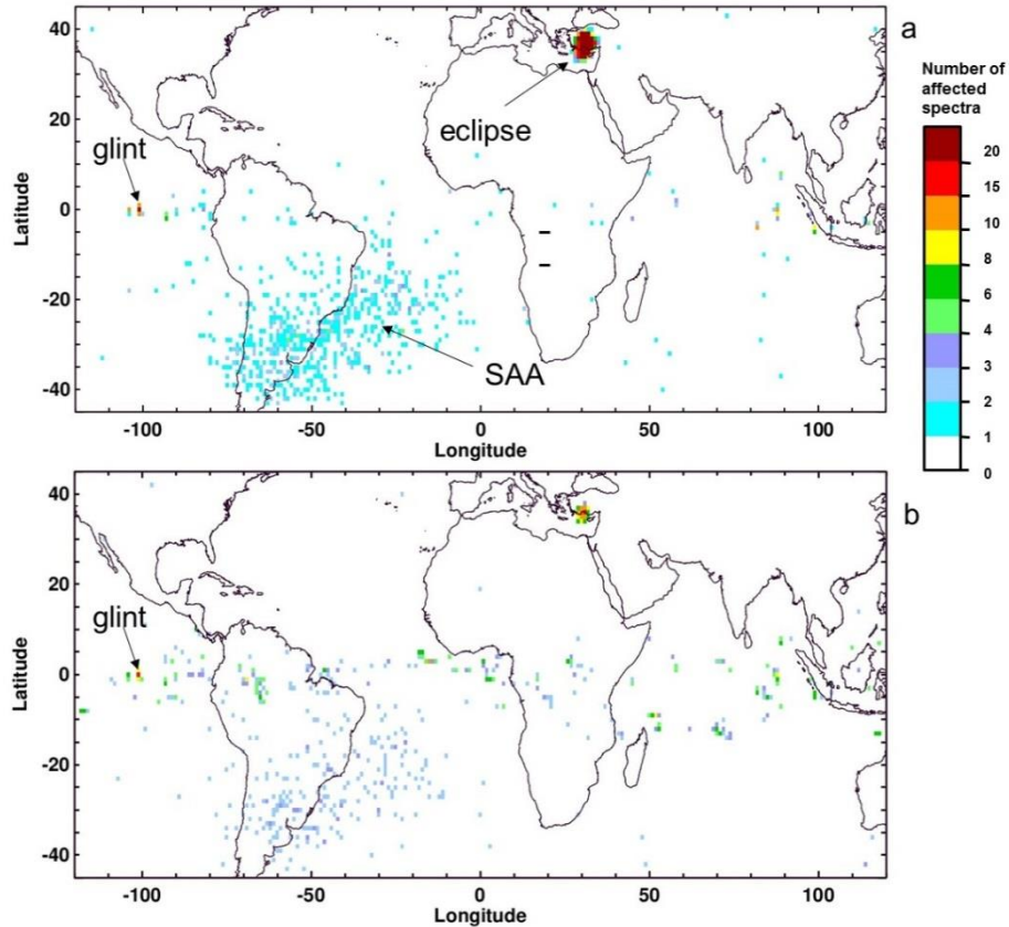
325 Figure 8: Gridded ( 1^\circ \times 1^\circ ) distributions of the number of affected spectra for March 2006; (a) Vis band 424.1-434.5 nm, DI > 0.03; (b) Vis 445.3-455.7 nm, DI > 0.25. The South Atlantic Anomaly (SAA) and a region affected by solar eclipse are clearly visible; the remaining pixels with high DI values are mostly associated with sun glints and bright clouds.
