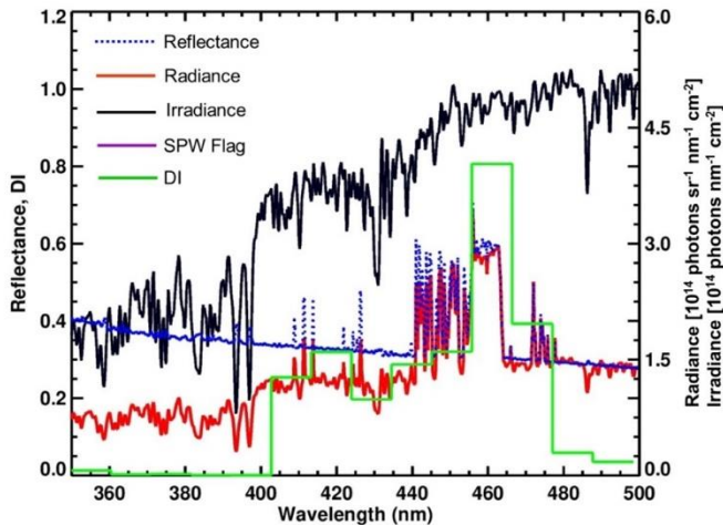
Figure 6: Similar to Fig. 5 but for pixel iTTime 823, row 11, orbit 7987 (see arrows in Fig. 4d). SPW flags are zero for this case and are not shown.
