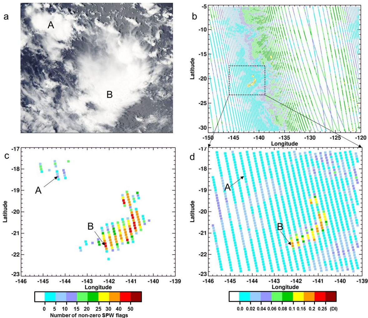
215 Figure 1: a. Two cloud zones in the south Pacific on January 14, 2006 for orbit 7990: small northern zone labeled “A” and large southern labeled “B” (a) Aqua MODIS image; (b), (d) DI maps for the Vis spectral region 414-424 nm; (c) The number of wavelengths for a given pixel marked with the SPW (Saturation Possibility Warning) flag as saturated (the maximum number is 51 in this Vis spectral region).
