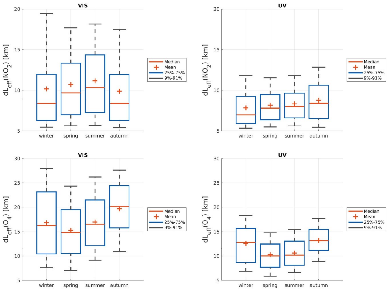
Figure 8: Upper panels show the box and whisker plots representing the seasonal horizontal sensitivity as derived from all the azimuthal viewing directions by applying the parameterization method for the Vis (left panel) and UV (right panel) spectral ranges. Every seasonal box contains the estimated dLeff (NO 2 ) of all the azimuthal viewing directions. Lower panels show the corresponding estimates of dLeff (O 4 ).
