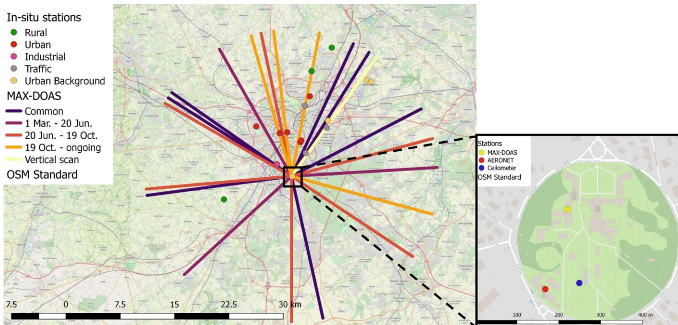
5 Figure 1: The dual-scan experimental set-up of the BIRA-IASB MAX-DOAS instrument (overlaid onto Open Street Map (OSM) Standard layer) (Left panel). The lines are color coded according to the three different experimental set-ups (Table 1), with a line length of 20 km each. The colored dots show the different types of in-situ stations around the MAX-DOAS instrument (see Section 4.2). Right panel shows the location of the MAX-DOAS, AERONET and ceilometer instruments at the measurement site. © OpenStreetMap contributors 2019. Distributed under a Creative Commons BY-SA License.
