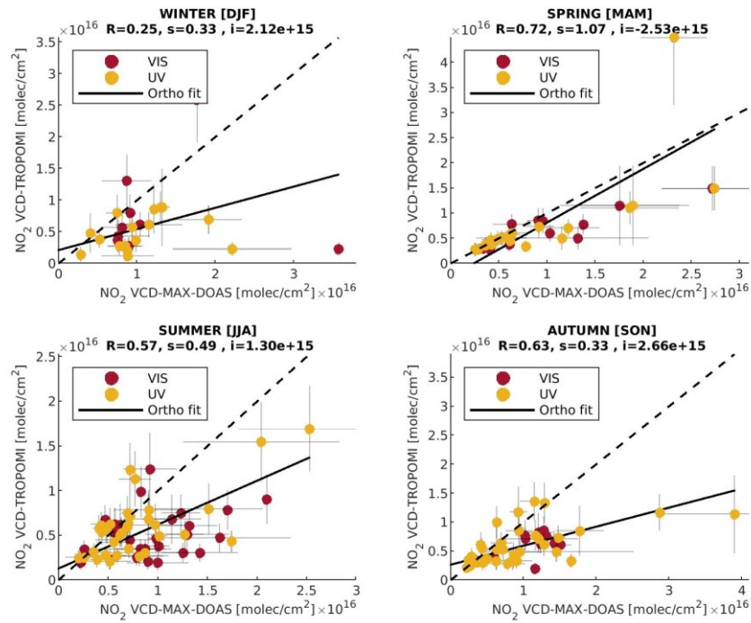
Figure 13: Seasonal scatter plots between the tropospheric \text{NO}_2 columns derived by UV and Vis MAX-DOAS observations (yellow and red circles, respectively) in the main azimuthal direction and the closest TROPOMI pixel with respect to the measurement site. The slope is estimated by using orthogonal regression analysis. The error bars are the same as in Figure 11.
