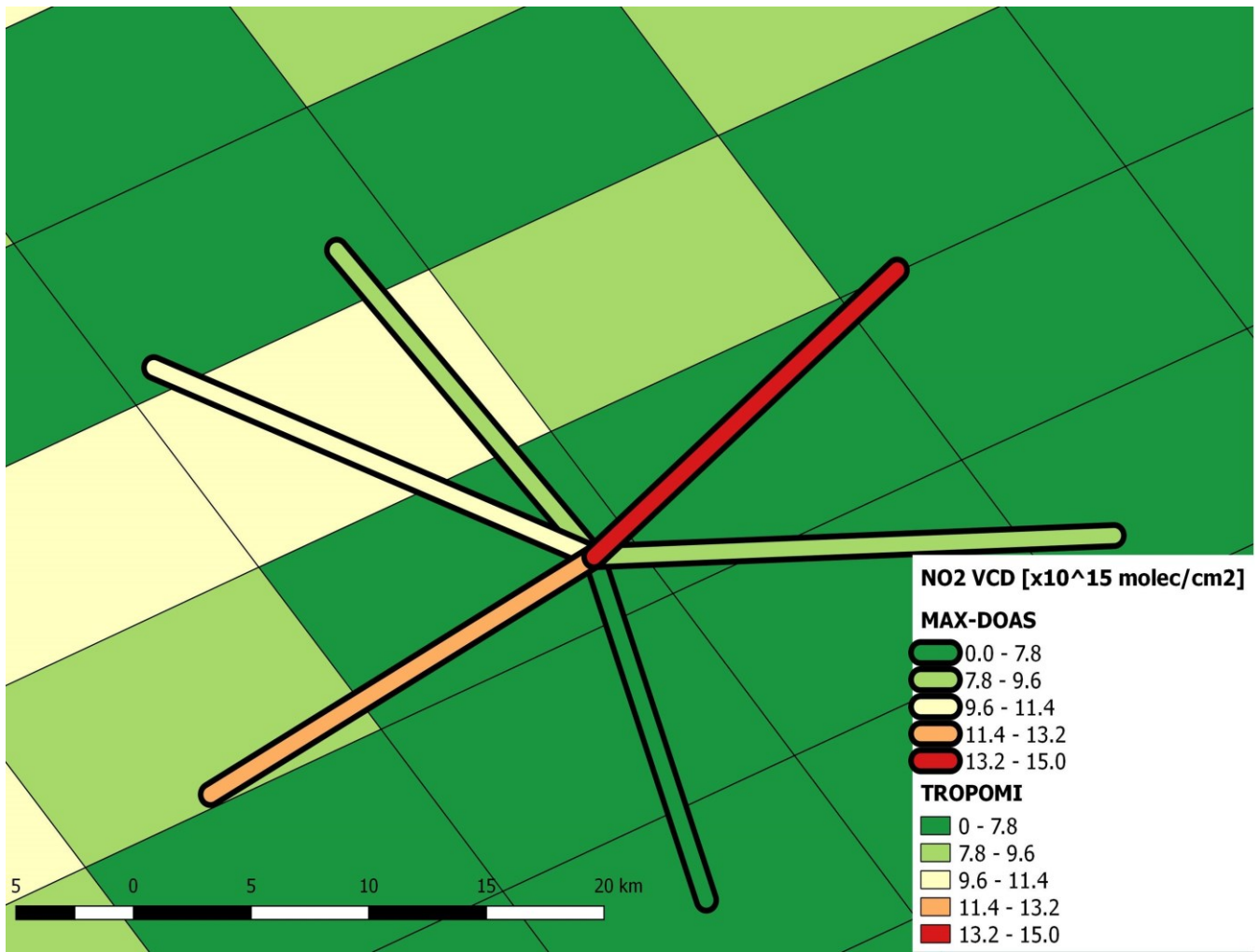
Figure 7: Tropospheric NO 2 columns derived from the TROPOMI (pixel size equal to 7 x 3.5 km 2 ) and the MAX-DOAS instrument on 06 June 2018 near the measurement site of Uccle.
