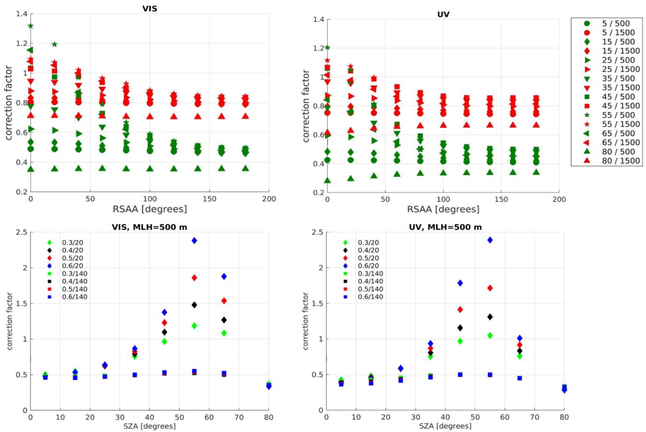
Figure 2: Upper panels correspond to the correction factors as a function of RSAA for two different MLH values (in every RSAA and MLH values, the different data points correspond to different SZA values) in the Vis and UV wavelength ranges. The first value in the symbols list corresponds to the SZA and the second to the MLH. Lower panels show the correction factors as a function of SZA for different AOD scenarios and RSAA values in the Vis and UV ranges for a MLH set to 500 m. The first value in the symbols list corresponds to the AOD and the second to the RSAA.
