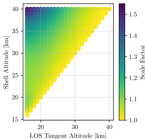
Figure 4. Scale factor matrix for a sunset occultation at the equator in March, simulated with PRATMO.
