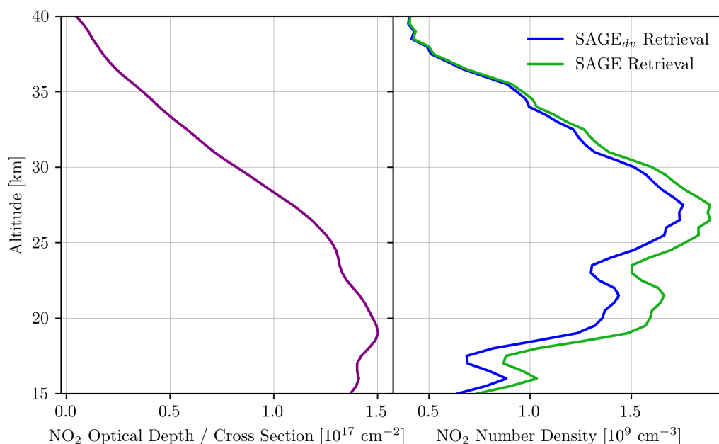
Figure 6. Optical depth and NO 2 number density for both the diurnally varying and SAGE v5.1 retrievals. Calculated for SAGE III/ISS event 967110.
