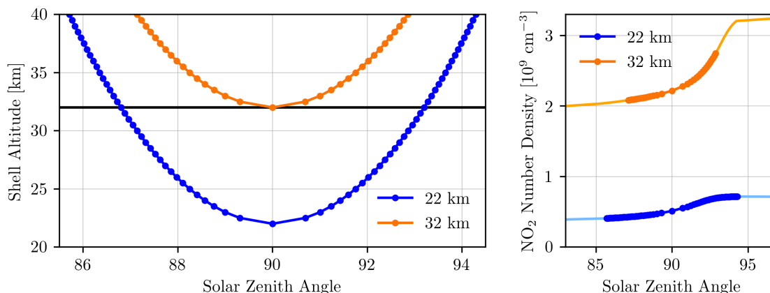
Figure 3. Left: Change in SZA with shell altitude along two lines of sight for a simulated sunset occultation. Right: Change in NO 2 at tangent altitudes of 22 km and 32 km for the same simulated sunset occultation. The dark, dotted lines correspond to the lines of sight from the left panel.
