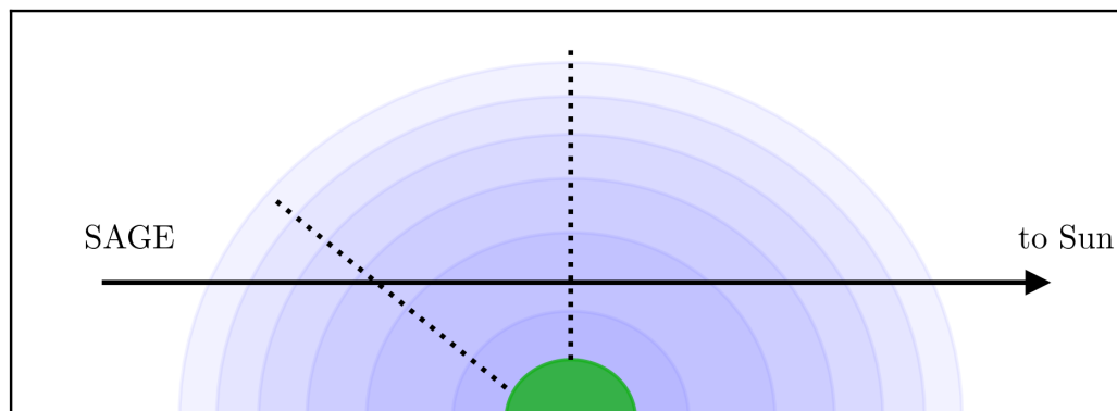
Figure 2. Geometry of a SAGE III occultation. The green semi-circle represents the Earth, and the blue semi-circles represent layers of the atmosphere. The angle between the dashed line and solid line is the solar zenith angle at a given location.
