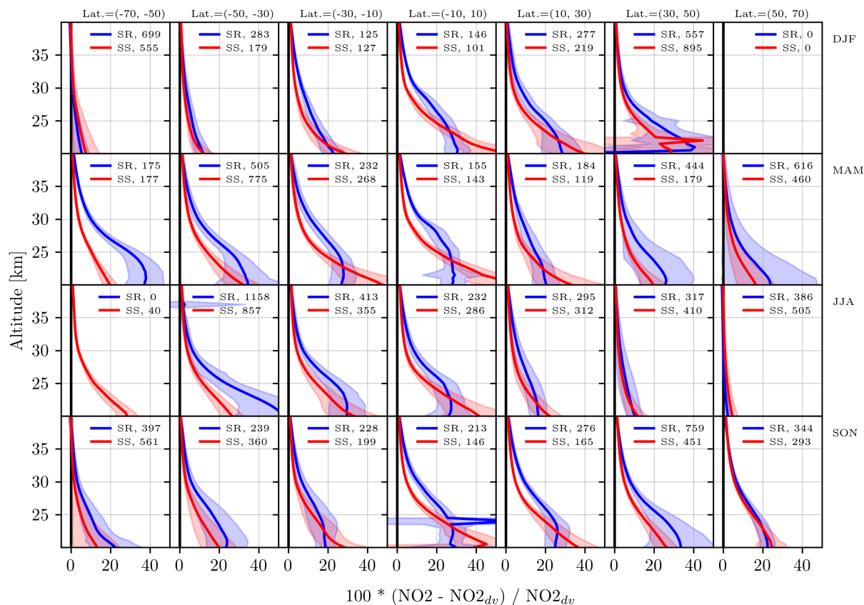
Figure 7. Mean difference between the SAGE v5.1 and diurnally varying (dv) retrievals for SAGE III/ISS sunset and sunrise \text{NO}_2 . The error bars are the standard deviation.
