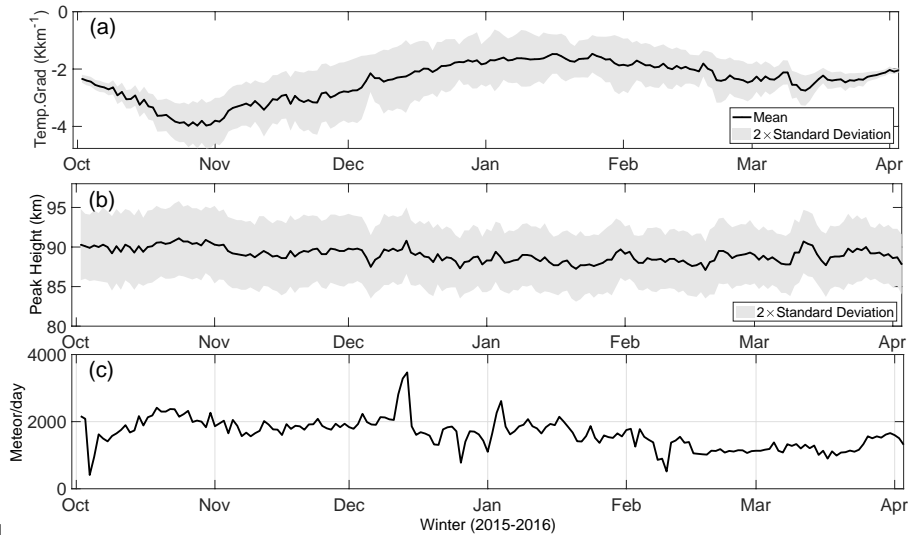
Figure 2. (a) Temperature gradient model derived from MSIS90. (b) Peak meteor heights for the data used in this work, and (c) the daily meteor detection for zenith angle less than 60^\circ – 50^\circ and velocity in the range \pm 100 m/s.
