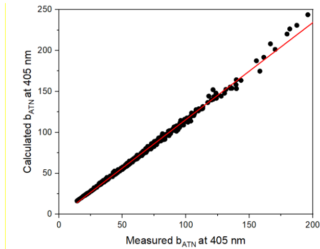
Figure S2. Measured b_{ATN} at 405 nm compared with b_{ATN} fitted from Eq. (3) using a two-component model.
