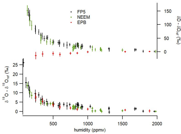
344 Figure 5: Influence of humidity on the isotopic composition ( \delta^{18}O and \delta D ) of the vapor obtained with the 345 LHLG with 3 water lab-standards. The error bars are calculated as the standard deviation ( 1\sigma ) over the 346 generated values by the L2130-i instrument during 10 minutes at 1 second resolution (i.e. without any pre- 347 averaging of the raw dataseries). The \delta^{18}O_{ref} and \delta D_{ref} are the values of the injected water standards at
