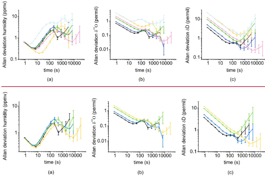
Figure 3: Allan deviation over 4 hours for different humidity levels (black 1,080 ppmv; dark blue 770 ppmv; green 400 ppmv; pink/yellow 320 ppmv; yellow and light blue 170 ppmv) for humidity (a), \delta^{18}\text{O} (b) and \delta\text{D} (c).
