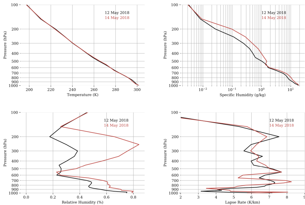
Fig. 1. MERRA-2 Reanalysis
