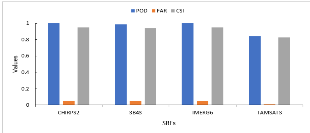
Figure 6. Categorical indices of the four SREs for the DRB.
