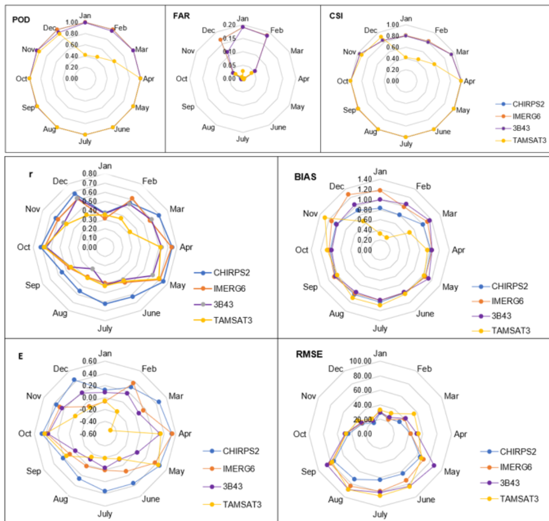
Figure 7. Seasonal statistical evaluation result comparison of each SREs for the DRB.
