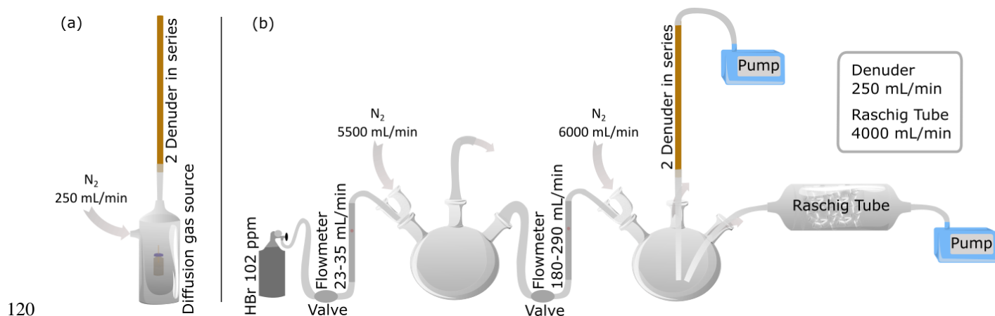
Figure 1: Experimental sampling setups in the laboratory. (a) Denuders were connected to a diffusion test gas source with PTFE tubes. The test gas source was heated to 50°C. Entering nitrogen was thermostated before it reached the diffusion source. (b) Experimental Setup for comparison of denuder and Raschig Tube technique for HBr determination.
