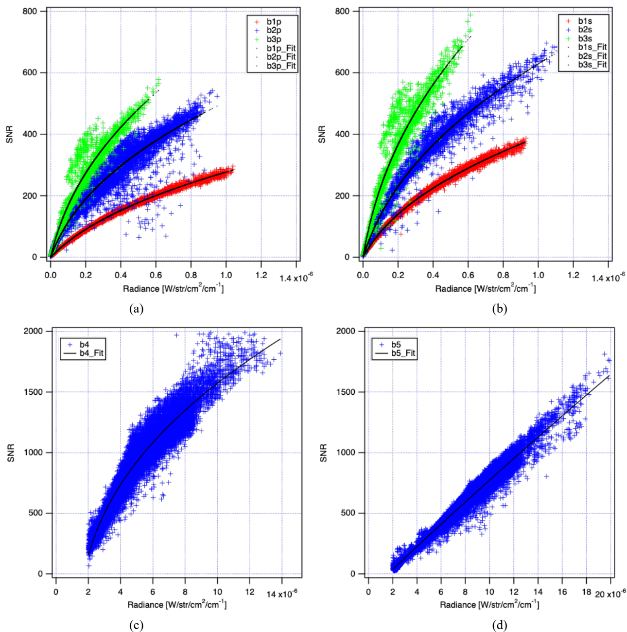
Figure 5. Signal to noise calculated from on-orbit data: (a) p-polarization bands for band 1,2,3, (b) s-polarization band for band 1,2,3, (c) band 4, and (d) band 5. Black dots show the model lines.
