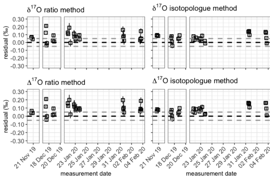
Figure 9. Quality control gas \delta^{17}O (upper panels) and \Delta^{17}O (lower panels) measurement averages for the three measurement periods for both the RM (left) and the IM (right). The averages are indicated by the black dotted line and the grey dotted line show the 0.05‰ range around the average. The error bars show the standard error of the measurements.
