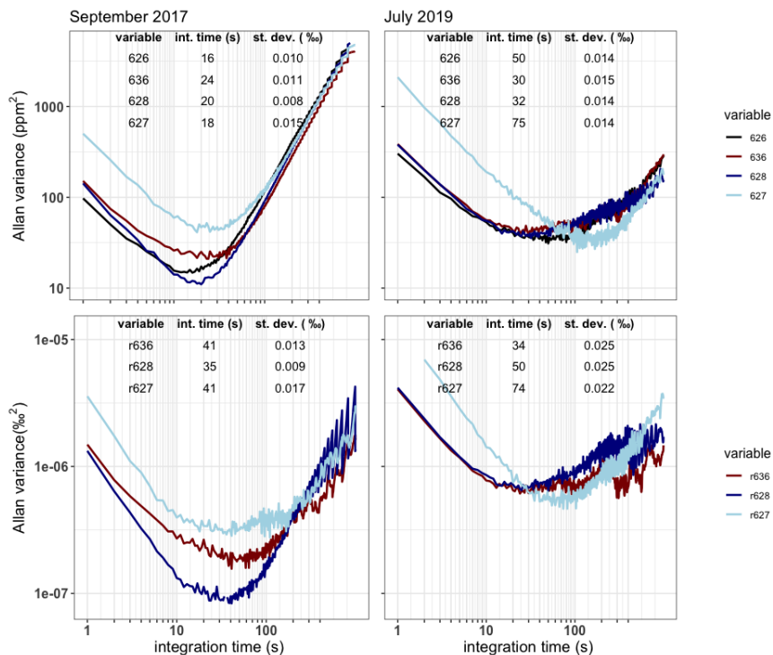
Figure 4. The Allan variance as a function of the integration time in seconds for a single gas measurement plotted for both the measured isotopologue abundance (top) and the isotope ratios (bottom) at September 2017 (left) and July 2019 (right). The best achieved precisions and corresponding integration times are shown as a table in the plots.
