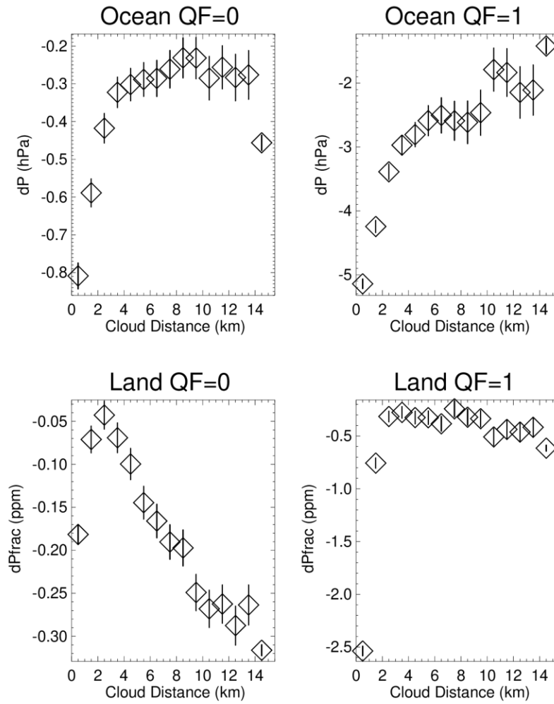
Figure 8. Averages of dPscO2 over the ocean and dPfrac over land as a function of the nearest cloud distance metric for QF=0 and QF=1 Version 10 data. 95 % ( 2\sigma ) confidence limits of the averages are represented by the vertical line associated with each average.
