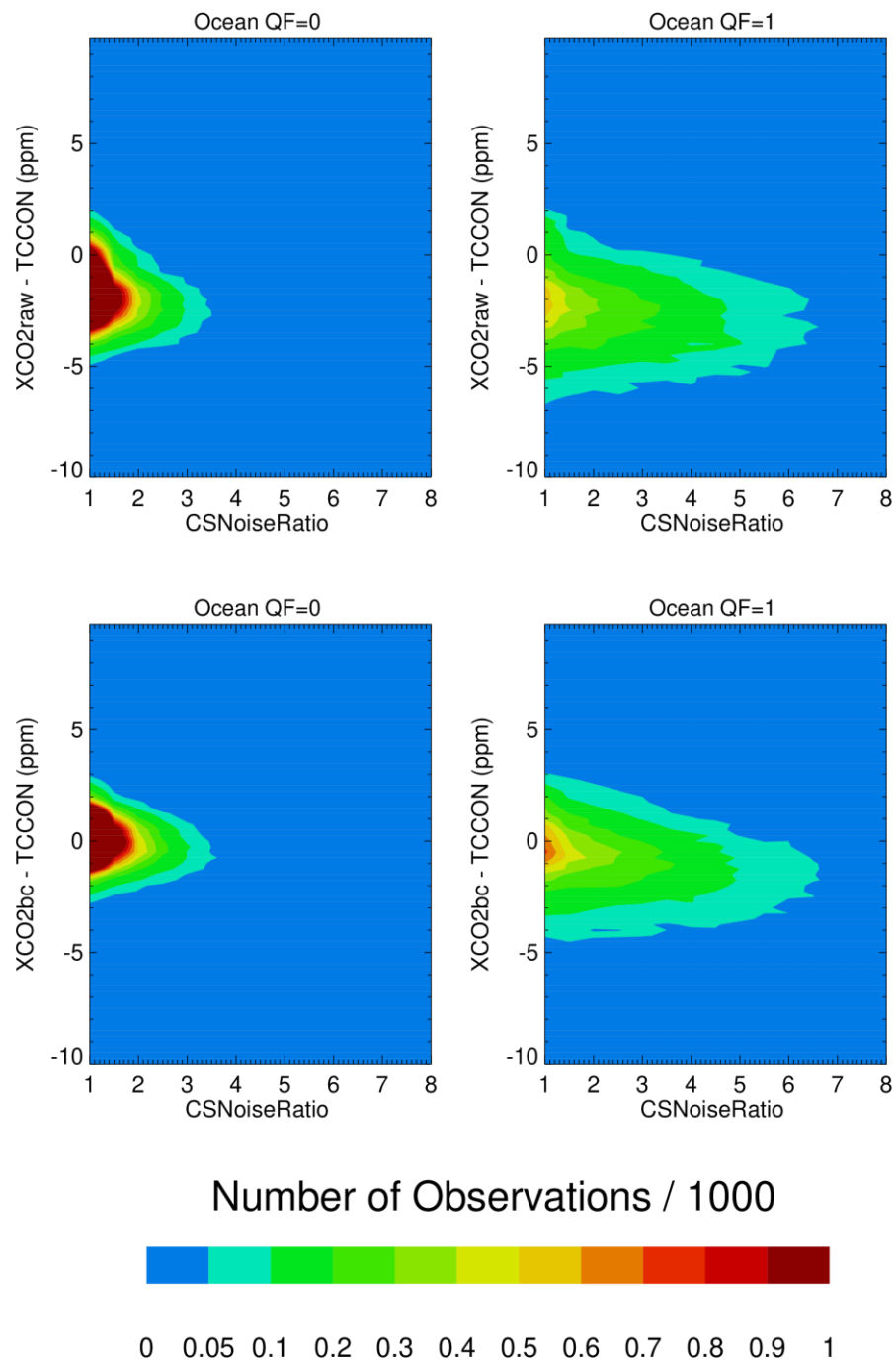
1510 Figure 5. Contour maps of XCO 2 – TCCON over the ocean as a function of the CSNoiseRatio metric for QF=0 and QF=1 XCO 2 raw and XCO 2 bc Version 10 data. The QF=1 XCO 2 bc data over the ocean has a noticeable asymmetry along CSNoiseRatio vertical lines.
