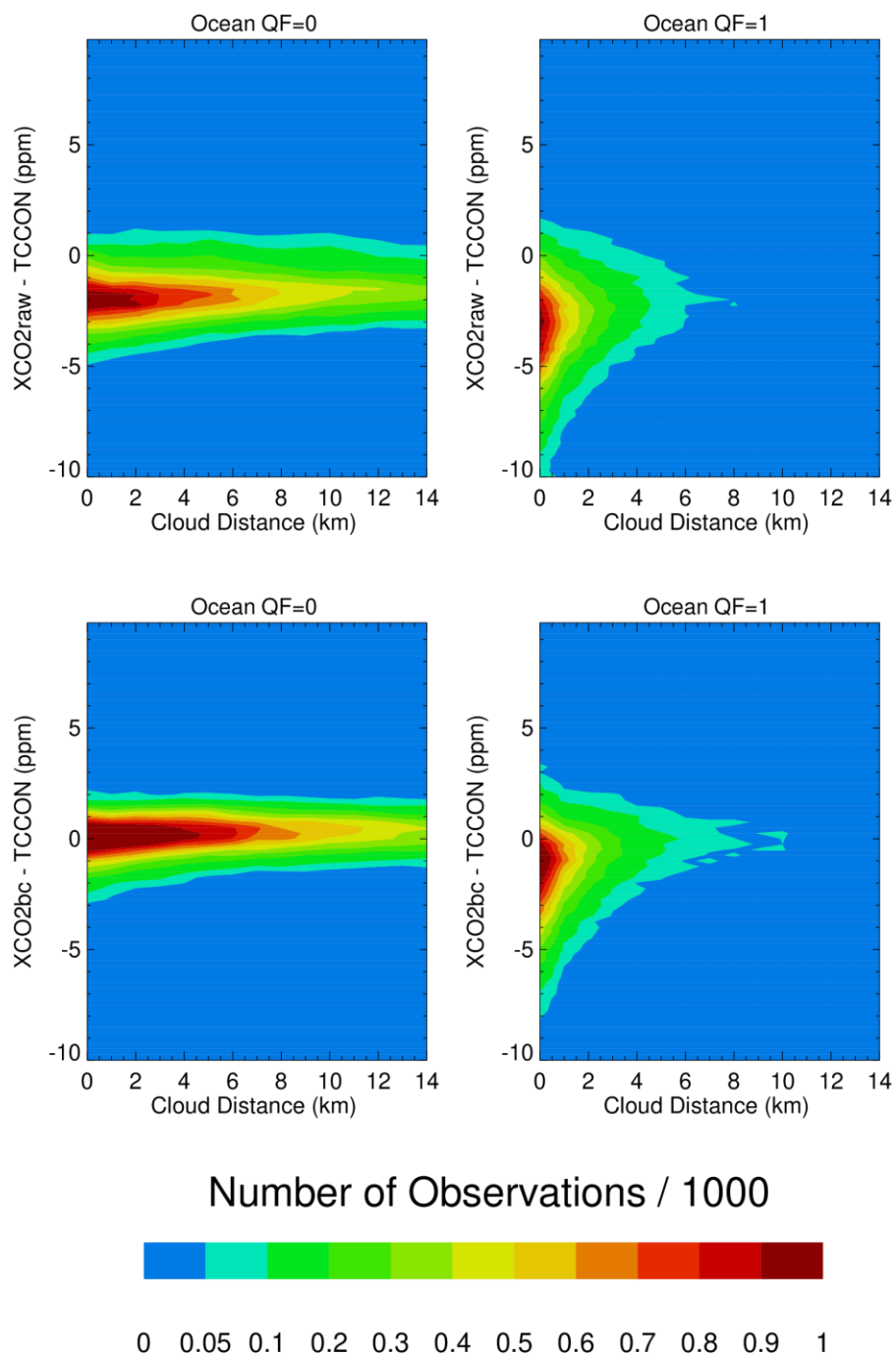
1505 Figure 4. Contour maps of XCO 2 – TCCON over the ocean as a function of the nearest cloud distance for QF=0 and QF=1 XCO2raw and XCO2bc Version 10 data. There is a very noticeable asymmetry (a tail of negative XCO2bc-TCCON) along vertical lines of nearest cloud distance in the QF=1 data, especially for small nearest cloud distance.
