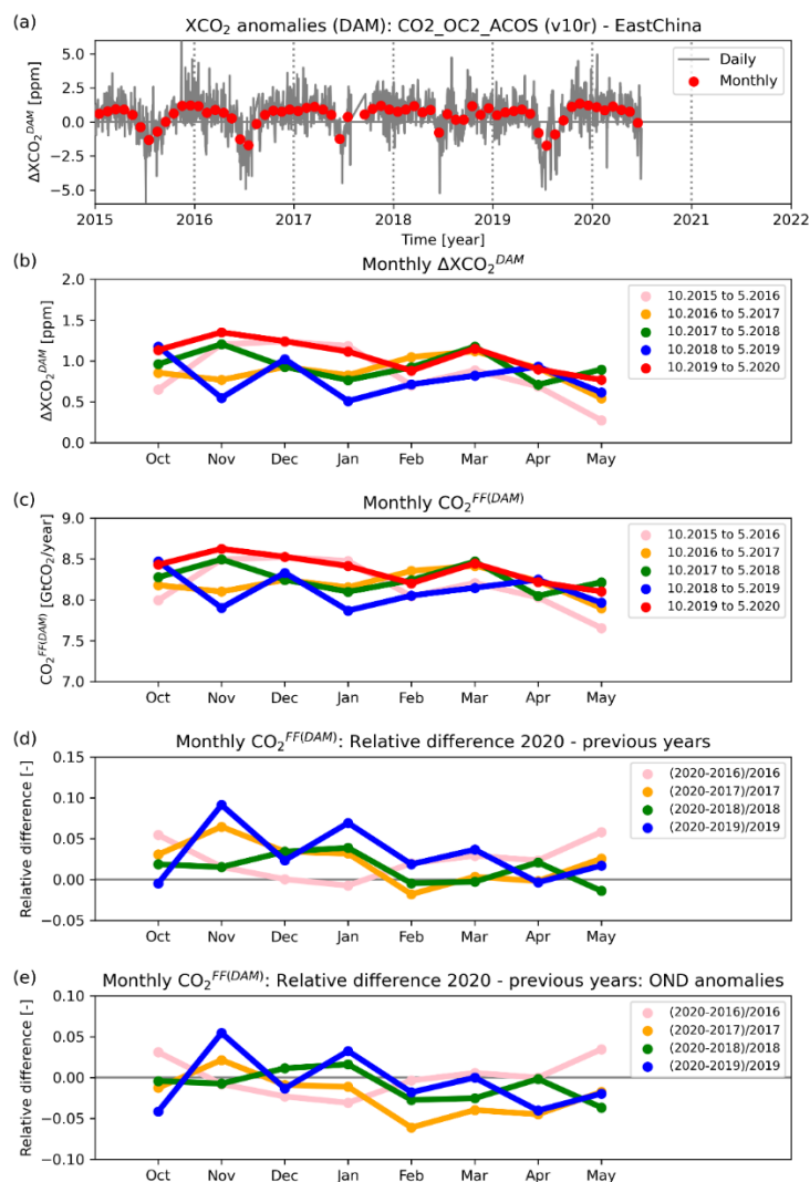
Figure 7: DAM analysis of the OCO-2 ACOS version 10r XCO 2 product (CO 2 _OC2_ACOS) for the region East China from January 2015 to May 2020. (a) The thin grey line shows the daily DAM XCO 2 anomalies, i.e., daily \Delta\text{XCO}_2^{\text{DAM}} . The red dots are the corresponding monthly values, which are also shown in (b) for different October – May periods. (c) As (b) but for \text{CO}_2^{\text{FF(DAM)}} , i.e., for the estimated East China monthly FF emissions (see main text). The data for October 2019 – May 2020 (10.2019-5.2020) are shown in red (see annotation for other periods). (d) Relative \text{CO}_2^{\text{FF(DAM)}} differences for different periods. In blue, for example, the differences correspond to the period 10.2019-5.2020 (shown in red in panel (c)) minus 10.2018-5.2019 (shown in blue in (c)). (e) As (d) but after the October to December mean value (“OND anomalies”). The following parameters have been used to generate this figure: Minimum number of observations/day: 30, minimum number of days/month: 5.
