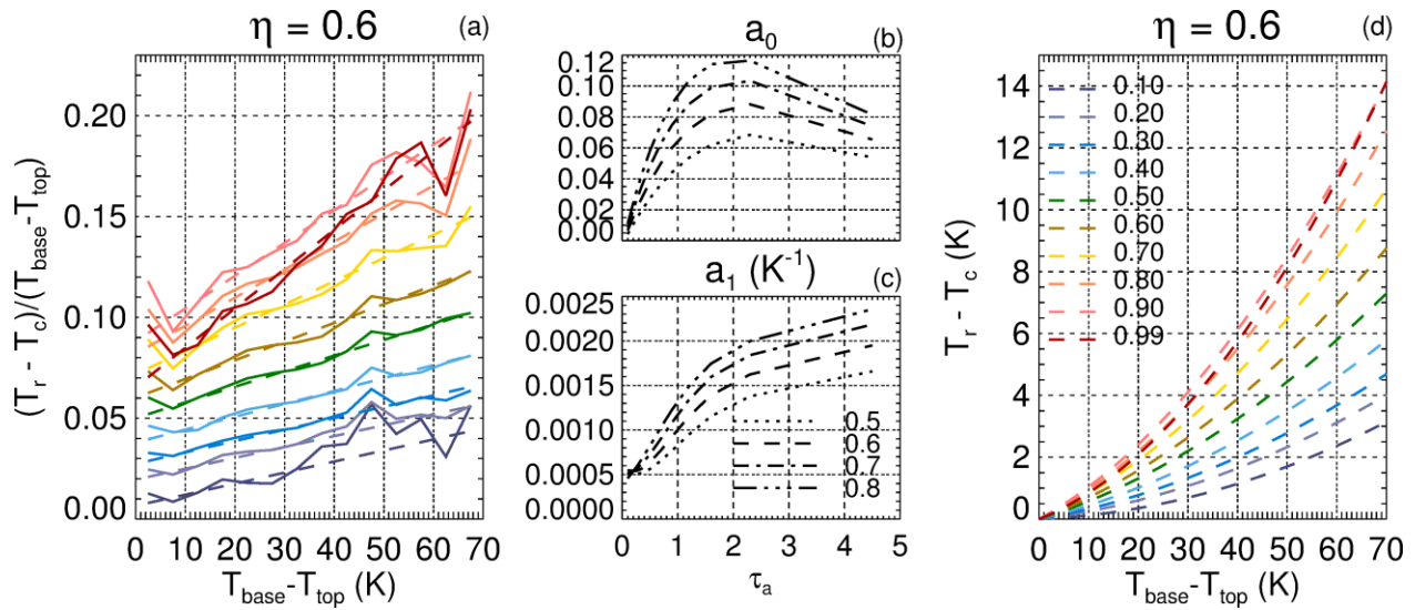
390 Figure 6: V4 correction functions of ice cloud radiative temperature: (a) (T_r - T_c)/(T_{base} - T_{top}) vs T_{base} - T_{top} for effective emissivities between 0.1 and 0.99 and \eta = 0.6 . The solid lines are median values from statistical analyses and the dashed lines are regression lines; (b) intercept and (c) slope of the regression lines vs. \tau_{a,12} for \eta between 0.5 and 0.8; (d) resulting V4 corrections T_r - T_c vs. T_{base} - T_{top} for effective emissivities between 0.1 and 0.99 and \eta = 0.6 . Channel 12.05 \mu\text{m} .
