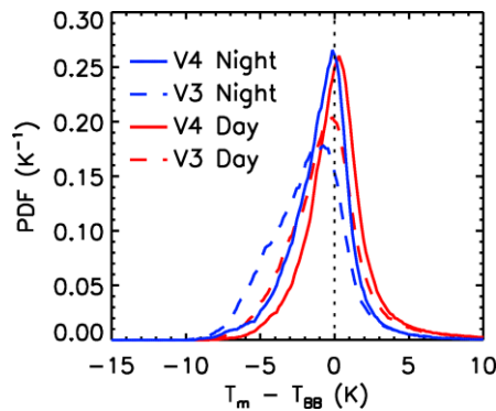
450 Figure 8: Probability density functions of the V4 (solid) and V3 (dashed) nighttime (blue) and daytime (red) differences between measured brightness temperature and computed blackbody brightness temperatures over oceans between 60^\circ S and 60^\circ N in January 2008 for the IIR 12.05 \mu\text{m} channel.
