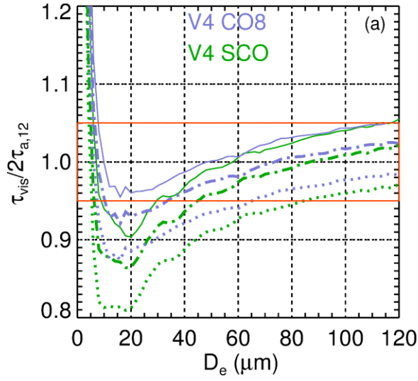
Figure 13: Comparison of (a) \tau_{vis}/2\tau_{a,12} and (b) \tau_{vis}/(\tau_{a,12} + \tau_{a,10}) vs. D_e for the V4 CO8 (purple) and SCO (green) ice models. Simulations with no scattering (solid line), and with scattering using \tau_{a,12} = 0.25 (dashed dotted lines) and \tau_{a,12} = 3 (dotted lines). The red rectangle identifies the domain within \pm 5\% limits.
