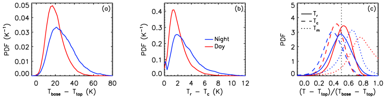
430 Figure 7: Nighttime (blue) and daytime (red) probability density functions in V4 opaque ice clouds of (a) apparent thermal thickness T_{\text{base}} - T_{\text{top}} , (b) T_r - T_c V4 correction, and (c) (T - T_{\text{top}})/(T_{\text{base}} - T_{\text{top}}) for T = T_r (solid lines), T = T_c (dashed lines), and T = T_m (dotted lines) over oceans between 60^\circ S and 60^\circ N in January 2008. Channel 12.05 \mu\text{m} .
