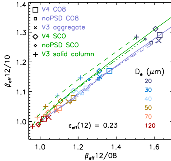
525 Figure 11: The V4 ice LUT values (solid lines; CO8: large squares; SCO: large diamonds) are compared with the V4 LUT values with 530 no PSD (dashed dotted lines and small symbols) and the V3 ice LUT values (dashed lines; cross: aggregate; plus signs: solid column), for 6 values of D_e between 20 and 120 \mu\text{m} and using \epsilon_{\text{eff},12} = 0.23 for the 3 configurations.
