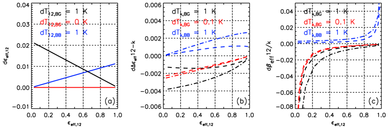
200 Figure 1: (a) Sensitivity of \epsilon_{\text{eff},12} to systematic errors dT_{12,BG} = +1 K (black), dT_{12,BG} = 0 K (red, no error), and dT_{12,BB} = +1 K (blue); (b) sensitivity of \Delta\epsilon_{\text{eff}12-k} (dashed lines) and \Delta\epsilon_{\text{eff}12-08} (dashed dotted lines) to systematic errors dT_{12,BG} = dT_{10,BG} = dT_{08,BG} = 1 K (black), dT_{12,BG} = 0 and dT_{10,BG} = dT_{08,BG} = 0.1 K (red), and dT_{12,BB} = dT_{10,BB} = dT_{08,BB} = 1 K (blue); (c): same as (b), but for \beta_{\text{eff}12/10} (dashed lines) and \beta_{\text{eff}12/08} (dashed dotted lines). Simulations using T_{BG} = 285 K and T_{BB} = 225 K, and \beta_{\text{eff}12/k} = 1.1 .
