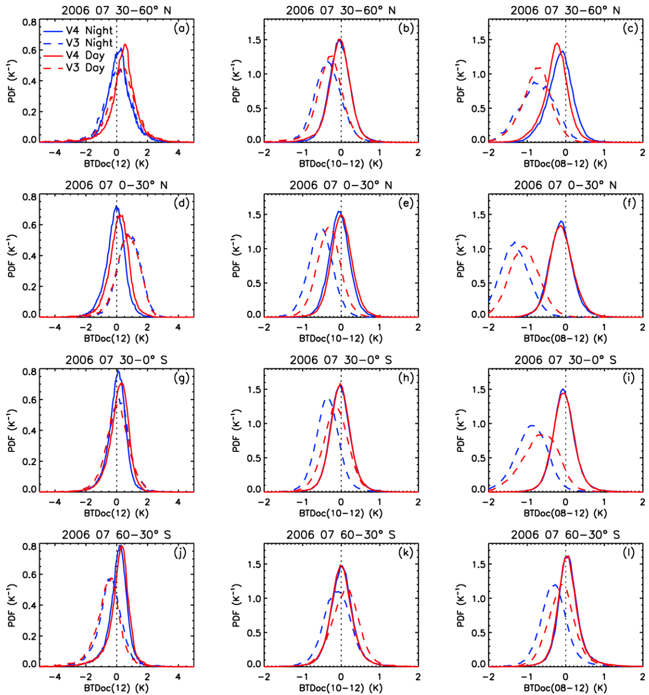
Figure 4: Same as Fig. 3 but for July 2006.
