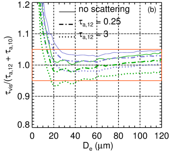
Figure 13: Comparison of (a) \tau_{vis}/2\tau_{a,12} and (b) \tau_{vis}/(\tau_{a,12} + \tau_{a,10}) vs. D_e for the V4 CO8 (purple) and SCO (green) ice models. Simulations with no scattering (solid line), and with scattering using \tau_{a,12} = 0.25 (dashed dotted lines) and \tau_{a,12} = 3 (dotted lines). The red rectangle identifies the domain within \pm 5\% limits.
