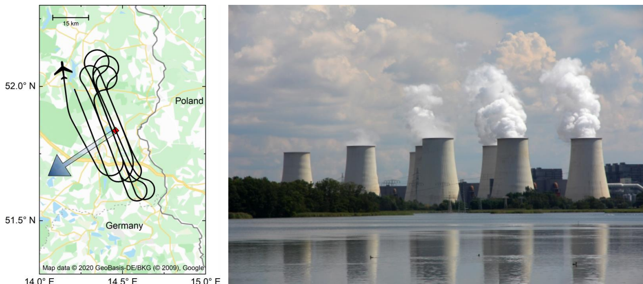
Figure 4: Flight track of HALO in the vicinity of the coal-fired power plant Jänschwalde. The black lines on the left depict the flight track of HALO between 10:24 and 11:36 on the 23 May 2018. The red square marks the position of the power plant Jänschwalde. The arrow shows the mean wind direction during the observation period. The right picture shows the nine cooling towers facing southwest. There the exhaust is released. The towers have a height of 120 m and horizontal spacing of 250 m and 50 m.
