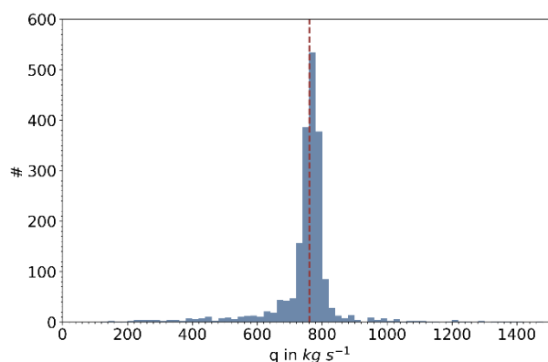
Figure 7: Histogram of virtually retrieved emission rates. The histogram shows a slightly skewed distribution towards smaller emission rates than the input emission rate (red dashed line). It depicts all 1980 emission rates retrieved over 66 simulated hours between 12 UTC on 21 May and 6 UTC on 24 May.
