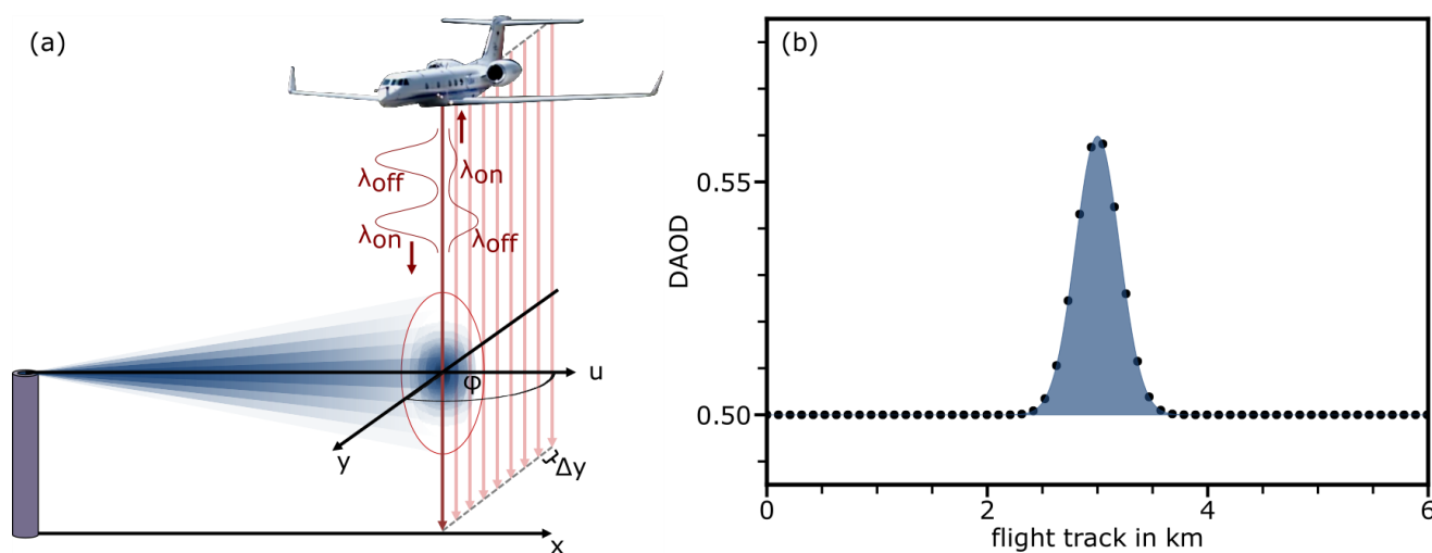
Figure 2: Crossing an exhaust plume illustrated by the example of CHARM-F carried on the aircraft HALO. (a) Two laser pulses are emitted towards the earth with short delay. The laser pulse with the wavelength \lambda_{\text{on}} is on the absorption wavelength of \text{CO}_2 , the laser pulse with the wavelength \lambda_{\text{off}} is not. By comparing the backscattered intensities, the DAOD can be calculated (see Sect. 2.1). An ideal exhaust plume of a point source has a Gaussian-shaped mean concentration distribution both horizontally and vertically. (b) A perpendicular crossing of the plume yields a Gaussian-shaped DAOD dataset.
