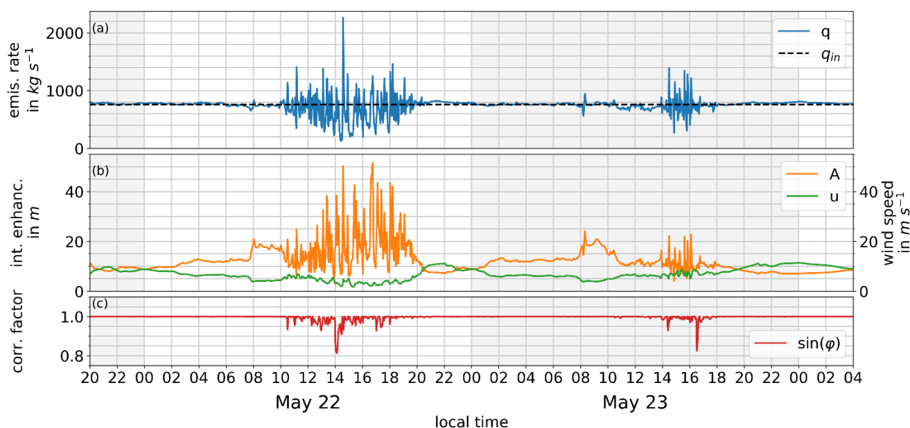
Figure 8: Virtual overflight results in the course of the day. Midday turbulence causes a deviation of the retrieved emission rates q from the input emission rate q_{in} in (a). This can correspondingly be seen in the integrated enhancement A in (b), while the wind speed u shows comparatively small variations. It is during the midday turbulence, that the virtual flight track is not exactly perpendicular to the instantaneous wind direction at the plume crossing, which is shown in the correction factor \sin(\varphi) in (c). In the night hours, as well as the morning the retrieved emission rates agree very well with the input emission rate q_{in} .
