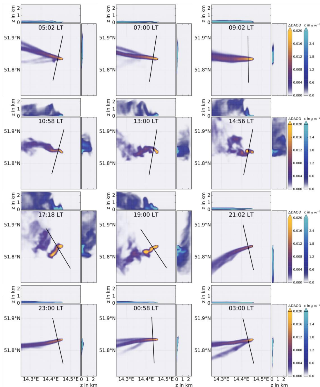
Figure A2: Exemplary snapshots of simulated plume and virtual flight track. The daily solar irradiation causes a deep, convective boundary layer with turbulent plume dispersion within. In the nocturnal absence of solar irradiation, the boundary layer shrinks, leading to narrow, homogeneous plume dispersion, within a laminar flow. Every two minutes a virtual measurement is performed yielding 60 measurements within a time frame of 2 hours. One representative snapshot within the two-hour time frame is shown.
