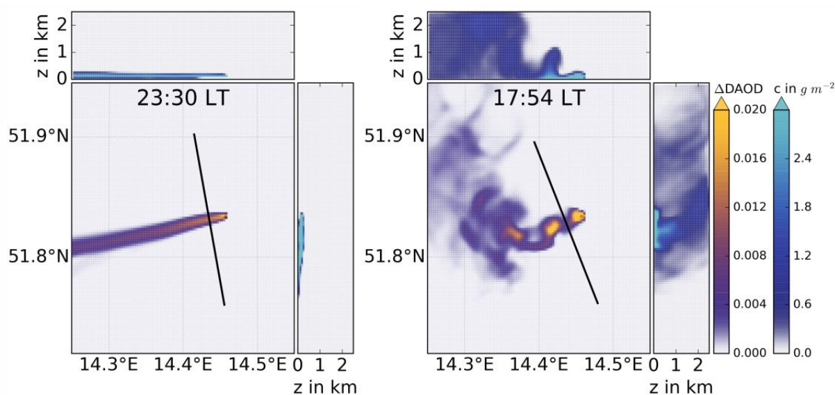
Figure 6: Exemplary snapshots of simulated exhaust plume. The flight track of the virtual plume overflight is shown as a black line. The first colorbar represents the DAOD enhancement and refers to the respective middle panel, which shows the horizontal dispersion of the plume. The second colorbar represents the mass per area and refers to the top and right panels, which show the vertical dispersion. For the DAOD, enhancement values beneath 0.008 cannot be distinguished from noise and are display blue. Values higher than 0.01 exceed the noise and can be identified as plume enhancement in a real measurement. A \Delta DAOD value of 0.02 corresponds to an enhancement of 4 % with respect to a background of 0.5 (cf. Fig. 3). The color maps follow the guidelines for a perception-based color map presented by Stauffer et al. (2015).
