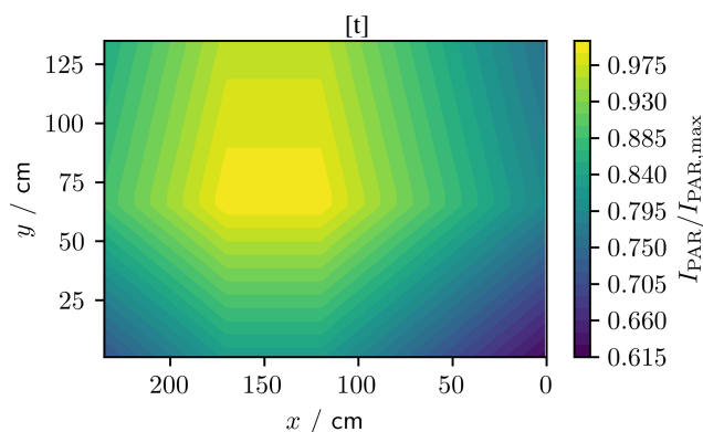
Figure 8. Normalised PAR ( \lambda = 400 to 700 nm) irradiance across the footprint of the tank at 1 m height. The (0, 0) cm coordinate corresponds to the pink asterisk in Fig. 3.
