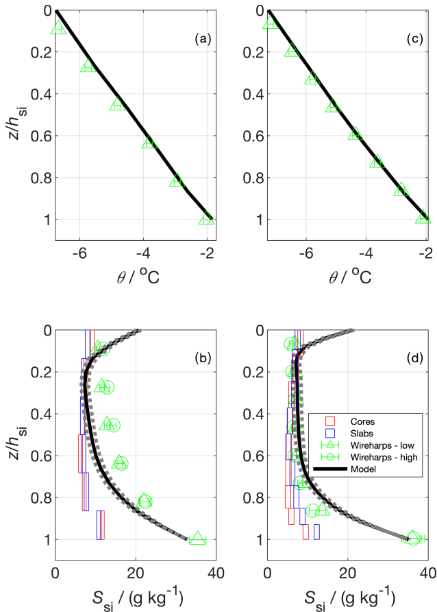
Figure 11. Vertical temperature (a and c) and bulk salinity profiles (b and d) for two experimental runs. In (a) and (c) the model temperature shows the model forcing, which was produced using measured temperature profiles; panels (b) and (d) show salinity estimated from cores, slabs (Cottier et al., 1999), wireharp (Notz et al., 2005), and a gravity drainage model. The horizontal box length shows the median 1\sigma standard deviation \sigma_{\text{TSS}} from repeat measurements at a given depth (cores and slabs), and the vertical box length shows the depth covered by the sample layer. Wireharp errors were calculated using methodology presented in Zeigermann (2018). The model used the Griewank and Notz (2013) gravity drainage parameterisation with tuning parameters taken from Griewank and Notz (2015). The solid line represents their best estimate tuning parameter set. The dotted bounds on the model show output using two other plausible sets of tuning parameters presented in Griewank and Notz (2015).
