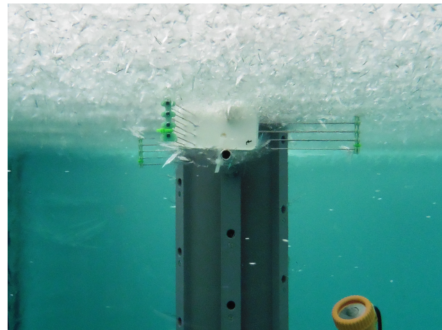
Figure 5. A view of a supercooled ocean. Frazil ice crystals are floating upwards in the water column (white flecks) and have nucleated on wireharps well ahead of the advancing sea-ice-ocean interface.
