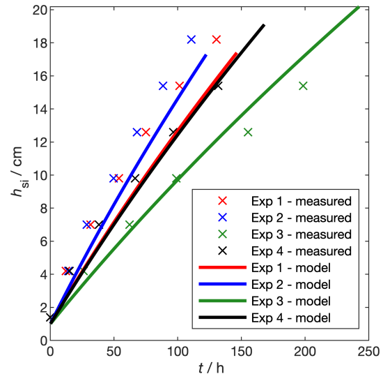
Figure 12. Thickness measured from temperature profiles during the experiments presented in Sect. 3.1.3 and modelled using Eq. (16).
