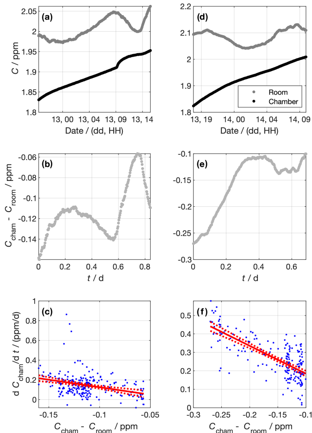
Figure 6. Data from experiments to determine the chamber air exchange rate. Panels (a) to (c) and (d) to (f) show data from the first and second experiments, respectively. The top panels (a) and (d) show the measured \text{CH}_4 concentrations in the chamber and the lab outside. Panels (b) and (e) show the concentration difference between the chamber and the lab outside. Panels (c) and (f) show the linear regressions constructed using Eq. (5). Blue dots show individual data points. The red lines show the best fit and 95 % confidence intervals of the linear regression of \frac{dC_{\text{cham}}}{dt} against C_{\text{cham}} - C_{\text{room}} . The gradient of the linear regression corresponds to the air exchange rate coefficient, -k . For the first experiment, k = (1.5 \pm 0.3) \text{ d}^{-1} , and for the second experiment, k = (1.5 \pm 0.1) \text{ d}^{-1} .
