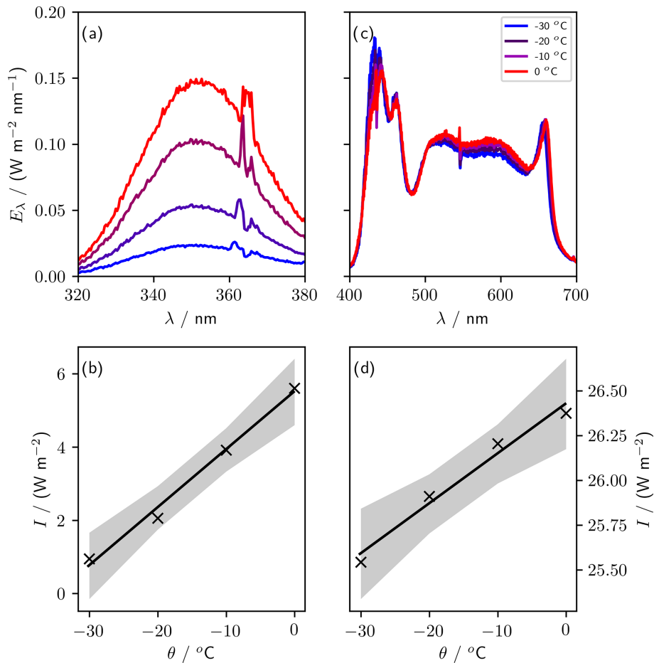
Figure 9. Sensitivity of lights to variations in temperature. Panels (a) (UV) and (c) (PAR) show spectra taken at four temperatures between 0 and -30 °C. Panels (b) (UV, 320 to 380 nm) and (d) (PAR, 400 to 700 nm) show the irradiance, I (integrated spectral irradiance over the respective wavelength ranges), at each temperature, \theta . The gradient of the regression of I against \theta is (0.028 \pm 0.003) \text{ W m}^{-2} \text{ °C}^{-1} for PAR and (0.16 \pm 0.01) \text{ W m}^{-2} \text{ °C}^{-1} for UV.
