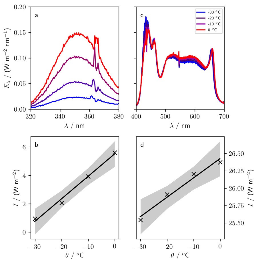
Figure 9. Sensitivity of lights to variations in temperature. Panels a (UV) and c (PAR) show spectra taken at four temperatures between 0^\circ\text{C} and -30^\circ\text{C} . Panels b (UV, 320 nm to 380 nm) and d (PAR, 400 nm to 700 nm) show the irradiance, I (integrated spectral irradiance over the respective wavelength ranges), at each temperature, \theta . The gradient of the regression of I against \theta is (0.028 \pm 0.003) \text{ W m}^{-2} \text{ }^\circ\text{C}^{-1} for PAR and (0.16 \pm 0.01) \text{ W m}^{-2} \text{ }^\circ\text{C}^{-1} for UV.
