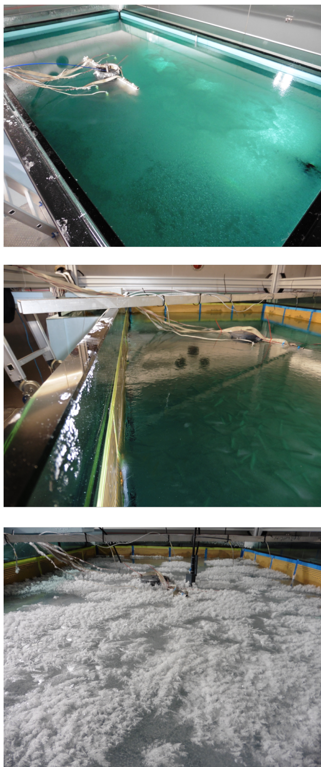
Figure 4. Grease ice (top) grown under pumping, nilas (middle) grown in quiescent conditions, and a frost flower field (bottom) grown in the RvG-ASIC.
