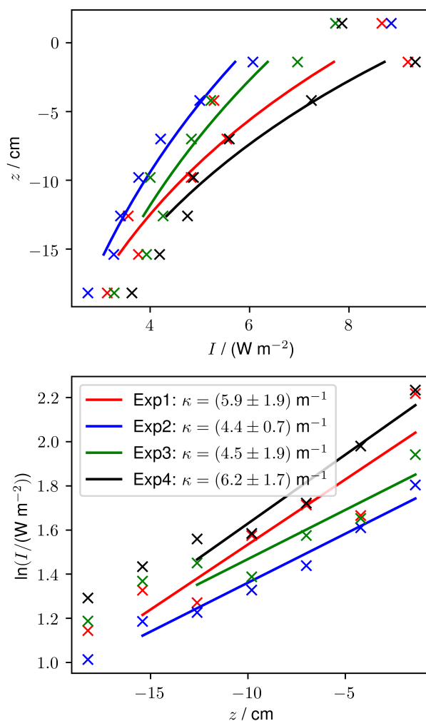
Figure 10. Irradiance profiles (a) and linear regressions of \ln(I / \text{W m}^{-2}) vs z (b) used to produce extinction coefficients (Equations 8 and 9) from the final profile of the freezing period. The legend in panel b gives the extinction coefficient for a given profile with one standard error.
