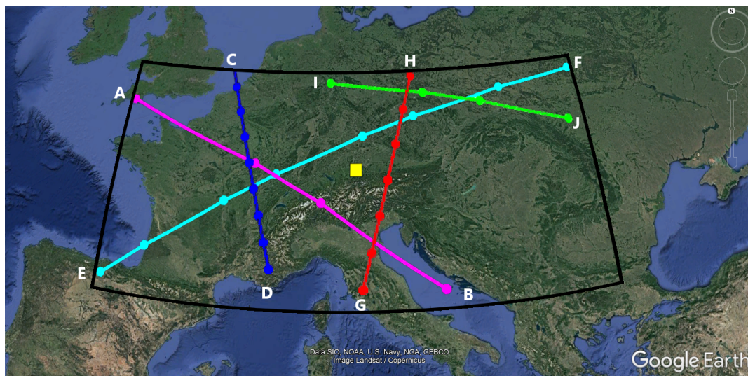
Figure 1. The area defined for coincident measurements during the HOPS campaign (42.8,-4.0) to (52.8,26.0). Meteorological Observatory Hohenpeißenberg is represented by the yellow square at (47.8,11.0) and the nearby München-Oberschleissheim radiosonde launches are located at (48.1,11.3). For the night beginning on the 29th of March 2019 the HOH lidar operated from 21:28-4:40 UTC; the MLS overpass (G-H, red) occurred at approximately 1:14 UTC on the 30th of March; the SABER overpasses occurred on the 29th of March at 22:45 UTC (E-F, cyan) and 23:30 UTC (A-B, magenta), and on the 30th March at 1:16 UTC (I-J, green); and the OMPS overpass (C-D, blue) occurred on the 30th of March at 11:50 UTC. (data: © Google Earth Pro, 2020)
