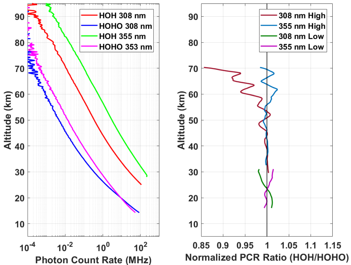
Figure 2. High gain signals for the HOH and HOHO lidars showing higher signal levels in the newly improved HOH lidar. Ratios of high and low gain signals for the HOH and HOHO lidars showing SNR improvement in received signal.
