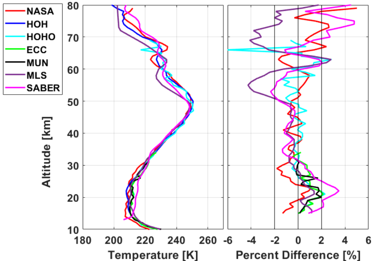
Figure 3. Temperature profiles measured by the NASA-STROZ (red), HOH (blue), and HOHO (cyan) lidars, locally launched ozonesonde (green), München meteorological radiosonde (black), and overpasses from MLS (violet) and SABER (magenta) on the night of 21 October 2018. Percent differences are with respect to the HOH lidar.
