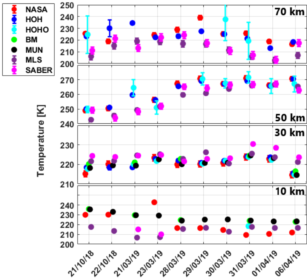
Figure 9. Time series of temperature measurements at smoothed using a 2 km boxcar average. Top panel contains temperatures at 70 km, second panel at 50 km, third panel at 30 km and the bottom panel at 10 km.
