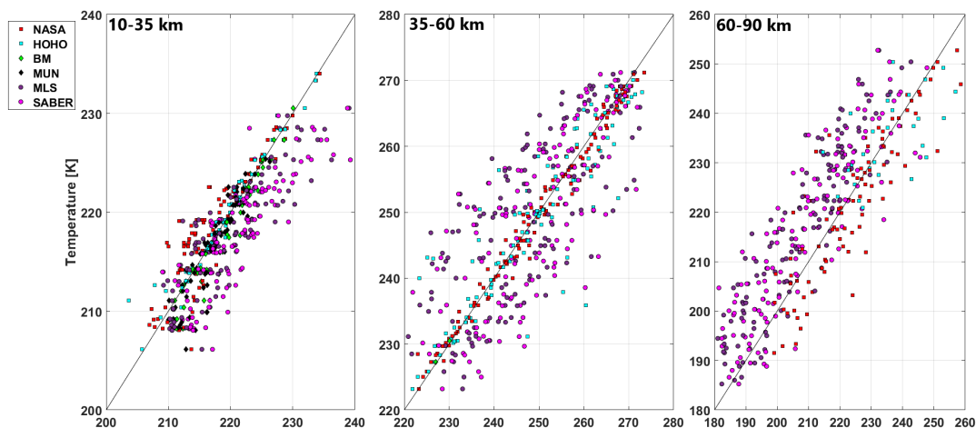
Figure 11. Scatter plots of temperature at 2 km resolution for the different instruments involved in the HOPS campaign with respect to the HOH lidar. (Left): 10 to 35 km; (Centre): 35 to 60 km; (Right): 60 to 90 km;
