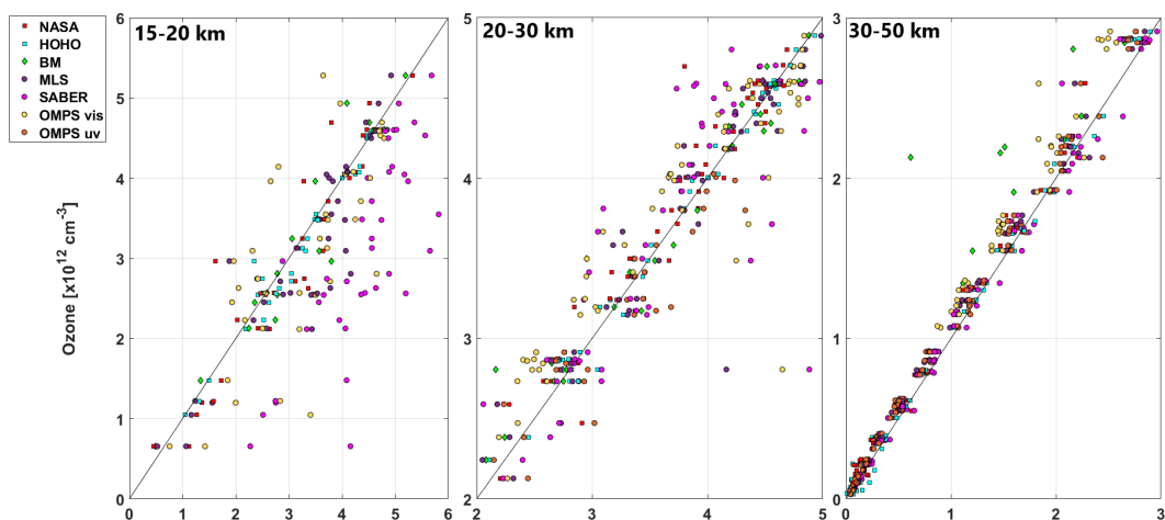
Figure 7. Ozone scatter plots, smoothed using a 2 km boxcar average, with respect to ozone number densities from the HOH lidar. (Left): 15 to 20 km; (Centre): 20 to 30 km; (Right): 30 to 50 km;
