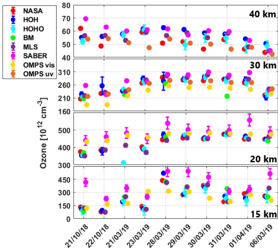
Figure 5. Time series of ozone measurements smoothed using a 2 km boxcar average. Top panel contains ozone densities at 40 km, second panel at 30 km, third panel at 20 km and the bottom panel at 15 km.
