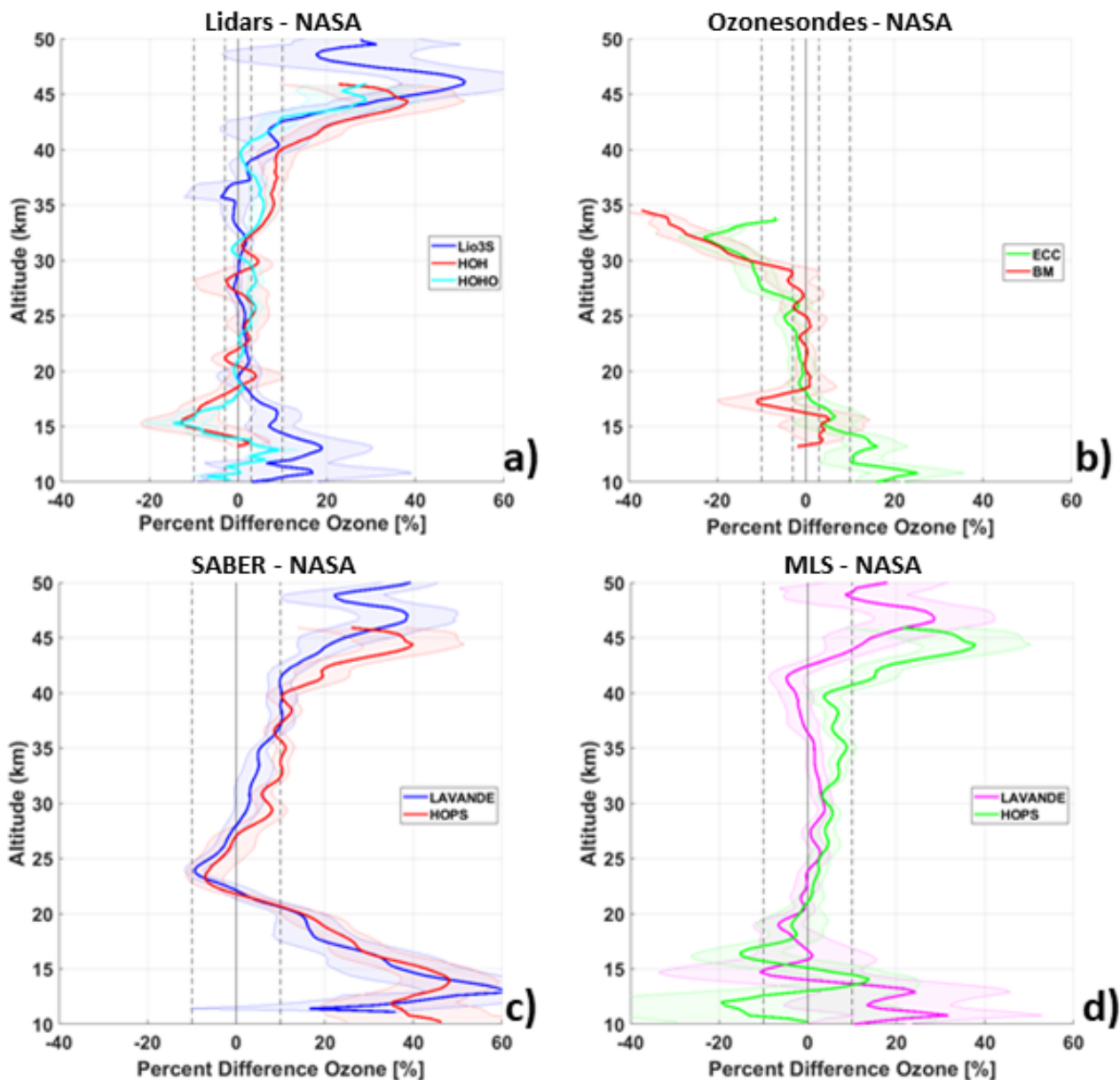
Figure 18. Cross-comparison of LAVANDE and HOPS ozone measurements for the NDACC lidars LiO 3 S, HOH, and HOHO; satellites MLS and SABER; and ozonesondes Brewer-Mast and ECC; with respect to the NASA-STROZ lidar.
