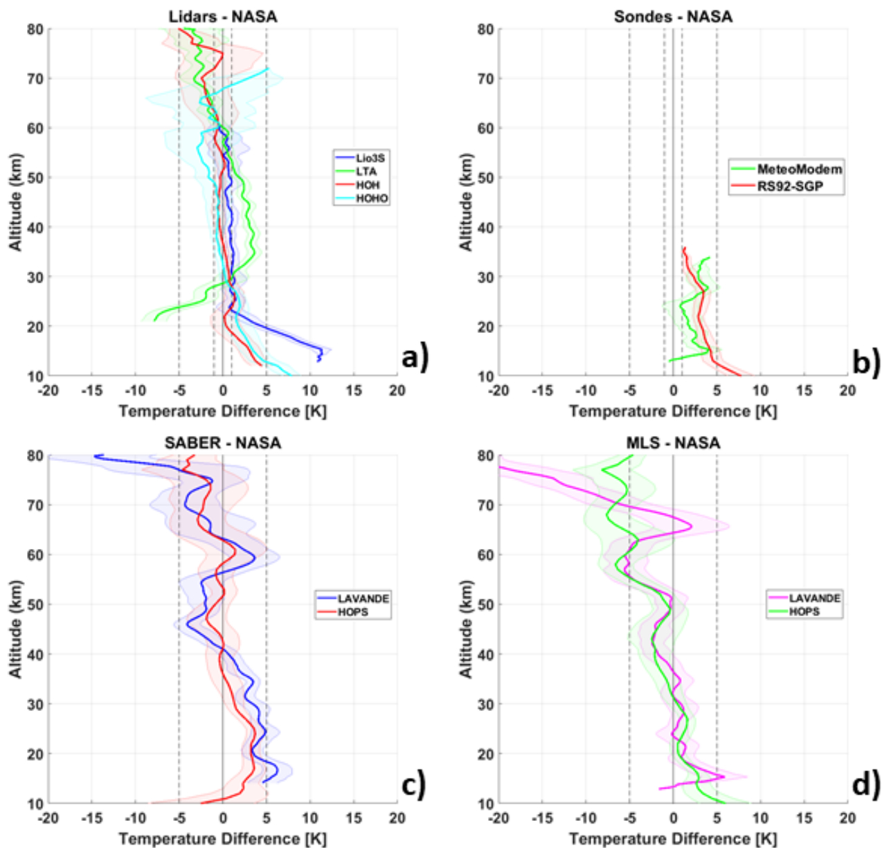
Figure 19. Cross-comparison of LAVANDE and HOPS temperature measurements for the NDACC lidars LiO3S, LTA, HOH, and HOHO; satellites MLS and SABER; and the radiosondes attached to the Brewer-Mast (RS92-SGP) and ECC (MeteoModem M10); with respect to the NASA-STROZ lidar.
