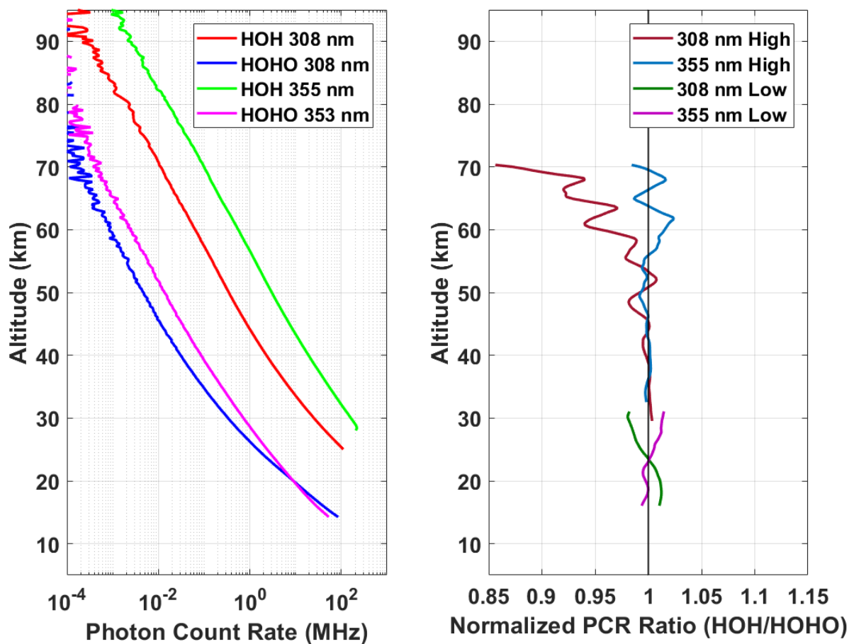
Figure 2. High gain signals for the HOH and HOHO lidars showing higher signal levels in the newly improved HOH lidar. Ratios of high and low gain signals for the HOH and HOHO lidars showing SNR improvement in received signal.
