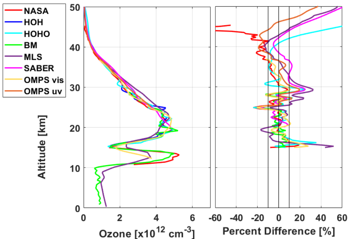
Figure 4. Ozone profiles measured by the NASA-STROZ (red), HOH (blue), and HOHO (cyan) lidars, locally launched ozonesonde (green), and overpasses from SABER (magenta), MLS (violet), OMPS VIS (mustard), OMPS UV (burnt orange) on the night of 6 April 2019.
