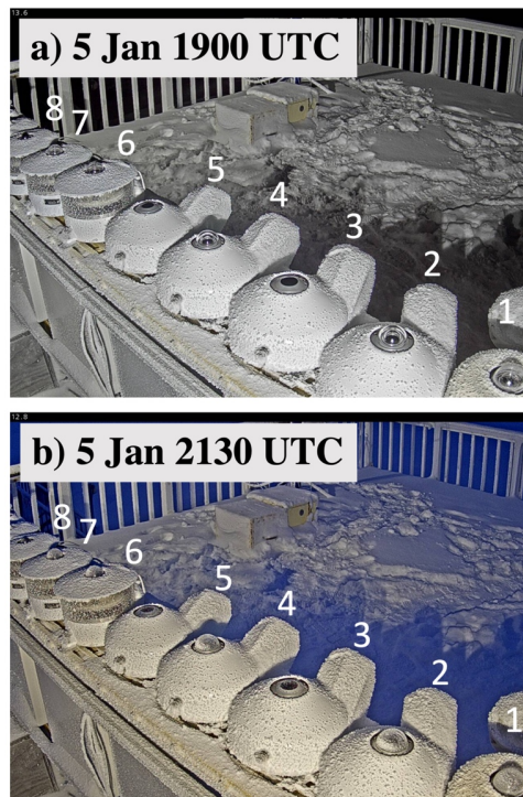
Figure 7. From CAM1, a freezing fog event in progress on 5 Jan and resulting in riming. (a) Ventilators operating normally during the riming event. (b) After the image in (a) was captured, the ventilators were unpowered resulting in icing on domes after several hours of equilibration. Numbers refer to the system positions from Figure 1b.
