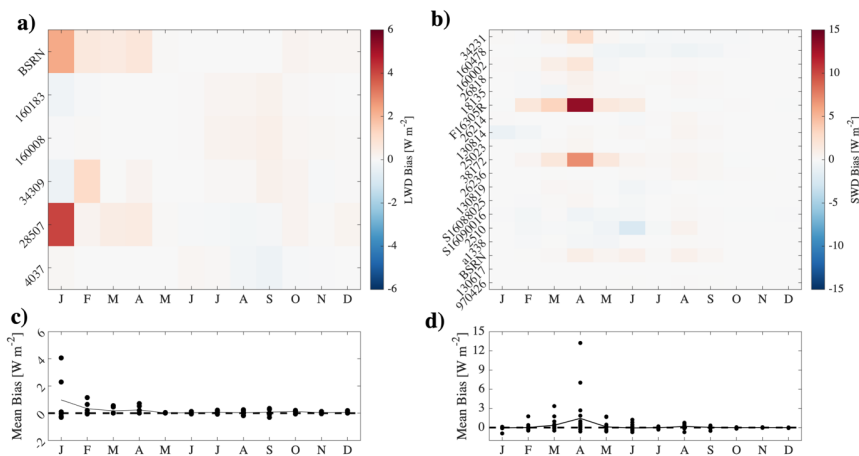
Figure 6. Calculations of biases in monthly means relative to the BE for LWD (a,c) and SWD (b,d). The upper panels show individual instruments and months; the same data are plotted in time series form in the lower panels for reference. All calculations are corrected for statistical differences between individual radiometers and the BE when ice-free. The calculations are for all conditions, not just times when ice was present.
