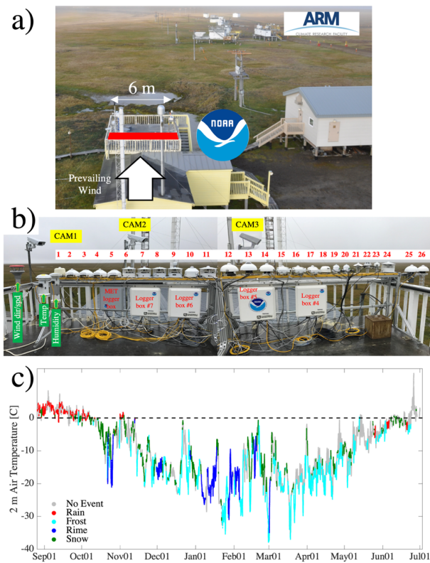
Figure 1. (a) NOAA-GML Barrow Atmospheric Baseline Observatory in Utqiagvik, Alaska ( 71.325^{\circ}\text{N} , 156.625^{\circ}\text{W} , 8 masl), DoE-ARM facility in the background (image from https://www.esrl.noaa.gov/gmd/obop/brw/ ). The red square in (a) shows location and orientation of the D-ICE table, which is pictured in (b). (c) Time series of air temperature color-coded with the types of precipitation and icing events that were recorded: rain (red), frost (cyan), rime (blue), snow (green), and grey (no event).
