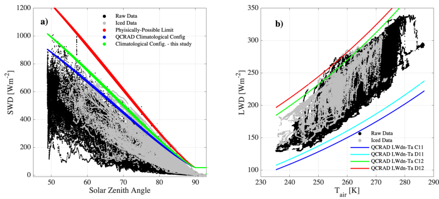
Figure 2. Examples of climatological configurable limit tests from Long and Shi (2008) for SWD (SN F16305R) (a) and LWD (SN 28507) (b). The figures are comparable to figures 1 and 9 from Long and Shi except that 1 min average are shown here instead of 15 min. Black points are ice-free and gray points are contaminated with ice. The colored lines are suggested thresholds for rejection of data of varying degrees of strictness.
