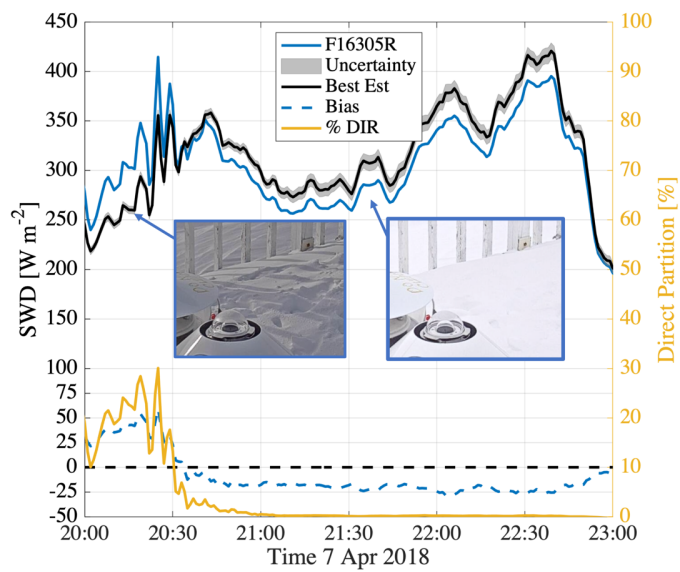
Figure 5. Case study of SWD on 7 April 2018. The solid black line and grey shading are the best estimate and uncertainty, the solid blue line is an icy pyranometer shown in the inset images. The dashed blue line is the bias in the solid blue relative to the solid black and the yellow line shows the percent of the irradiance contributed by the direct beam: when this value is near zero, the lighting is diffuse under overcast conditions.
