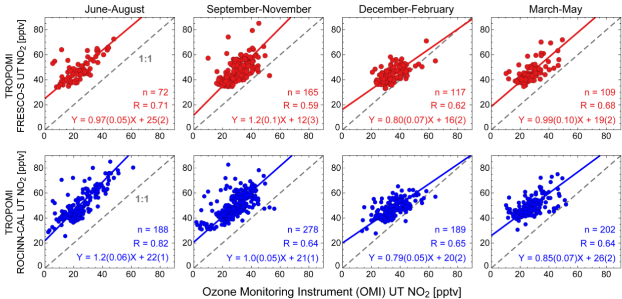
570 Figure 8: Comparison of TROPOMI and OMI cloud-sliced UT NO 2 . Points are seasonal means in June 2019 to May 2020 for TROPOMI and January 2005 to December 2007 for OMI gridded to the same 5° × 8° (latitude × longitude) grid for FRESCO-S vs OMI (upper panel, red) and ROCINN-CAL vs OMI (lower panel, blue). Values give the number of points, Pearson’s correlation coefficients (R), RMA regression coefficients, and, in parentheses, bootstrap resampling slope and intercept errors.
