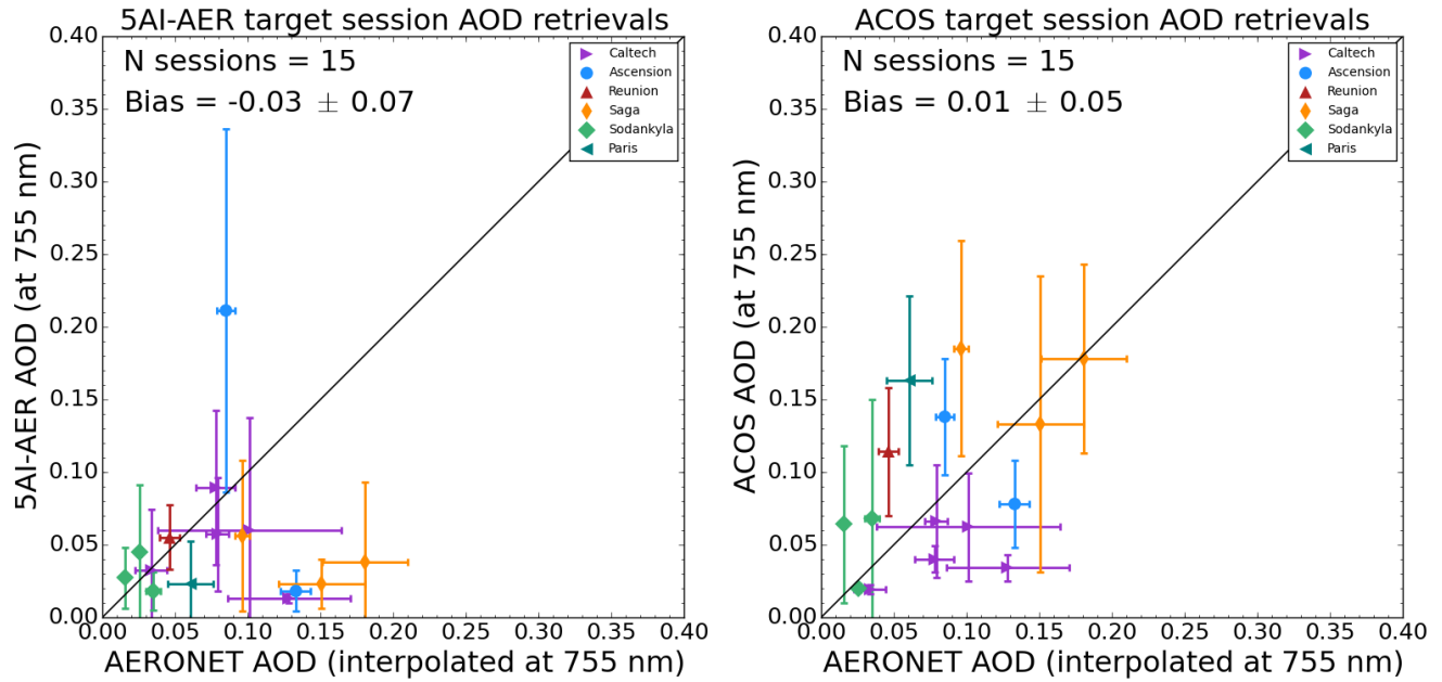
Figure 10. 5AI-AER (left) and ACOS B8r (right) OCO-2 target total AOD retrieval results compared to AERONET AOD 430 interpolated at 755 nm. Individual sounding results are averaged for every target session: markers show session average for OCO- 2 and AERONET AOD, and error bars show standard deviations.
