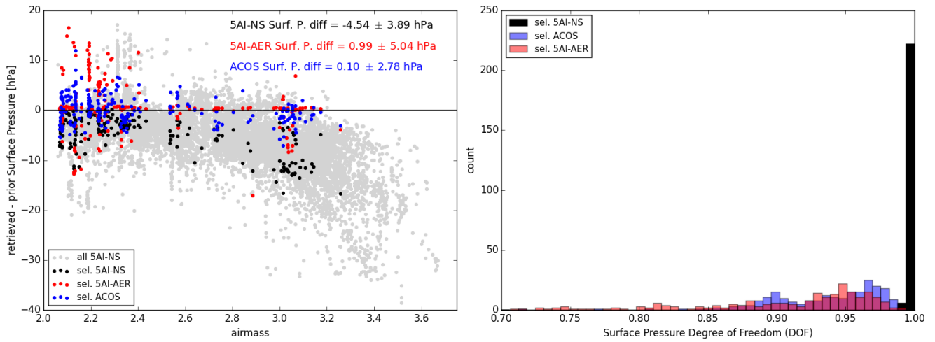
Figure 8. Retrieved surface pressure airmass dependence (left) for all 5AI-NS target OCO-2 soundings (light grey), 5AI-NS soundings selected in the small sub-sample that passed all filters (black), corresponding 5AI-AER (red) and ACOS (blue). Distributions of surface pressure degrees of freedom (right) for 5AI-NS (black), 5AI-AER (red) and ACOS (blue).
