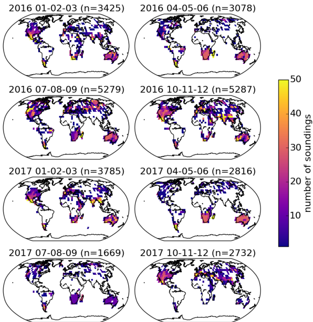
Figure 1. Spatial and temporal repartition of the sample of nadir OCO-2 soundings selected for 5AI retrievals, in seasonal and 5^\circ \times 5^\circ square bins. The titles include the number of soundings n for the corresponding panel: the low number of selected soundings in July-August-September 2017 is due to an identified OCO-2 data gap.
