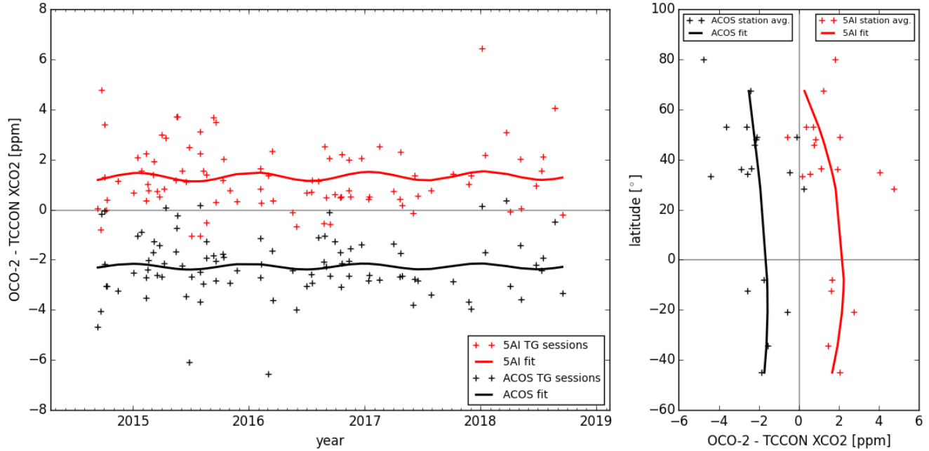
Figure 4. 5AI and raw ACOS B8r OCO-2 target X_{CO_2} bias with regard to TCCON as a function of time (left panel) and latitude (right panel). Crosses show individual session averages in the left panel and individual station averages in the right panel, full lines show polynomial fits of this bias for all target sessions.
