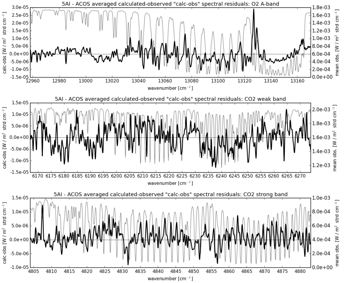
Figure 11. 5AI – ACOS average calculated – observed ‘calc-obs’ spectral residuals in the O 2 A-band (top panel), CO 2 weak band (middle panel) and CO 2 strong band (bottom panel) appear in thick black lines (left axis). A typical spectrum for the three bands is shown in thin grey lines (right axis).
