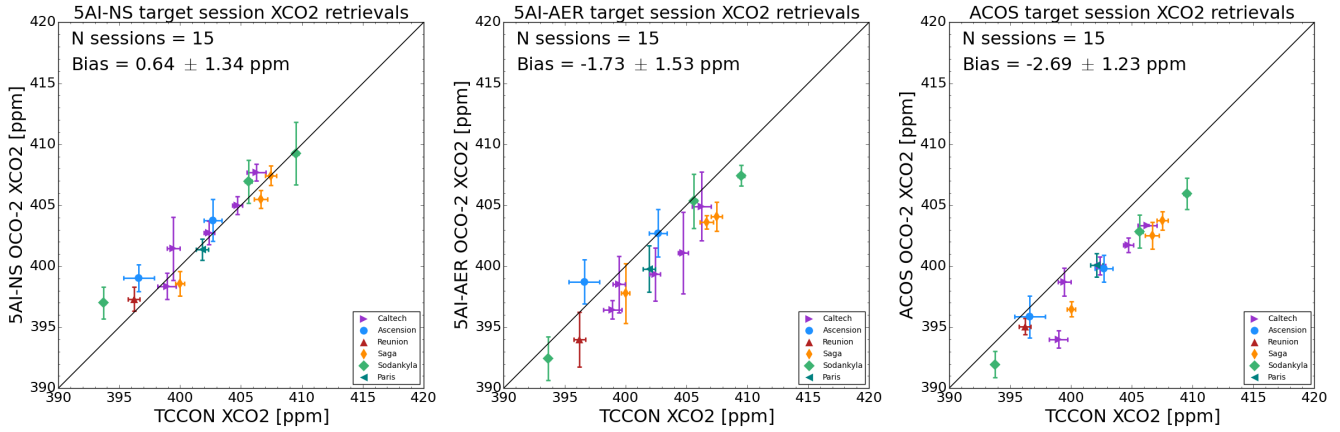
Figure 9. 5AI-NS (left), 5AI-AER (center) and raw ACOS B8r (right) OCO-2 target X_{CO_2} retrieval results compared to TCCON 425 official X_{CO_2} product. Individual sounding results are averaged for every target session: markers show session average for OCO-2 and TCCON X_{CO_2} , and error bars show standard deviations.
