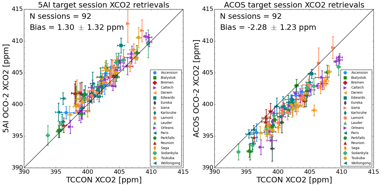
Figure 3. 5AI (left) and raw ACOS B8r (right) OCO-2 target X_{CO_2} retrieval results compared to TCCON official X_{CO_2} product. Individual sounding results are averaged for every target session: markers show session average for OCO-2 and TCCON X_{CO_2} , and error bars show standard deviations.
