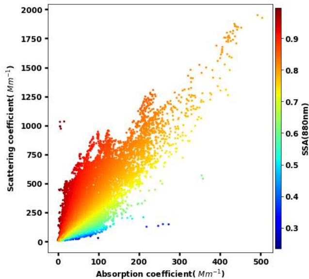
Figure 2. The SSA of field observation (1)-(8).
