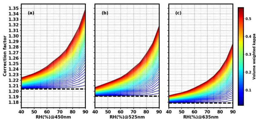
Figure 912. The theoretical calculation of the scattering correction factors (CF) versus relative humidity (RH) and hygroscopicity \kappa at the wavelengths of 450 nm (a), 525 nm (b), 635 nm (c). The dashed line represents scattering correction factor in the dry state, and the color represents the overall hygroscopicity of aerosols ( \kappa ). The color bar is derived from multiplying the total volume-weighted \kappa of 0.281 by 0.05 to 2, with 0.01 as the interval.
