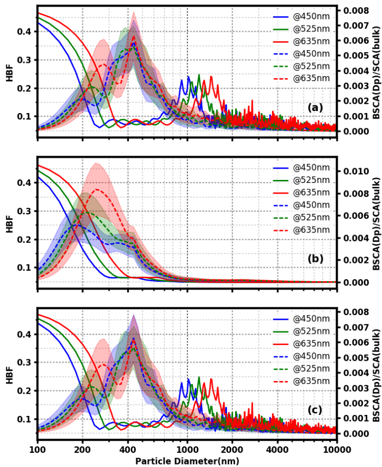
Figure 54. The HBF change of scattering particles (a), absorption-absorbing particles (b), and core-shell mixing particles of core radius 35 nm (c) with the change in particle diameter (solid line). The dashed lines represent the ratio of hemispheric backscattering at a certain diameter relative to the total scattering.
