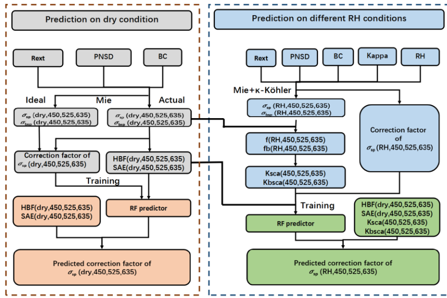
270 Figure 87. Flow chart of estimating CF under different relative humidity conditions by machine learning.
