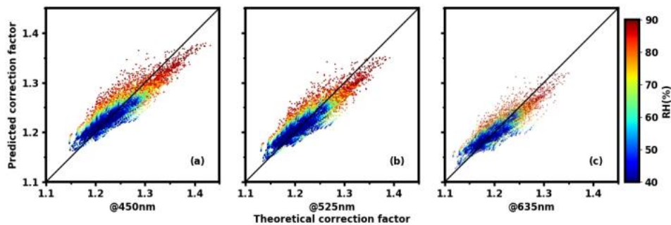
295 Figure 10. The comparison of theoretical correction factor and predicted correction factor calculated by the Ångström index at different wavelengths; the figure (a), (b), (c) are the comparison results for 450 nm, 525 nm and 635 nm, respectively. The black solid line represents that theoretical correction factor equals to the predicted one. The color of data points represents different relative humidity conditions.
