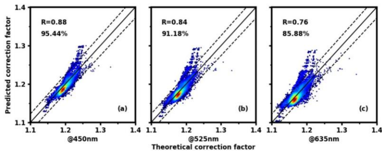
Figure 8.11. On dry conditions, the comparison of the correction factors calculated by our method and theoretical Mie-calculation values at the wavelengths of 450 nm (a), 525 nm (b), and 635 nm (c), respectively, with a black solid 1:1 line and two dashed lines representing a deviation of 2 %. The color of the data point represents data density; the warmer the hue, the denser the data point. R is the correlation coefficient, and the percentage indicates the percentile of points falling within the error range of 2 %.
