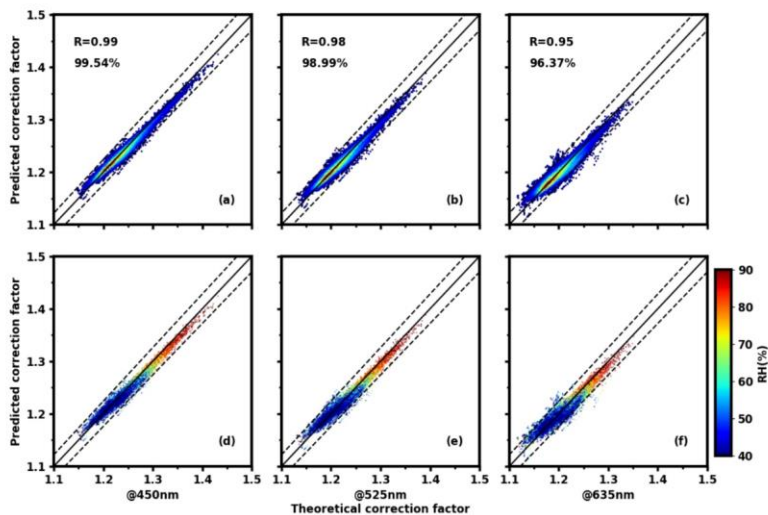
Figure 4013. On different relative humidity conditions, the comparison of the correction factors calculated by our method and theoretical Mie-calculation values at the wavelengths of 450 nm (a), 525 nm (b), and 635 nm (c), respectively, with a black solid 1:1 line and two dashed lines representing a deviation of 2 %. The color of the data point represents data density; the warmer the hue, the denser the data point. R is the correlation coefficient, and the percentage indicates the percentile of points falling within the error range of 2 %. The data in (d), (e), (f) are the same as those in (a), (b), (c), but the color here stands for different relative humidity conditions rather than density.
