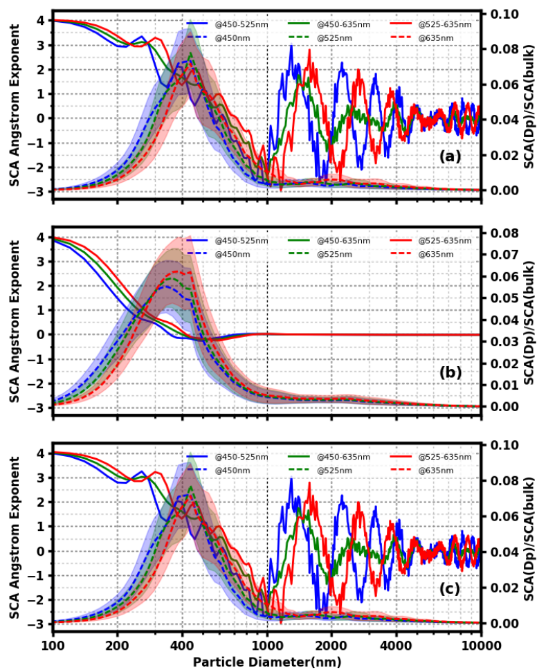
Figure 43. The SAE change of scattering particles (a), absorption absorbing particles (b), and core-shell mixing particles of core radius 35 nm (c) with the change in particle diameter (solid line). The dashed lines represent the ratio of scattering at a certain diameter relative to the total scattering.
