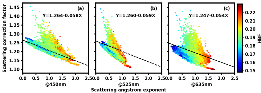
Figure 23. Scattering correction factors versus the scattering Ångström index. (a), (b), (c) respectively represent the results at the wavelengths of 450 nm, 525 nm, and 635 nm. The black dashed line is a statistical linear relationship, and the color of points represents the hemispheric backscattering fraction HBF.
