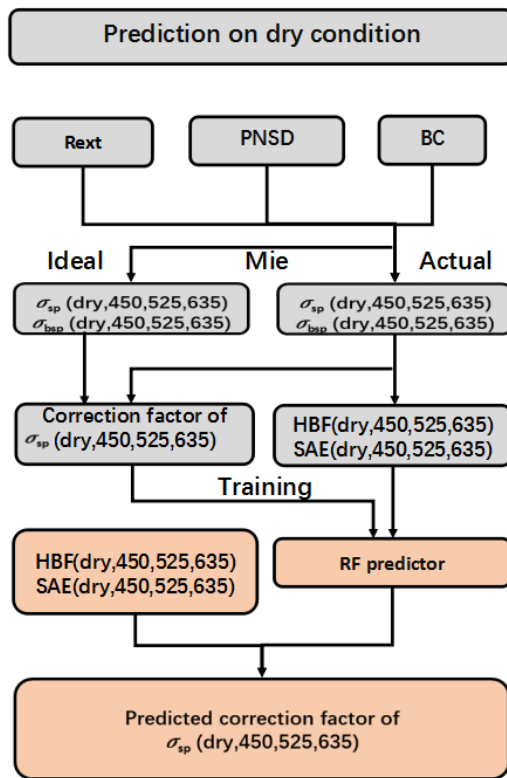
Figure 65. Flow chart of estimating CF under dry conditions by machine learning.
