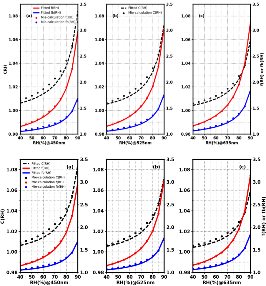
Figure 76. The comparison between \kappa fitted and theoretical Mie-calculation f(RH) , f_b(RH) and C(RH) at the wavelengths of 450 nm (a), 525 nm (b), and 635 nm (c) under the condition of nephelometer light source. The scatter points represent each theoretical Mie-calculation value. The red solid line is the f(RH) fitted curve and the blue solid line is the f_b(RH) fitted curve, both corresponding to the right ordinate value. The black dashed line is the C(RH) fitted curve, which corresponds to the left ordinate value.
