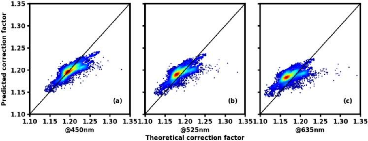
255 Figure 9. The comparison of theoretical correction factor and predicted correction factor calculated by the Ångström index at different wavelengths; figure (a), (b), (c) are the comparison results for 450 nm, 525 nm and 635 nm, respectively. The black solid line represents that theoretical correction factor equals to the predicted one. The color of data points represents the data density; the warmer the hue, the denser the data points.
